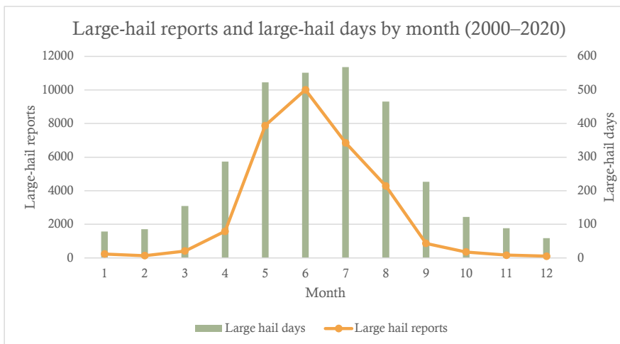
240 241 Figure 3. Combined line graph and bar chart of the total monthly numbers of large-hail reports (orange 242 line) and large-hail days (green bars) across Europe: 2000–2020. These quantities are not divided by the 243 number of years because of the incomplete data for the year 2020.
