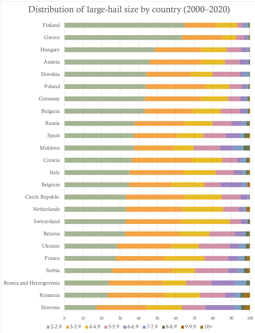
492 Figure 14. Horizontal bar charts of the size distribution of large hail for countries with 100 or more 493 reports (%): 2000–2020.
