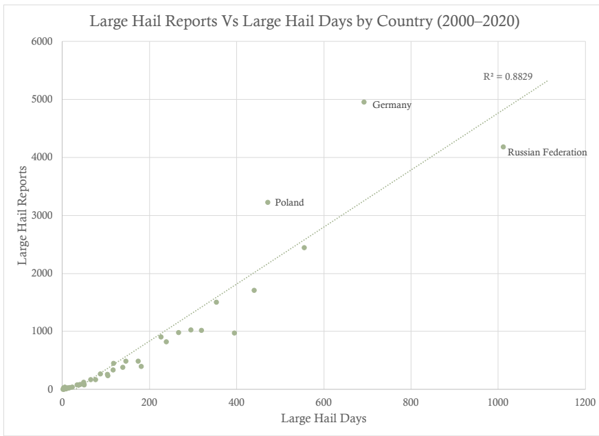
460 461 Figure 13. Scatterplot of the total number of large-hail reports versus large-hail days by country: 2000– 462 2020.
