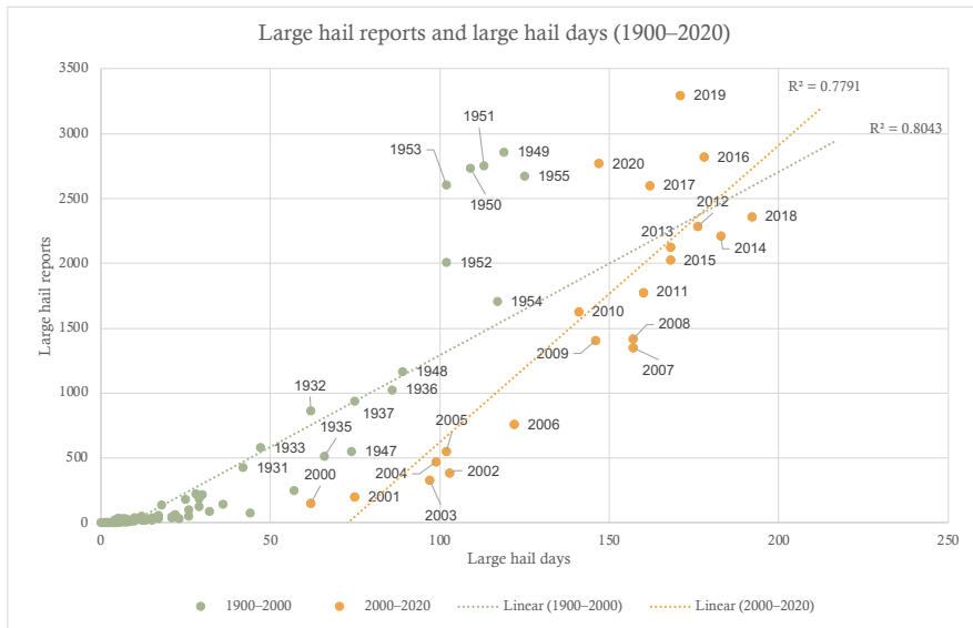
216 217 Figure 2. Scatterplot of the annual number of large-hail days versus annual number of large-hail reports 218 across Europe: 1900–2000 (green dots) and 2000–2020 (orange dots), with corresponding linear regression 219 lines. These quantities are not divided by the number of years because of the incomplete data for the year 220 2020.
