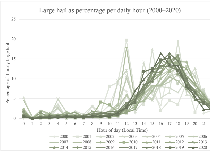
313 314 Figure 6. Hourly percentage of large hail in local time across Europe in local time for each year 2000 to 315 2020.
