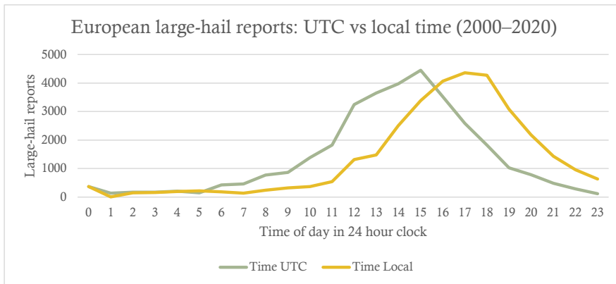
296 297 Figure 5. Distribution of the hourly time of large-hail reports across Europe in UTC (green line) and local 298 time (orange line): 2000–2020. Reports are associated with the starting hour (i.e., a report at 1515 UTC 299 would be placed in the 1500-UTC bin).
