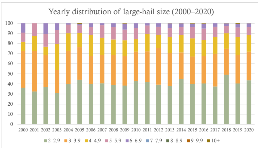
317 Figure 8. Time series of bar charts of the annual distributions of large-hail size across Europe in 1-cm 318 diameter bins: 2000–2020.
