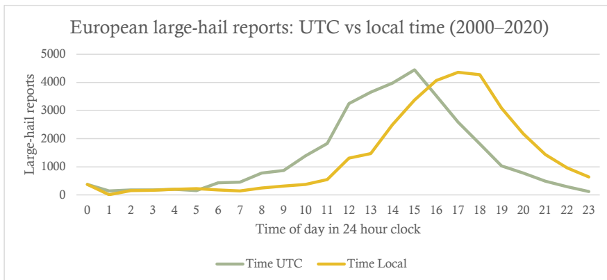
258 259 Figure 5. Distribution of the hourly time of large-hail reports across Europe in UTC (green line) and local 260 time (orange line): 2000–2020. Reports are associated with the starting hour (i.e., a report at 1515 UTC 261 would be placed in the 1500-UTC bin).
