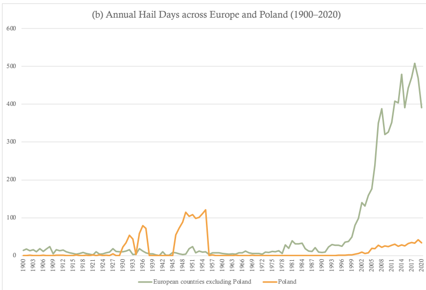
513 Figure 14. Time series of annual numbers of (a) large-hail reports for Europe (green line) and Poland (red 514 line), and (b) large-hail days for Europe (green line) and Poland (red line): 1900–2020.
