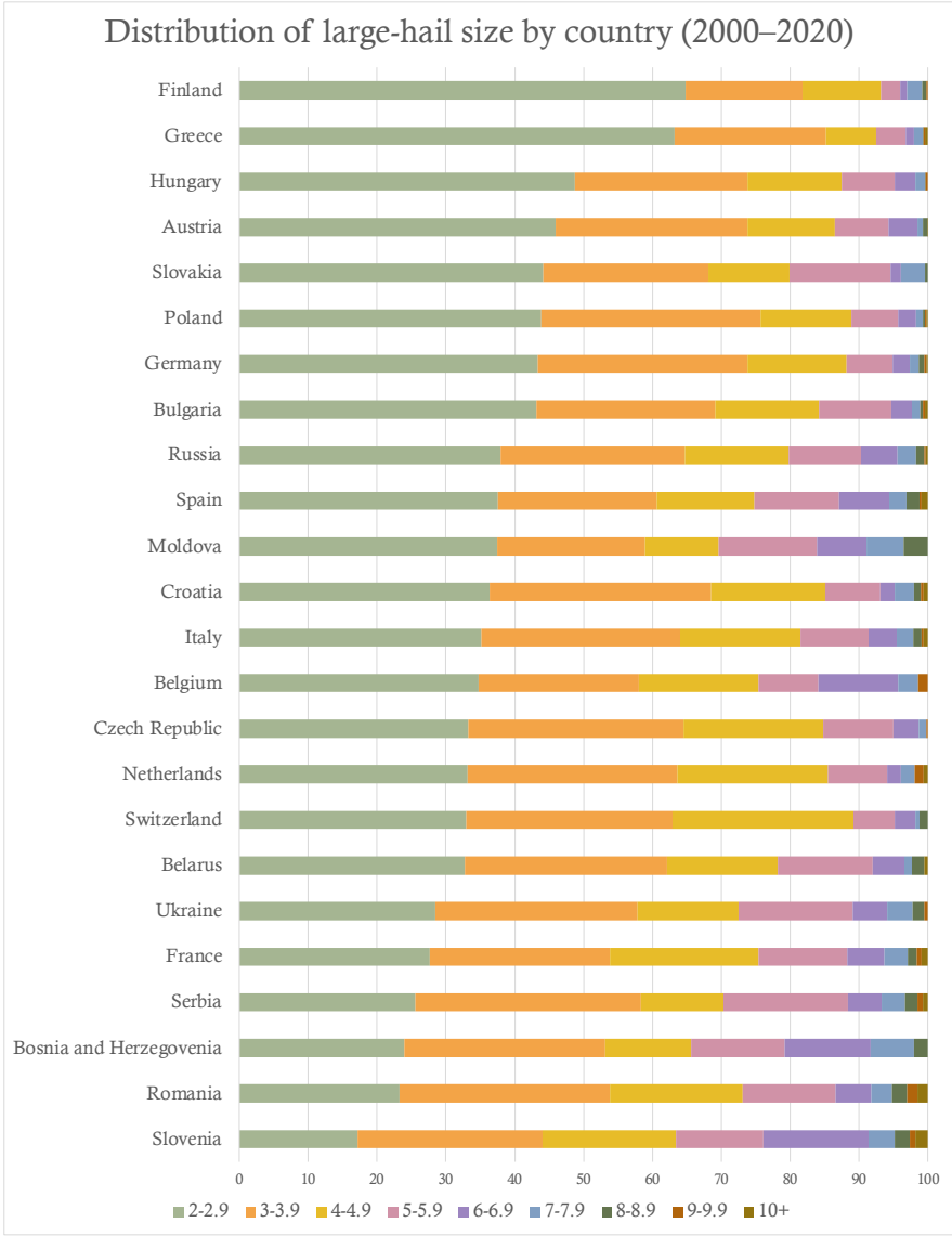
425 Figure 13. Horizontal bar charts of the size distribution of large hail for countries with 100 or more 426 reports: 2000–2020.
