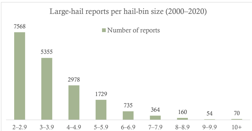
298 Figure 7. Bar chart of the number of large-hail reports across Europe by maximum diameter in 1-cm bins: 299 2000–2020.
