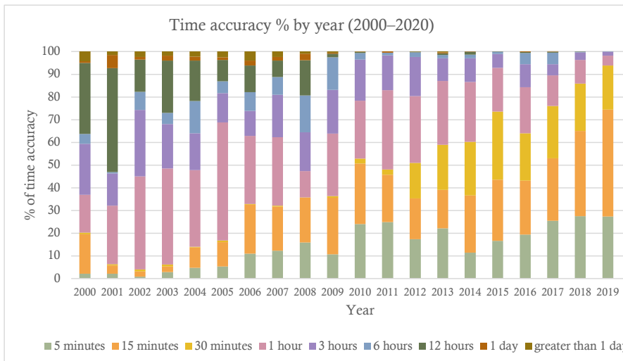
352 Figure 10. Time series of bar charts of the annual distributions of time accuracy of reports across Europe: 353 2000–2020.
