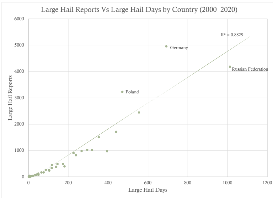
395 396 Figure 12. Scatterplot of the total number of large-hail reports versus large-hail days by country: 2000– 397 2020.
