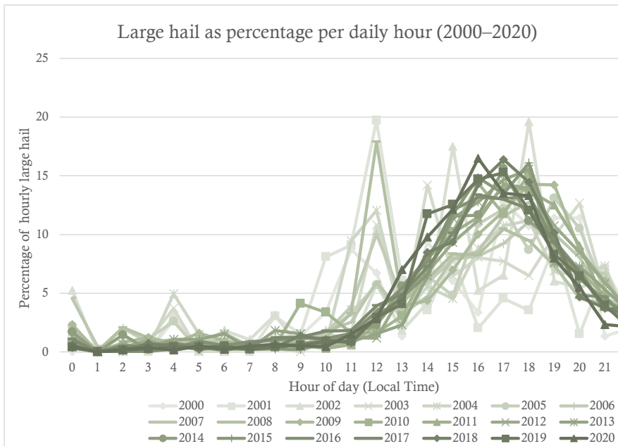
276 Figure 6. Hourly percentage of large hail in local time across Europe in local time for each year 2000 to 277 2020.
