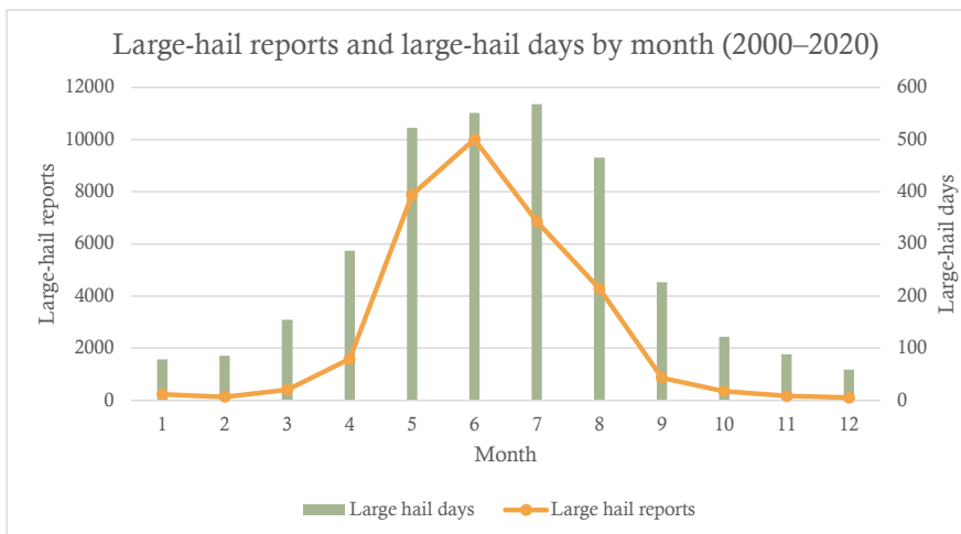
213 214 Figure 3. Combined line graph and bar chart of the total monthly numbers of large-hail reports (orange 215 line) and large-hail days (green bars) across Europe: 2000–2020. These quantities are not divided by the 216 number of years because of the incomplete data for the year 2020.
