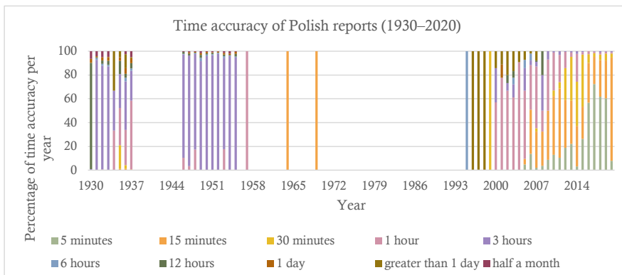
540 541 Figure 15. Time series of bar charts the annual distributions of time accuracy of reports for Poland: 1930– 542 2020.
