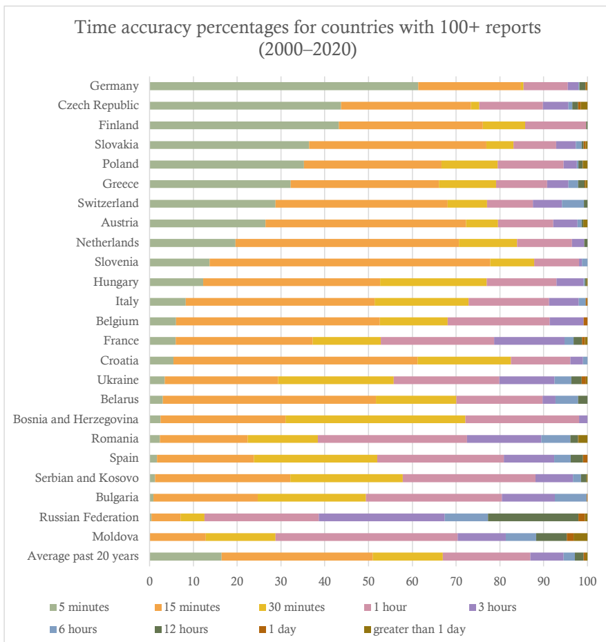
362 363 Figure 11. Horizontal bar charts of the time accuracy for countries with 100 or more reports: 2000–2020.
