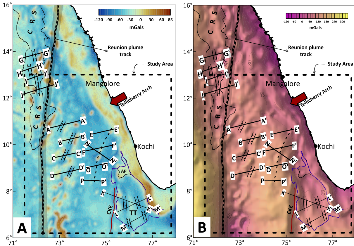
Figure 2. A) Satellite-derived free-air gravity anomaly map B) Crustal Bouguer anomaly map. The location and orientation of identified extensional features, grabens and intrusives are marked. Black solid lines represent the location of the profiles. Interpreted seismic sections are shown in fig. 5. The thick broken reddish line in the centre of the basin represents the identified volcanic ridge. (refer to fig. 5 & S1 for seismic sections). The location of the maps is shown in fig. 1A. CRS represents the Cannanore Rift System as identified by DGH2024. CKE: Chain-Kairali Escarpment; AP: Alleppey Platform; TT: Trivandrum Terrace.
