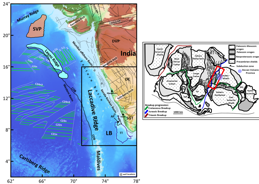
Figure 1. Regional tectonic map of the western continental margin of India (Smith and Sandwell, 1997) on the left . Solid green coloured lines represent the mapped seafloor spreading type magnetic lineations (Bhattacharya and Yatheesh, 2015, and references therein) . Solid white lines represent the mapped fracture zones or pseudo-faults. Black solid lines in the offshore region represent shear zones and faults. The larger study area is marked in a black rectangle. MR- Murray Ridge- The map on the right shows the position of India relative to Madagascar and Deccan Volcanic Province in late Paleozoic fit (Lovecchio et al., 2020, modified after). The area of interest is marked in red rectangle. SVP: Saurashtra volcanic province; DVP: Deccan Volcanic Province; DC: Dharwar Craton; SGT: Southern Granulite Terrain; LB: Laccadive Basin; AP: Alleppey Platform; TT Trivandrum Terrace.
