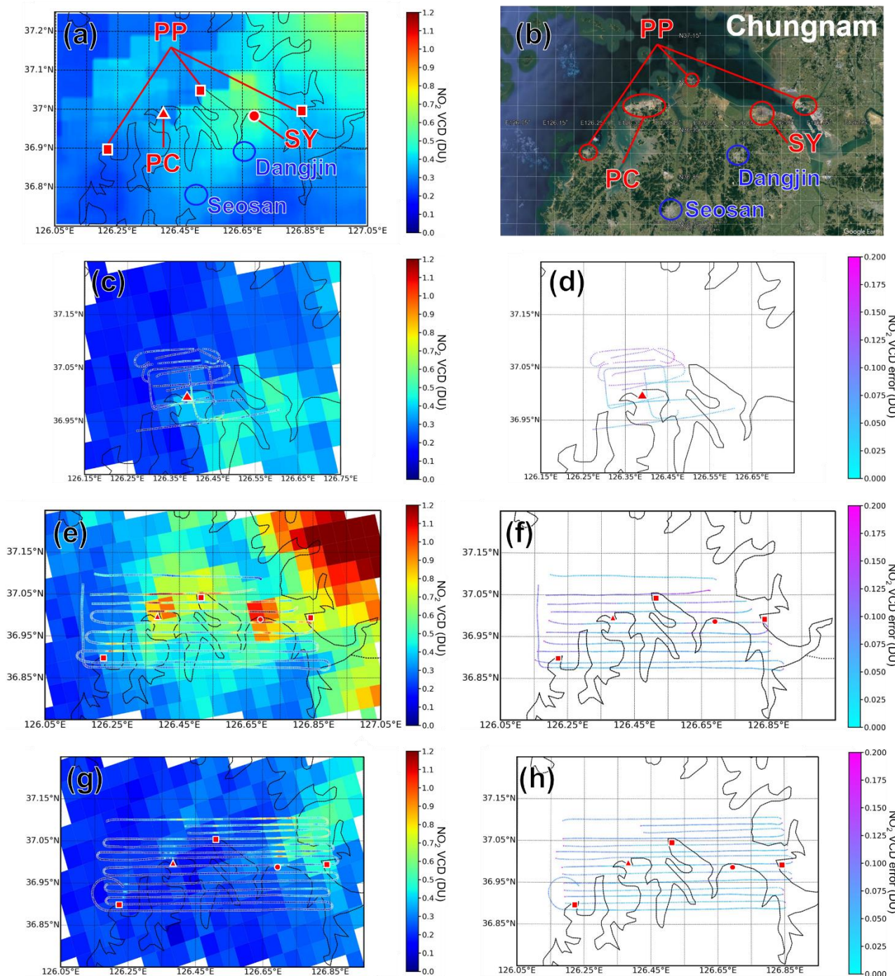
Figure 5. (a) Downscaled average TROPOMI \text{NO}_2 VCD in October and November from 2019 to 2022 and (b) Google Earth image (© Google Earth) of the Chungnam domain with major industrial point sources of \text{NO}_2 and populated urban areas denoted in red and blue circles, respectively. (c), (e), and (g) show \text{NO}_2 VCD retrieval results from HIS overlaid on TROPOMI swath data and (d), (f), and (h) show the uncertainty of HIS-retrieved \text{NO}_2 VCD. (c) and (d), (e) and (f), and (g) and (h) show observed results from the research flight on 17 October 2020, 24 November 2022, and 25 November 2022, respectively.
