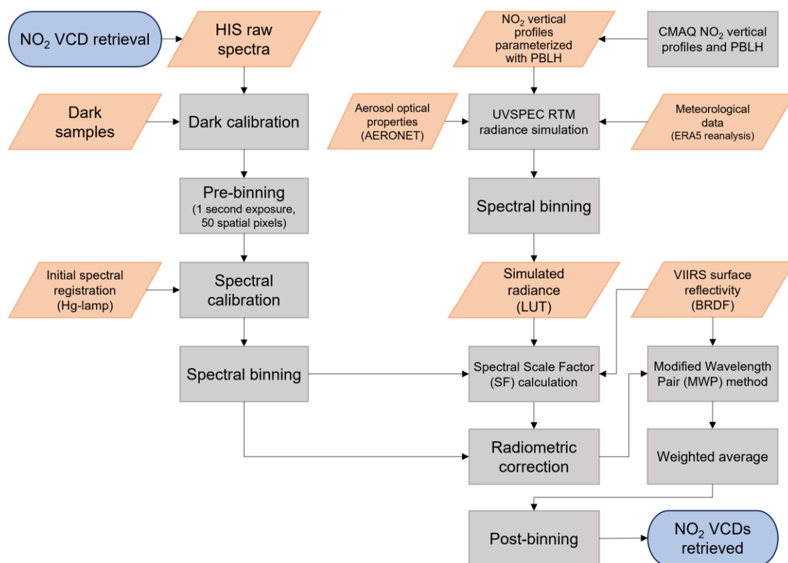
135 Figure 1. Flowchart of the NO 2 VCD retrieval from the airborne HIS spectra using the MWP method.
