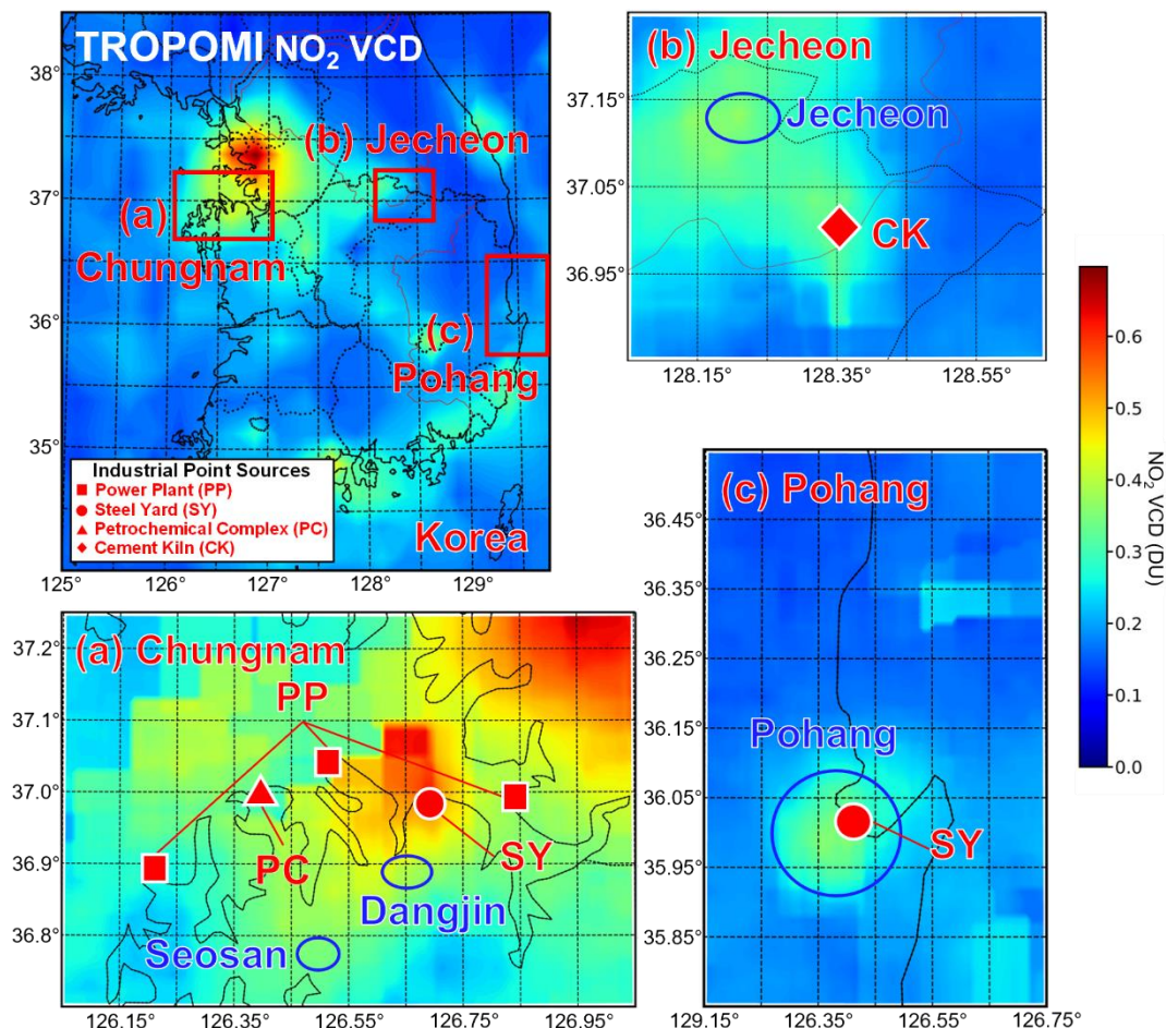
465 Figure 4. Location of major industrial point sources in Korea targeted for airborne HIS observations overlaid by average TROPOMI \text{NO}_2 \text{VCD}_{\text{Total}} in October and November from 2019 to 2022. Corresponding TROPOMI swath datasets were downsampled to 0.25^\circ \times 0.25^\circ and 0.01^\circ \times 0.01^\circ resolutions for Korea and each respective target domain (i.e., Chungnam, Jecheon, and Pohang, respectively).
