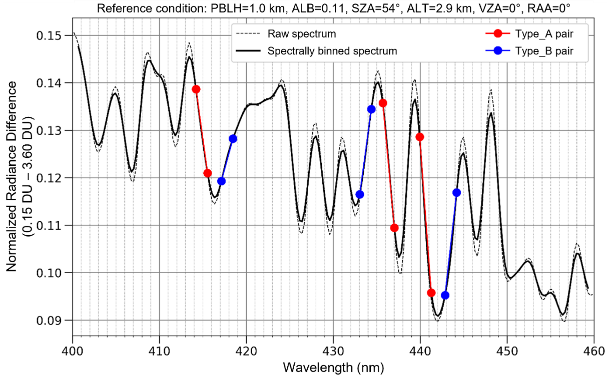
165 Figure 2. Example of spectral radiance sensitivity to NO 2 VCD under reference HIS observation condition at Pohang area shown with three different wavelength-pairs per each wavelength pair type (Type_A in red and Type_B in blue) used in the MWP method.
