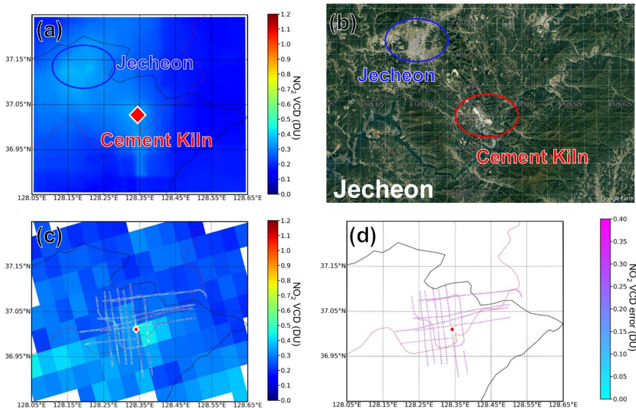
535 Figure 6. (a) Downscaled average TROPOMI \text{NO}_2 VCD in October and November from 2019 to 2022 and (b) Google Earth image (© Google Earth) of the Jecheon domain with major industrial point source of \text{NO}_2 and populated urban area denoted in red and blue circles, respectively. (c) and (d) show observed results from the research flight on 3 November 2020, while (c) shows \text{NO}_2 VCD retrieval results from HIS overlaid on TROPOMI swath data, and (d) shows the uncertainty of HIS-retrieved \text{NO}_2 VCD.
