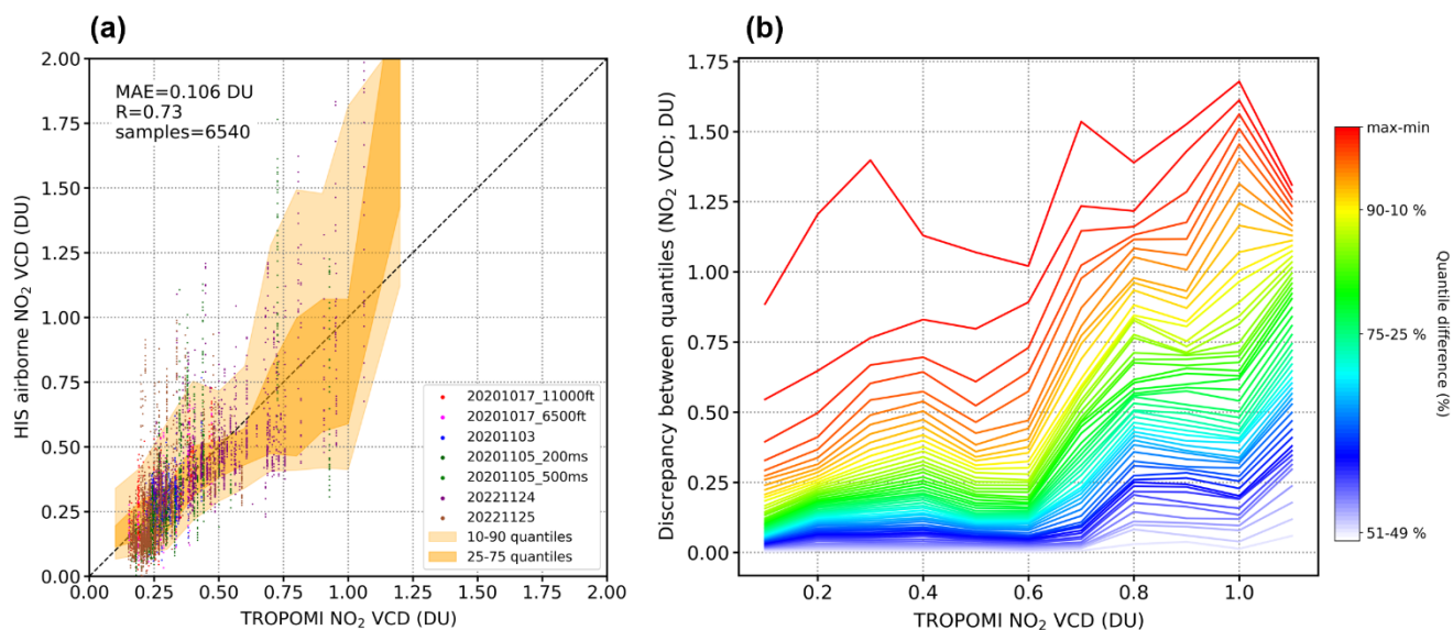
600 Figure 8. (a) Comparison of bias-corrected HIS and TROPOMI NO 2 VCDs with the corresponding HIS NO 2 VCD quantiles (10, 25, 75, 90-th) shown over the TROPOMI NO 2 VCD range. (b) Differences between HIS NO 2 VCDs quantile values (from maximum-minimum to 51%-49%) at corresponding TROPOMI NO 2 VCD range.
