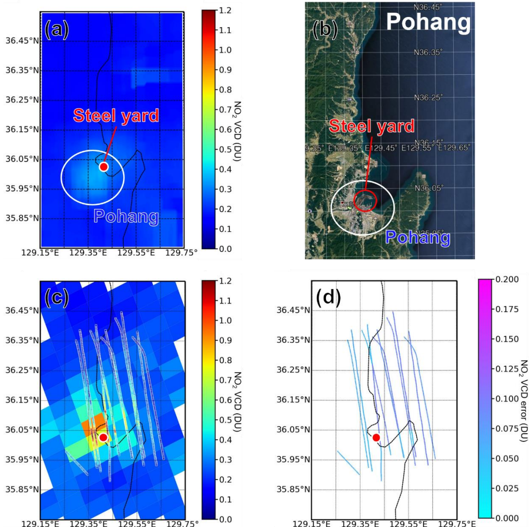
555 Figure 7. (a) Downscaled average TROPOMI NO 2 VCD in October and November from 2019 to 2022 and (b) Google Earth image (© Google Earth) of the Pohang domain with an industrial point source of NO 2 and populated urban area denoted in red and white circles, respectively. (c) and (d) show observed results from the research flight on 5 November 2020, while (c) shows NO 2 VCD retrieval results from HIS overlaid on TROPOMI swath data, and (d) shows the uncertainty of HIS-retrieved NO 2 VCD.
