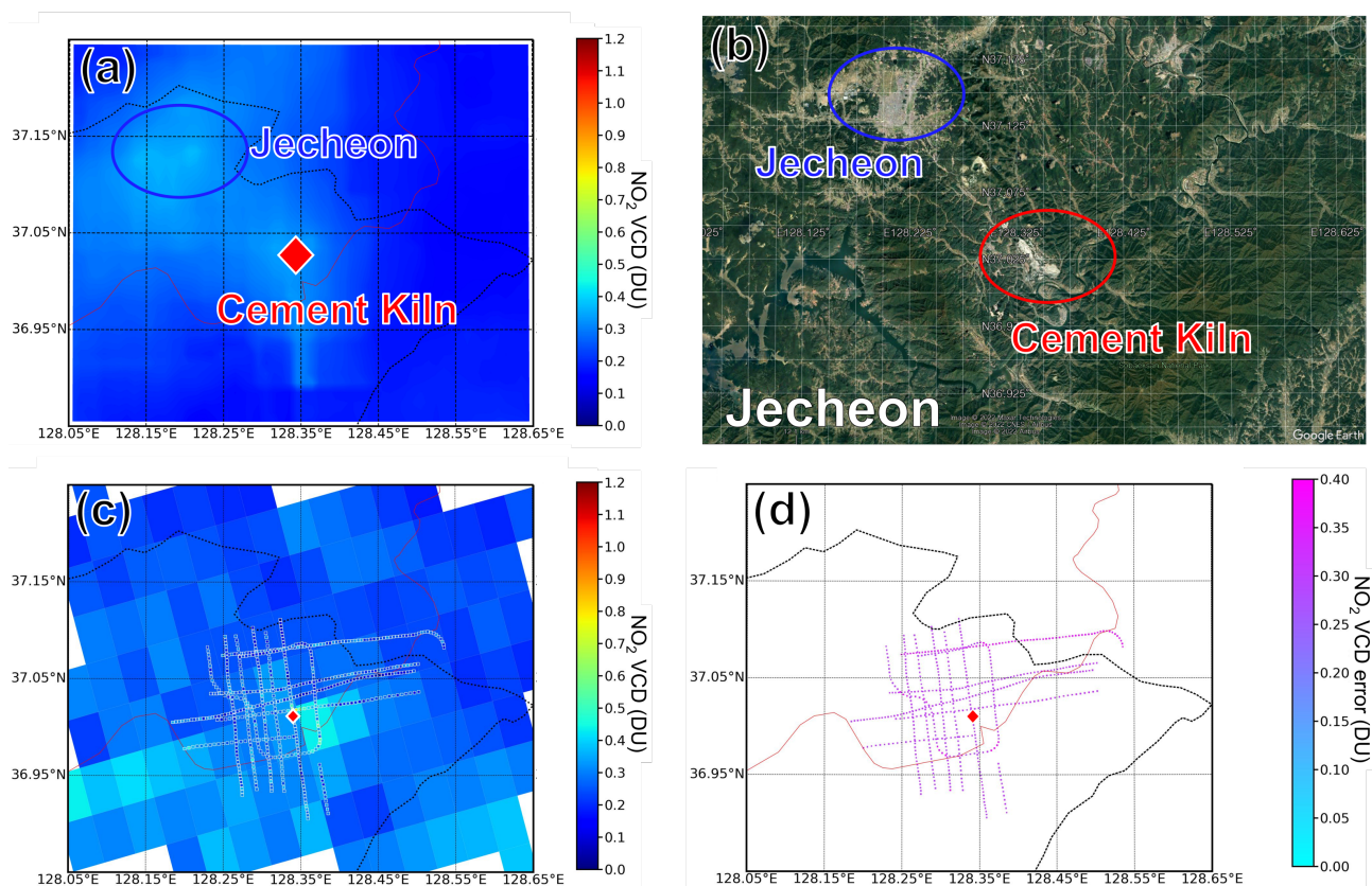
555 Figure 6. (a) Downscaled average TROPOMI NO 2 VCD in October and November from 2019 to 2022 and (b) Google Earth image (© Google Earth) of the Jecheon domain with major industrial point source of NO 2 and populated urban area denoted in red and blue circles, respectively. (c) and (d) show observed results from the research flight on 3 November 2020, while (c) shows NO 2 VCD retrieval results from HIS overlaid on TROPOMI swath data, and (d) shows the uncertainty of HIS-retrieved NO 2 VCD.
