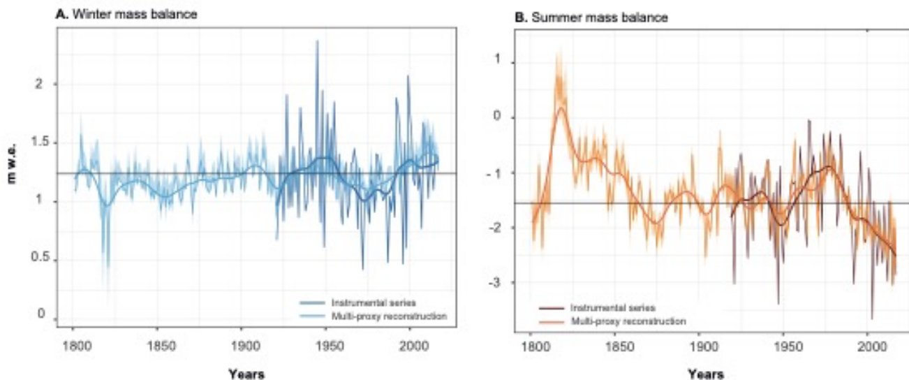
360 Figure 4. Winter (A) and summer (B) mass balance of Silvretta glacier reconstructed from tree-ring proxies over the 1802-2017 period. The thin light blue and orange curves illustrate interannual variations in winter and summer mass balance, respectively, derived from \delta^{18}\text{O} and D_{\text{rad}} (winter) and TRW, \text{CWT}_{\text{rad}} and D_{\text{rad}} (summer). The dark blue and dark brown curves represent the winter and summer mass balance records of Silvretta glacier from 1919- 2017. Thick lines indicate decadal variations, smoothed with an 11-year spline.
