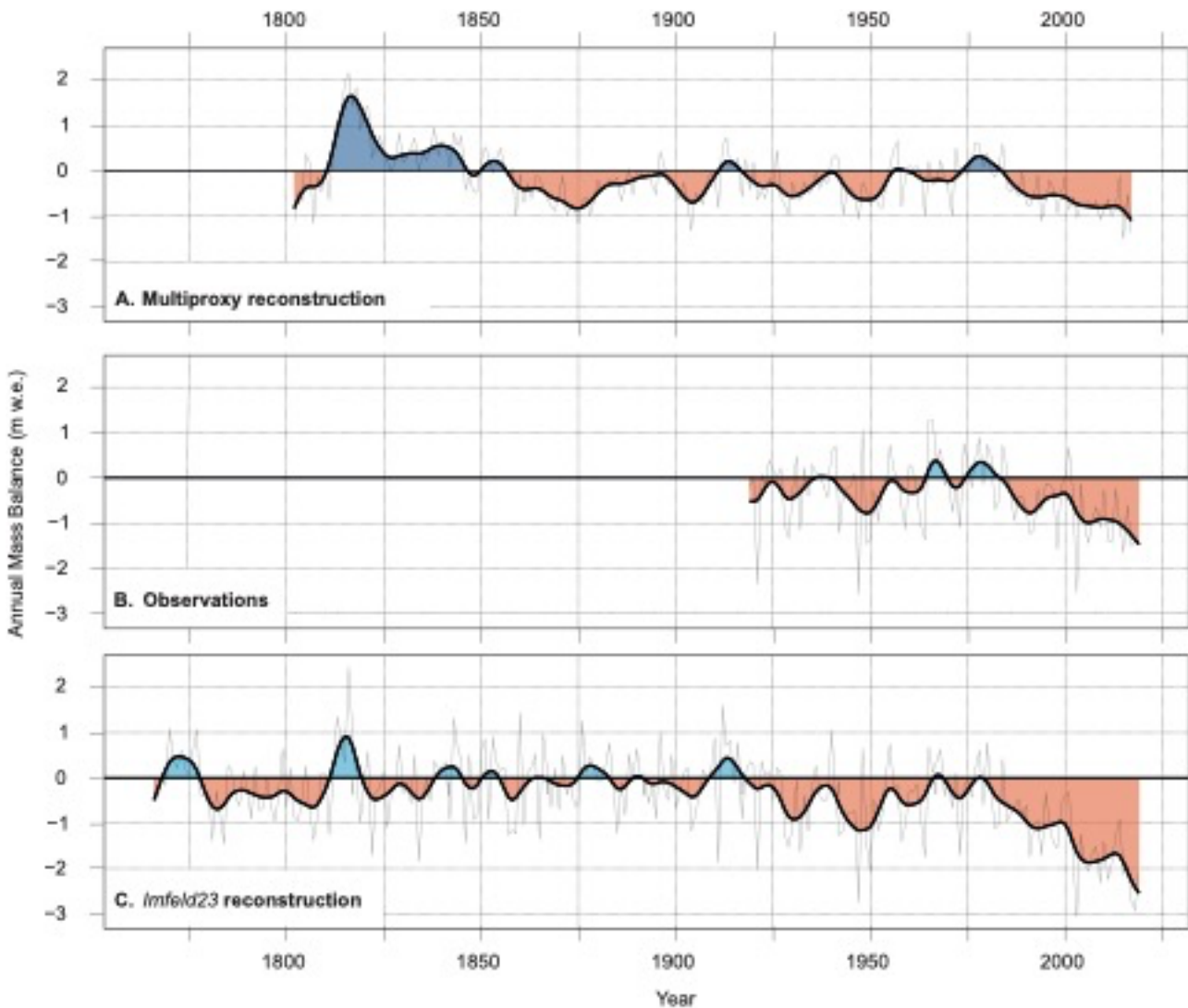
Figure 6. Comparison between annual (thin grey lines) and 11-yr spline smoothed (thick lines) variations of (A) the multiple wood-proxy annual mass balance (Ba) reconstruction, (B) observed Ba and (C) Ba reconstructed from gridded temperature and temperature fields (Imfeld et al., 2023). Periods with positive mass balance are shown in blue, periods with negative mass balance are given in red.
