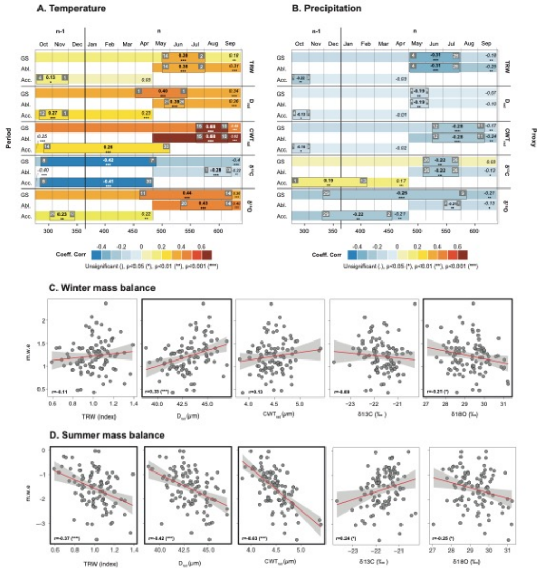
275 Figure 3. Correlations between the TRW, D_{rad} , CWT_{rad} , \delta^{13}C and \delta^{18}O chronologies from God da Tamangur, gridded temperature (A) and precipitation (B) fields from Imfeld23, as well as winter (C) and summer (D) mass balance series from the Silvretta glacier. In panels A, B, correlation coefficients and their associated p-values are presented in italics for the growing (GS, Oct 1 (n-1)-Sep 30(n)), ablation (Abl, May 1 (n)-Sep 30(n)), and accumulation (Acc, Oct 1 (n-1)-Apr 30 (n)) seasons. Time periods with the highest coefficients (highlighted in bold) are delineated by black rectangles. The beginning 280 and end of these optimal periods are denoted by white numbers on a grey background.
