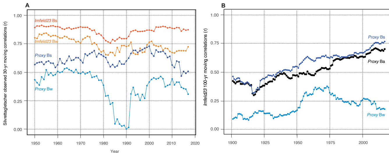
360 Figure 5. (A) 30-yr moving correlations ( r ) of summer ( B_s ) and winter ( B_w ) mass balances estimated from gridded temperature and precipitation fields (Imfeld et al., 2023) and multiple wood-proxy B_s and B_w mass balance reconstruction (this study) with the Silrettagletscher B_w and B_s records (Huss et al., 2015). (B) 100-yr moving correlations of proxy B_s , B_w and annual ( B_a ) mass balance reconstruction with Imfeld23 (Imfeld et al., 2023).
