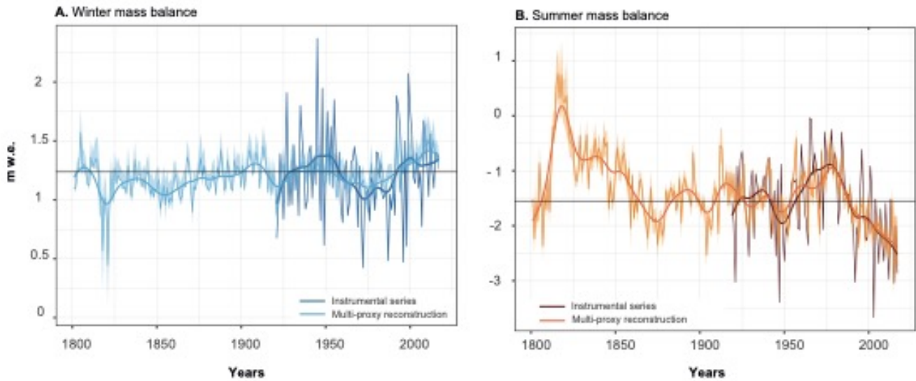
335 Figure 4. Winter (A) and summer (B) mass balance of Silvretta glacier reconstructed from tree-ring proxies over the 1802-2017 period. The thin light blue and orange curves illustrate interannual variations in winter and summer mass balance, respectively, derived from \delta^{18}\text{O} and D_{rad} (winter) and TRW, CWT_{rad} and D_{rad} (summer). The dark blue and dark brown curves represent the winter and summer mass balance records of Silvretta glacier from 1919-2017. Thick lines indicate decadal variations, smoothed with an 11-year spline.
