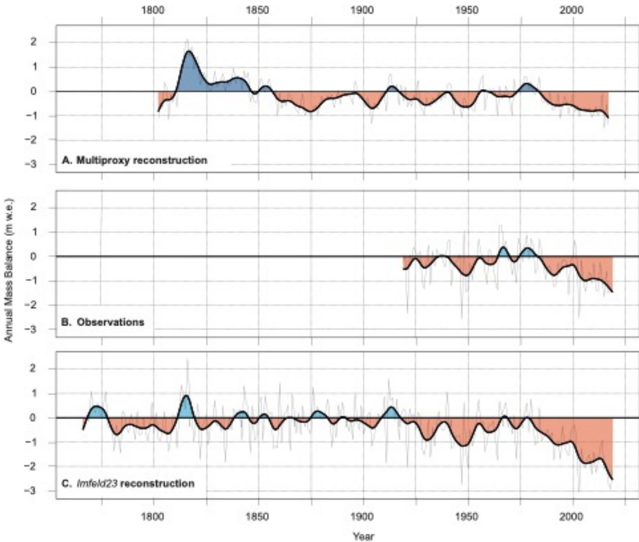
380 Figure 6. Comparison between annual (thin grey lines) and 11-yr spline smoothed (thick lines) variations of (A) the multiple wood-proxy annual mass balance ( B_a ) reconstruction, (B) observed B_a and (C) B_a reconstructed from gridded temperature and temperature fields (Imfeld et al., 2023). Periods with positive mass balance are shown in blue, periods with negative mass balance are given in red.
