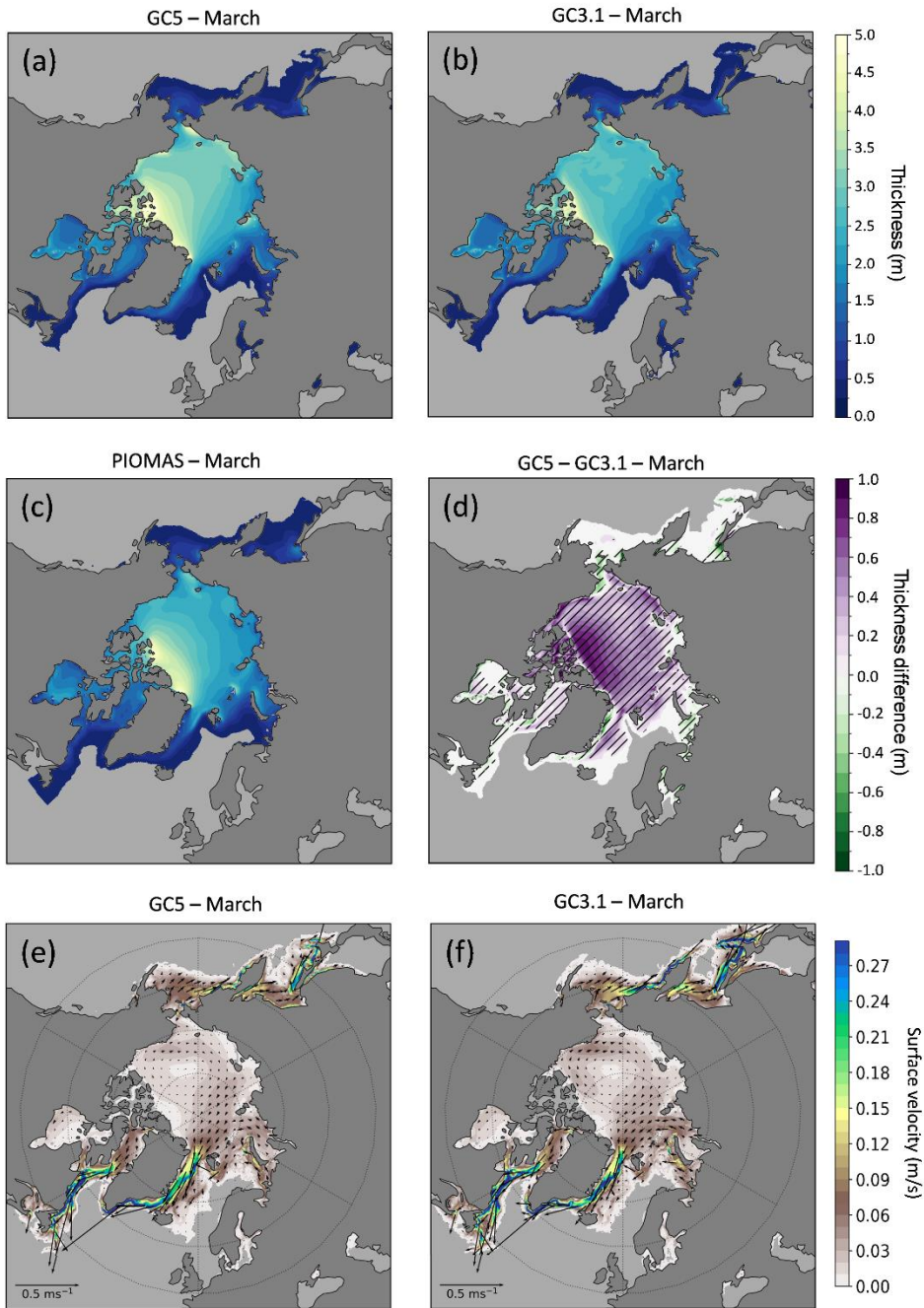
565 Figure 3: March mean sea ice thickness (m) from the last 50 years of 100-year model simulations using year-2000 continuous forcing for (a) GC5 and (b) GC3.1, and (c) from the PIOMAS reanalysis for the period 1990-2009. Panel (d) shows mean sea ice thickness difference between GC5 and GC3.1 (GC5-GC3.1) with hatched areas identifying differences that are significant at the 95% level, calculated using a Welch t-test. Panels (e) and (f) show corresponding 50-year March mean sea ice velocity for GC3.1 and GC5 respectively with coloured shading depicting ice speed and velocity arrows overlain in black.
