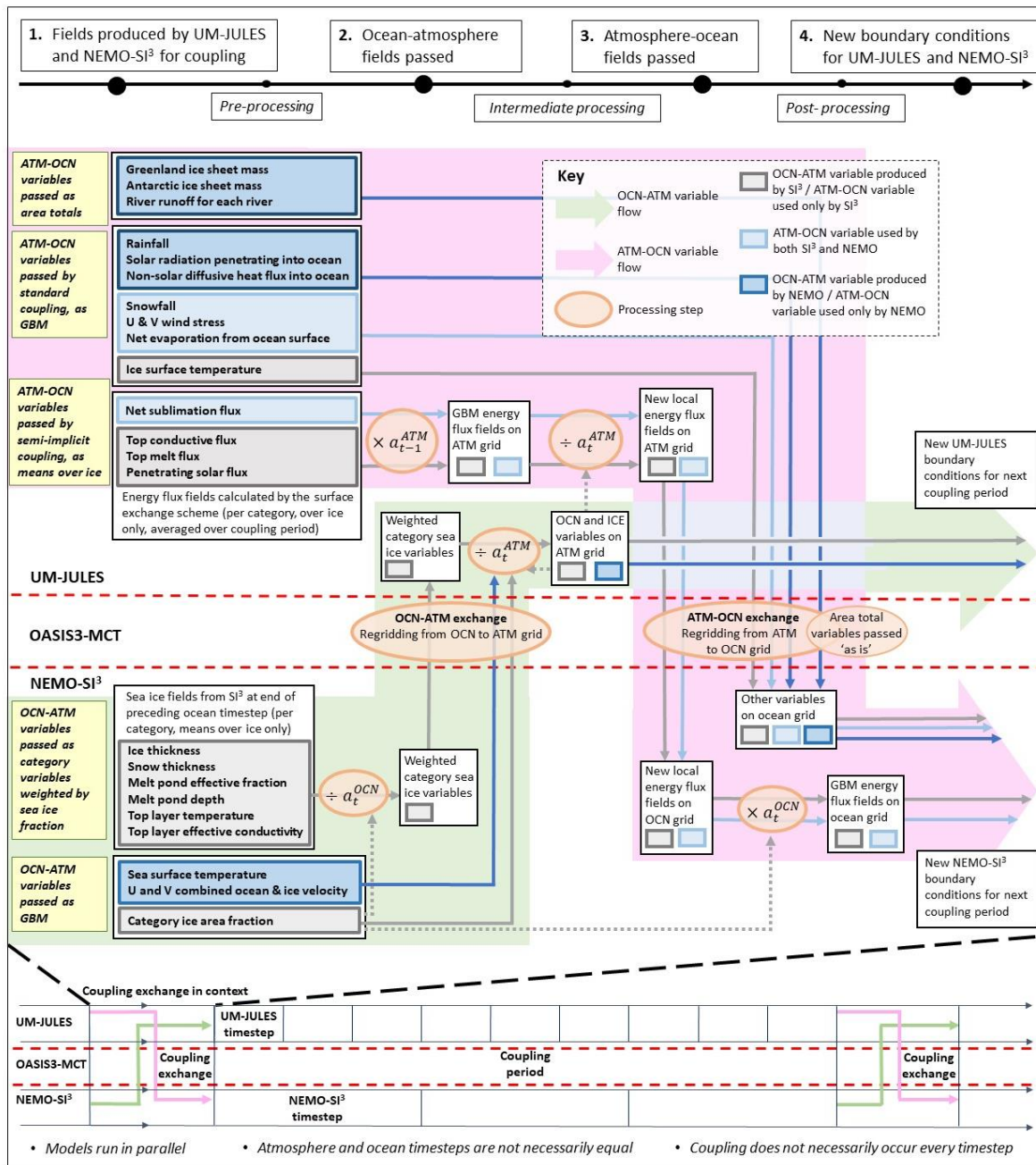
550 Figure 1: Schematic overview of the coupling between UM-JULES and NEMO-Si 3 used in GC5. The general coupling approach is illustrated in the form of a time-series across the bottom of the schematic; the upper 80% of the figure shows the detail for a single coupling instance, including a full list of variables passed in both directions with the key arithmetic operations performed on them.
