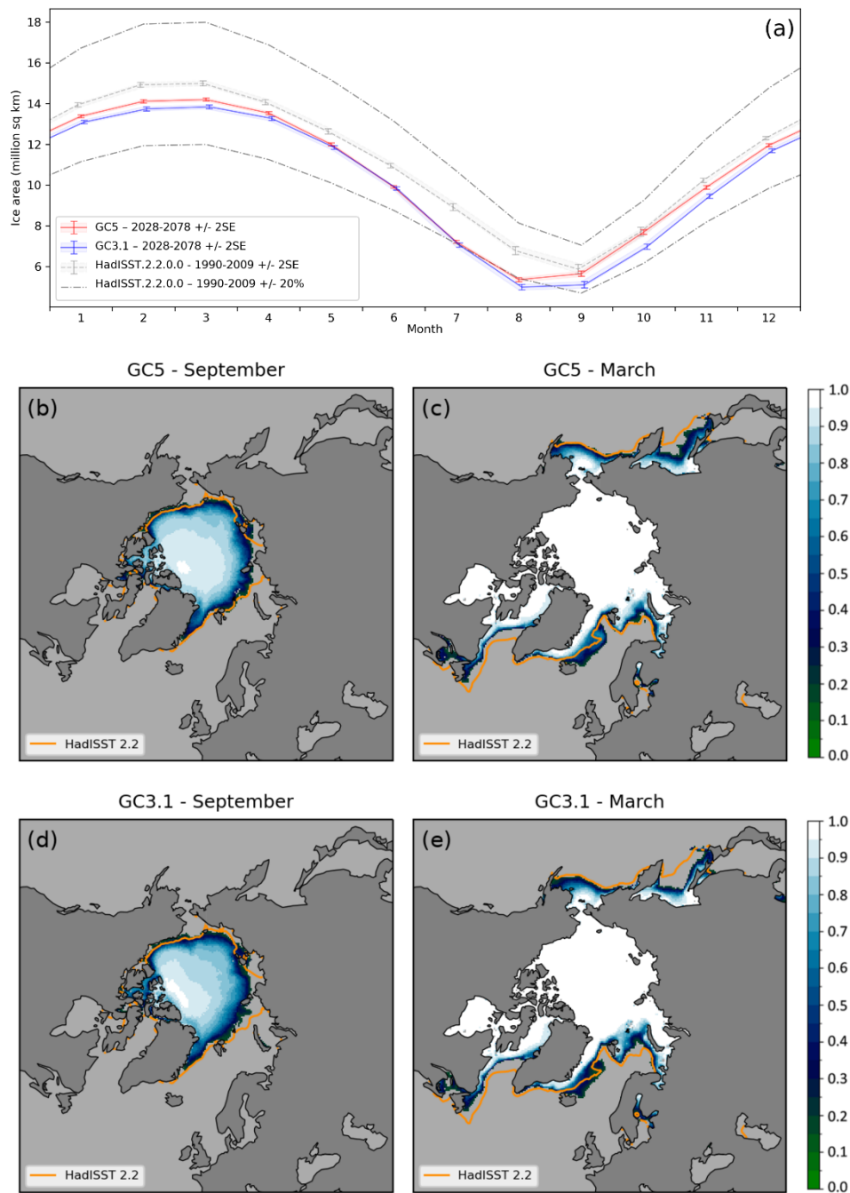
560 Figure 2: (a) The model seasonal cycle of sea ice area ( 10^6 \text{ km}^2 ) in the Arctic for GC5 (red) and GC3.1 (blue). Area estimates from the HadISST.2 sea ice dataset are included in grey, with +/- 2 standard error (SE) shading and error bars, and +/- 20% indicated with chain lines. Panels (b) – (e) show simulated mean sea ice fraction with HadISST.2 0.15 contours added in orange from GC5 (b,c) and from GC3.1 (d,e) for September and March respectively. GC5 and GC3.1 data are the last 50 years from 100-year model simulations using year-2000 continuous forcing, whilst HadISST.2 data are from the period 1990-2009.
