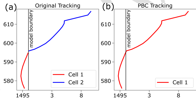
Figure 15. A depiction of 2D tobac tracking with and without accounting for PBCs. Panel (a) shows the two discrete cells that would be identified by tobac v1.2 when a feature crosses a boundary. Panel (b) illustrates the single, unified cell that is produced with the PBC tracking procedure.
