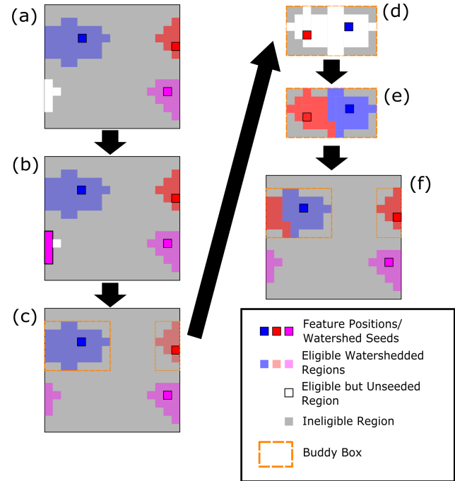
Figure B1. A depiction of two elements of the PBC segmentation treatment. In panel (a), we have two sets of regions (the red and blue shapes in one set and the magenta and white shapes in the other) that are artificially separated by a model boundary. The white shape in panel (a) is “eligible but unseeded”, meaning it exceeds the segmentation magnitude threshold but did not have a marker placed within it to conduct watershedding. Since the magenta shape is in contact with this shape across the model boundary, we first seed all adjacent boundary points (as depicted in panel b) and then use these to watershed the relevant “eligible but unseeded points” as shown in panel (c). The red and blue shapes shown in panel (a) have both been watershed by different feature markers but are artificially separated by the model boundary. This necessitates the selection of these two shapes into their own contiguous domain (the dashed orange “Buddy Box” depicted in panels c–f) so that watershedding can be performed again to obtain the correct segmentation boundaries. After transforming these grid points and their included data into the Buddy Box domain as shown in panel (d), we place our feature markers (the red and blue boxes with black outlines) in the domain and perform watershedding again, as shown in Panel (e). Subsequent to the Buddy Box watershedding, the correct segmentation regions are transformed back into the original domain, as shown in Panel (f). Boxes with bright colours and black outlines depict the feature markers used for watershedding, the paler corresponding colours denote the regions segmented by these markers through watershedding, the white boxes denote “eligible but unseeded” regions (i.e. above the segmentation magnitude threshold but not marked by a feature), and the gray boxes denote regions that are beneath the magnitude threshold and are not eligible to undergo watershedding.
