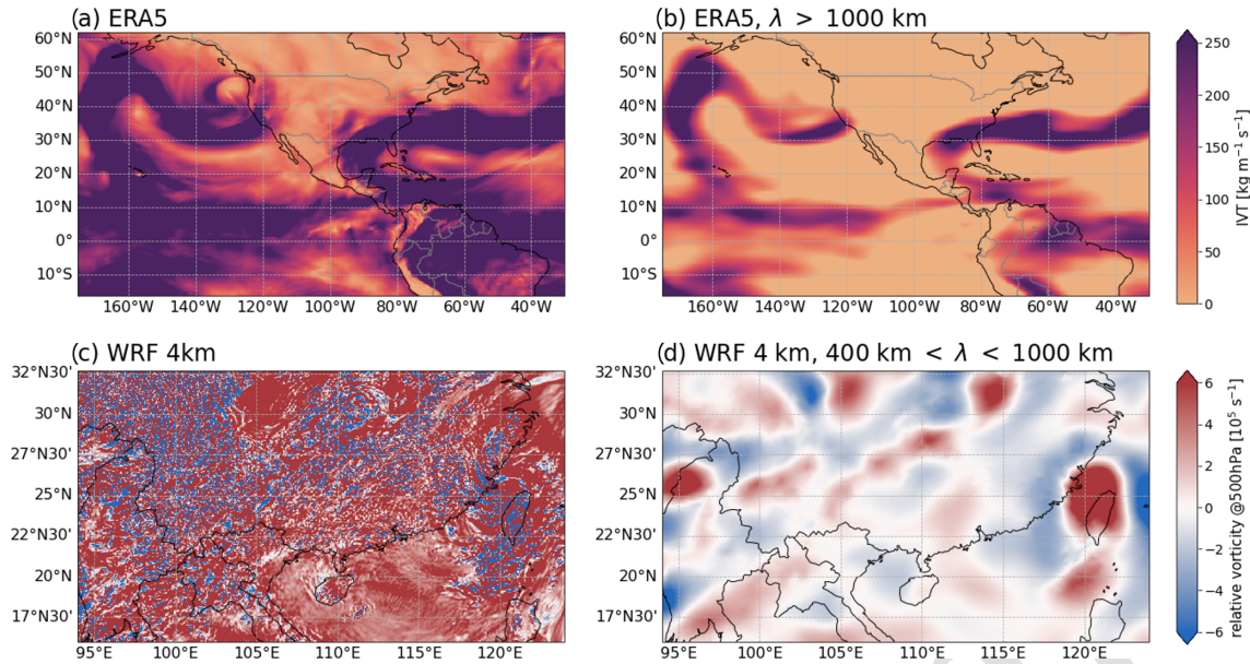
Figure 11. Examples for hourly atmospheric input fields ( a , c ) and their corresponding spectrally filtered fields ( b , d ). ( a ) Vertically integrated water vapour transport (IVT) [ \text{kg m}^{-1} \text{s}^{-1} ] from ERA5 at 27 January 2021 10:00:00 UTC showing an atmospheric river over the San Francisco Bay area. ( b ) The same as in ( a ) but spectrally filtered for wavelengths > 1000 km. ( c ) Relative vorticity at 500 hPa [ 10^5 \text{s}^{-1} ] from a WRF simulation with 4 km grid spacing over Southeast Asia for 18 July 2008 05:00:00 UTC (when Typhoon Kalmaegi hit Taiwan). ( d ) Same as in ( c ) but spectrally filtered for wavelengths between 400 and 1000 km. Note that the typhoon over Taiwan only becomes visible in the vorticity field after the filtering has been applied because the original vorticity field is dominated by sub-mesoscale noise.
