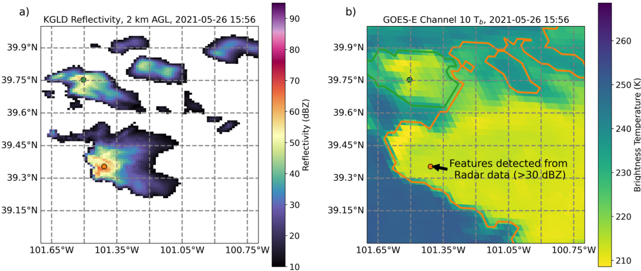
805 Figure 13: A depiction of the output from the new procedure for differently gridded data included in tobac v1.5. Panel (a) shows NEXRAD radar reflectivity in dBZ from the Goodland, KS site at 15:56 UTC on 26 May 2021, as well as the associated features detected at a 30 dBZ threshold marked by coloured dots which represent different convective cores. Panel (b) shows GOES-16 satellite observed brightness temperature in K (initially on a different grid from the radar data), as well as the segmentation masks associated with each of these features as differently coloured outlines. The segmentation outlines shown in panel (b) are produced after regridding the satellite data to the same grid as the radar data and depict the upper-level cirrus shields associated with the different convective cores seen in the radar data.
