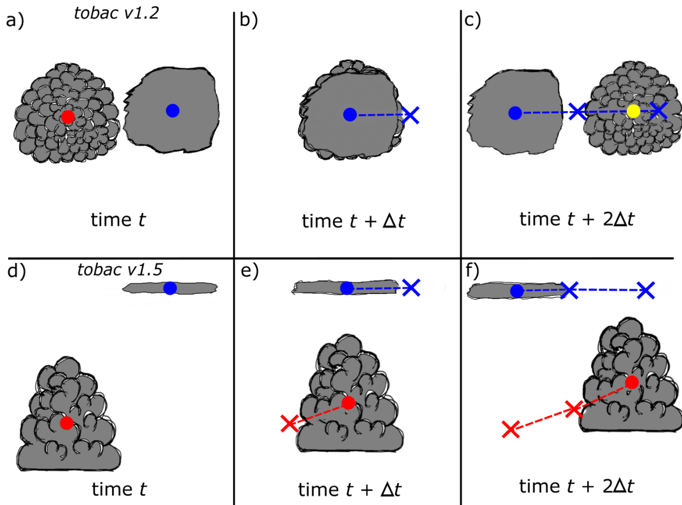
735 Figure 3: A depiction of tobac v1.2 (top row, plan view) and tobac v1.5 (bottom row, vertical cross section) feature detection and tracking for a scenario with upper-level cirrus moving over a cumulus cloud developing in a sheared environment. Each column's panels are depictions from the same time. The tobac v1.2 approach pictured in the top row fails to capture the temporal evolution and vertical propagation of the cumulus cloud due to the overlying cirrus, and even incorrectly recognizes the cumulus in panel (c) as a completely new feature and track from its earlier stage in panel (b). In contrast, the tobac v1.5 approach consistently and continuously identifies each cloud due to their separation in 3D space, resulting in correctly linked cloud tracks for each of the cirrus and cumulus. The coloured circles denote different features at their present times in each panel, with the coloured X's indicating their position at previous times and the dotted lines representing the corresponding tracks. The symbol t here denotes a generic starting time, while \Delta t denotes the timestep from scene to scene. 740
