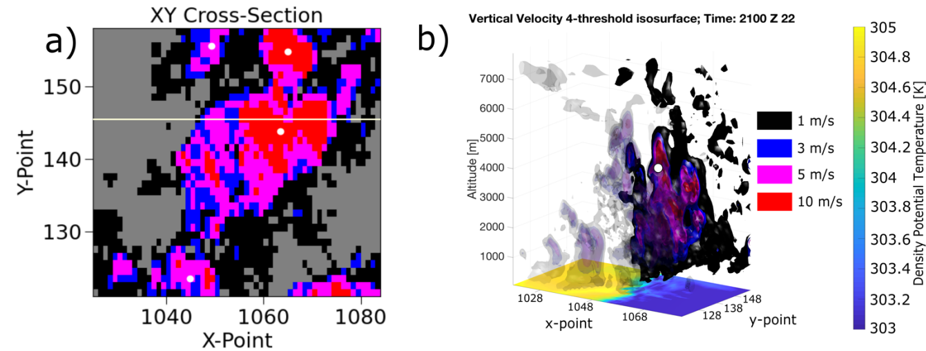
Figure 2: An illustration comparing cross-sections of 2D and 3D updraft four-threshold feature detection on the same model 3D vertical velocity field. Panel (a) shows the projection of column maximum vertical velocity and the multiple features contained in this area as white dots, while panel (b) shows a cutaway 3D isosurface plot of a 3D updraft detected at the 10 m/s threshold covering the same area as panel (a). Black, blue, magenta, and red shading indicate pixels exceeding the 1 m/s, 3 m/s, 5 m/s, and 10 m/s thresholds, the white dots illustrate feature positions within each cross-section, and the white line in panel (a) represents the location of the front-left cutaway in panel (b), ahead of which (in y-point space) transparent isosurfaces are used to reveal the complex inner
