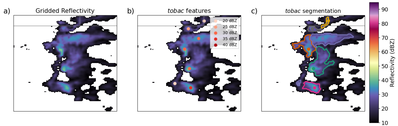
Figure 1: Demonstration of tobac feature detection and segmentation of NEXRAD radar reflectivity data at 2 km above ground level from the Cheyenne, WY radar (located just to the NW of the domain shown here) on 25 May 2017 during the C 3 LOUD-Ex field campaign (van den Heever et al., 2021). Panel (a) shows the actual radar data, panel (b) displays the objectively identified radar reflectivity features for thresholds of 20, 25, 30, 35, and 40 dBZ as dots with a progressively darker red colour at higher magnitude, and panel (c) shows the reflectivity segmentation regions associated with the features as differently coloured outlines. The straight grey lines depicted in each panel represent state borders.
