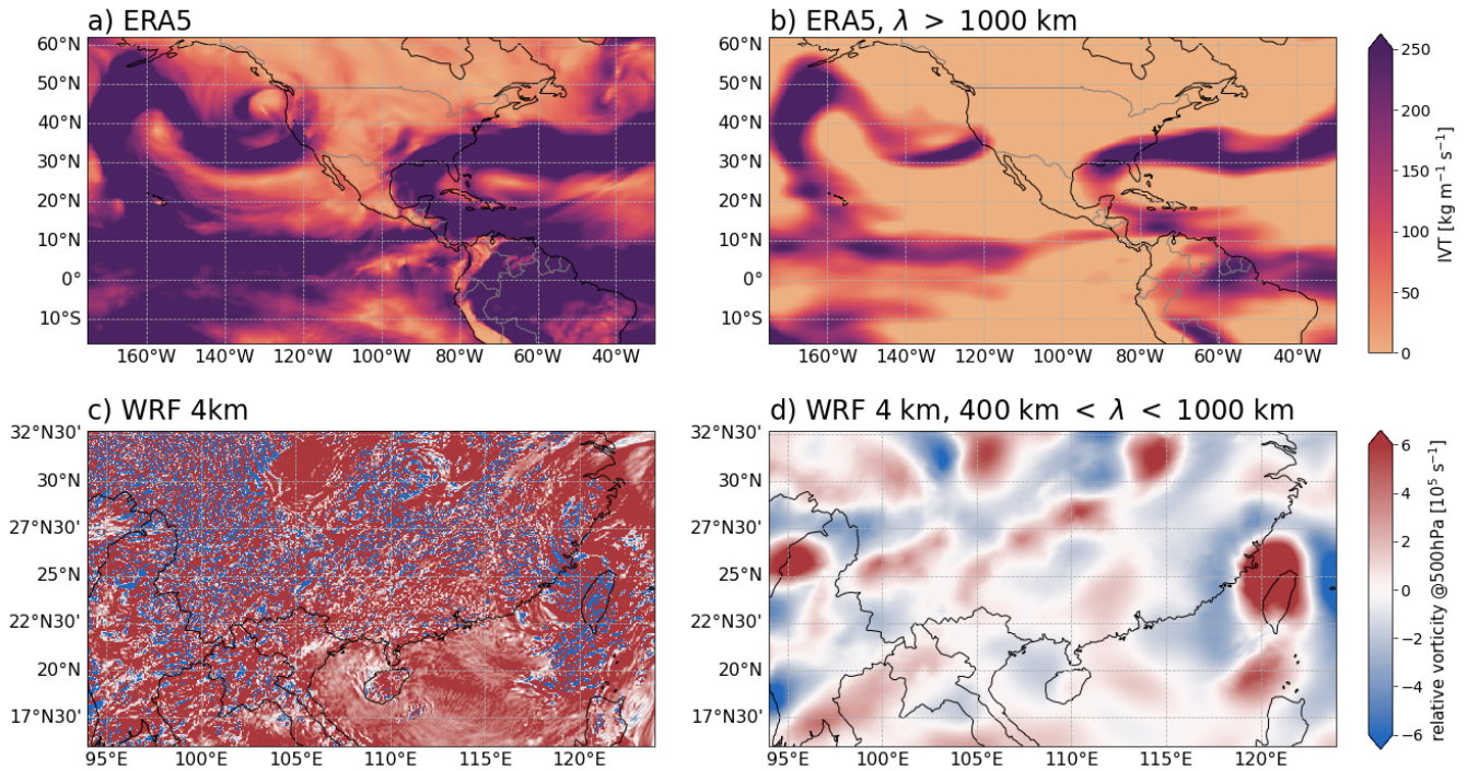
Figure 11: Examples for hourly atmospheric input fields (a, c) and their corresponding spectrally filtered fields (b, d). a) Vertically integrated water vapor transport (IVT) [ \text{kg m}^{-1} \text{s}^{-1} ] from ERA5 at 2021-01-27 10:00:00 UTC showing an atmospheric river over the San Francisco Bay area b) Same as in a) but spectrally filtered for wavelengths > 1000 km, c) Relative vorticity at 500 hPa [ 10^5 \text{s}^{-1} ] from a WRF simulation with 4km grid spacing over Southeast Asia for 2008-07-18 05:00:00 UTC (when Typhoon Kalmaegi hit Taiwan) d) Same as in c) but spectrally filtered for wavelengths between 400 and 1000 km. Note that the typhoon over Taiwan only becomes visible in the vorticity field after the filtering has been applied, because the original vorticity field is dominated by sub-mesoscale noise.
