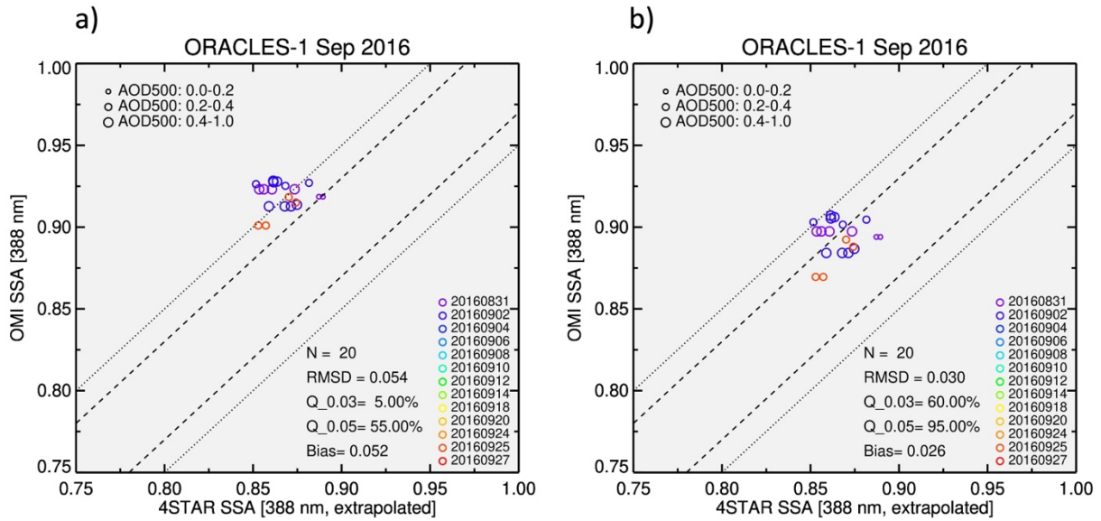
1330 Figure 9. Comparison of spatiotemporally collocated above-cloud aerosol SSA retrieved from OMI (388 nm) against those derived from 4STAR sunphotometer sky scan observations for the ORACLES-1 September 2016 campaign. The OMI SSA retrievals using the original aerosol model (a, left) with 20% relative spectral dependence in the imaginary part of the refractive index (AAE \sim 2.45-2.60) and modified aerosol model (b, right) with 10% spectral dependence in the imaginary index (AAE \sim 1.72-1.87) are evaluated against those of 4STAR inversions. The Q_0.03 1335 and Q_0.05 are the % matchups falling within the relative difference of \pm 0.03 and \pm 0.05, respectively. The OMI- 4STAR matchups are color-coded according to the date of observations shown in legends. The sizing of the circles corresponds to the magnitude of coincident AOD (500 nm). The statistical measures of the comparison are printed in the lower left of each plot.
