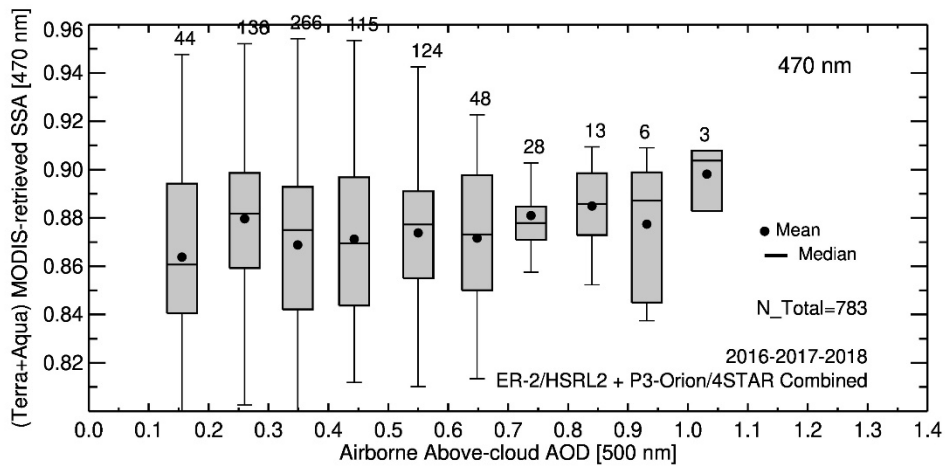
1310 Figure 7 Satellite-retrieved above-cloud aerosol SSA at 388 nm (top) and 470 nm (bottom) as a function of coincident airborne ACAODs used as input to the inversion algorithm. The data are represented as a box-whisker plot for each 0.1 bin size in ACAOD. The number of data points obtained for each bin of ACAOD is shown at the top/bottom of the whisker. The satellite-airborne collocated datasets obtained from HSRL-2 and 4STAR for all three years of the ORACLES deployments are combined and included.
