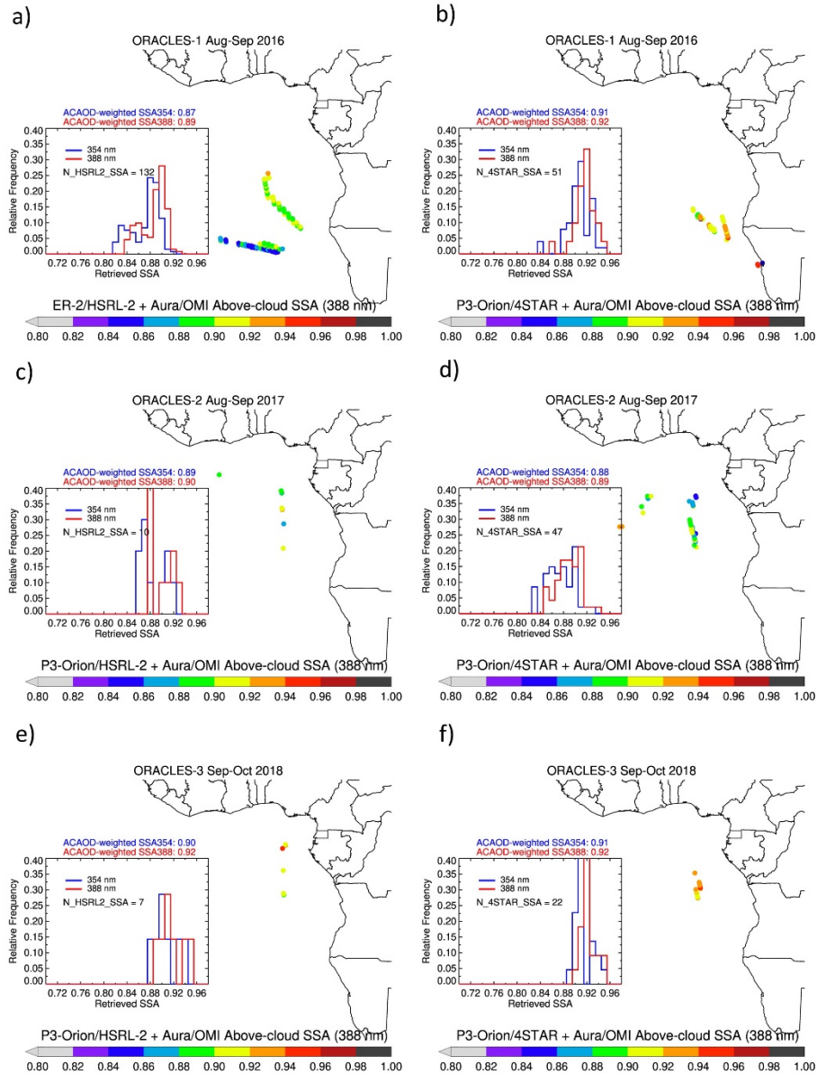
1300 Figure 5. Spatial distribution of above-cloud aerosol SSA at 388 nm retrieved from the collocated measurements of OMI radiances and airborne HSRL-2 (left column) and 4STAR (right column) ACAOD (>0.2 at 500 nm) for the ORACLES-1 (top row-a, b), -2 (middle row-c, d), and -3 (bottom row-e, f) deployments. The corresponding histograms of the retrieved spectral SSA are also shown within each plot.
