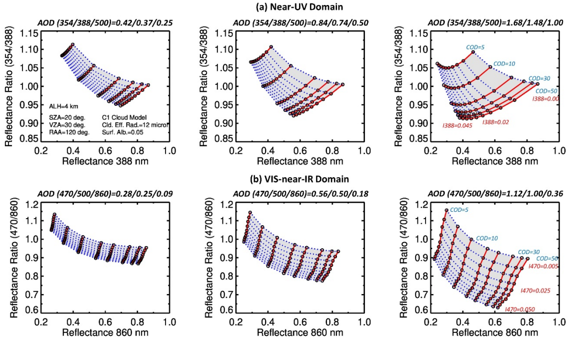
1270 Figure 1 Radiative transfer simulations of TOA reflectance in the a) near-UV (354-388 nm) and b) visible-near- 1275 infrared (470-860 nm) wavelength domains of an assumed atmosphere constituted by above-cloud carbonaceous aerosols with varying magnitudes of the imaginary part of the refractive index and COD. The simulation is carried out for the solar zenith, viewing zenith, and relative azimuth angles of 20°, 30°, and 120°, respectively, and assumed an aerosol layer with a quasi-Gaussian profile with peak concentration at 4 km above sea level placed above a half- kilometer thick cloud deck located between 850 hPa and 900 hPa. Three scenarios of aerosol loading are presented, i.e., ACAOD of 0.25 (left), 0.5 (center), and 1.0 (right) at 500 nm; ACAODs at other wavelengths were adjusted following the assumed spectral dependence of aerosol extinction. Solid (dotted) curves connecting simulations for the different values of the imaginary index (COD) represent sensitivity to aerosol absorption (cloud brightness).
