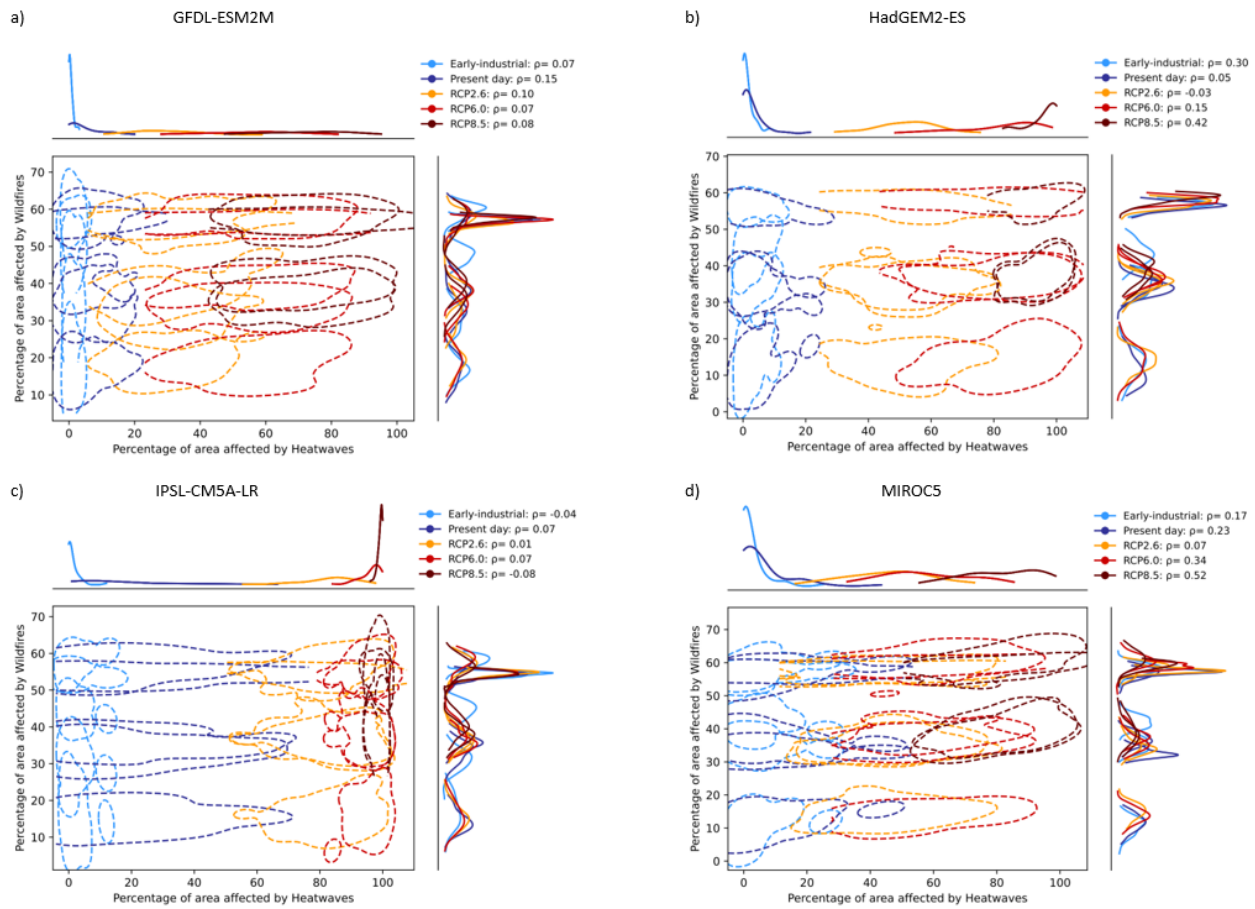
Figure 7. Bivariate distribution of heatwaves & wildfires across 50-year time periods representing the early-industrial period (1861-1910), the present day (1956-2005), and the end of century (2050-2099) under RCP2.6, 6.0, and 8.5. The figure separates the impact models by driving GCM: (a) GFDL-ESM2M, (b) HadGEM2-ES, (c) IPSL-CM5A-LR, (d) MIROC5. The \rho values represent the average value across all the impact models under their respective historical or future climate scenarios. The marginal distributions of each extreme event (per scenario), based on the KDE method (Węglarczyk, 2018), are shown along the top and right axes of the plots. The contours (dotted lines) illustrate smooth estimates of the underlying distribution of co-occurring extremes. Here, the 68 th percentile contour, which envelopes data within one standard deviation to either side of the mean, per scenario is used to show a generalized view of the distribution of the percentage of area affected by co-occurring extremes per year and per impact model driven during the respective scenarios. For each GCM, wildfire distributions for each impact model are shown separately.
