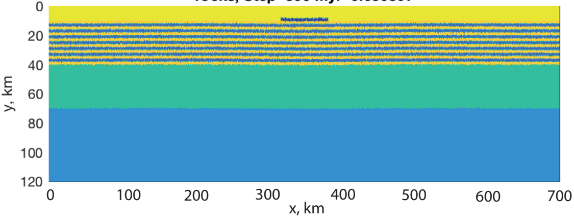
rocks, Step=390 Myr=0.050397
