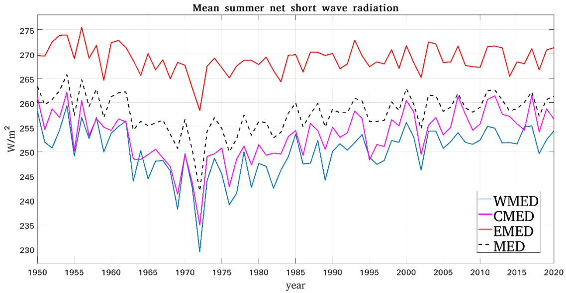
985 Figure B4: ERA5 mean Summer net short wave radiation ( W/m^2 ) in the Mediterranean Sea (1950-2020) for the entire basin (dashed black line) and for the western (extending from Gibraltar Strait to the Strait of Sicily; blue line), central (Strait of Sicily up to 22° E; purple line) and eastern (22° E eastwards; red line) sub-basins.
