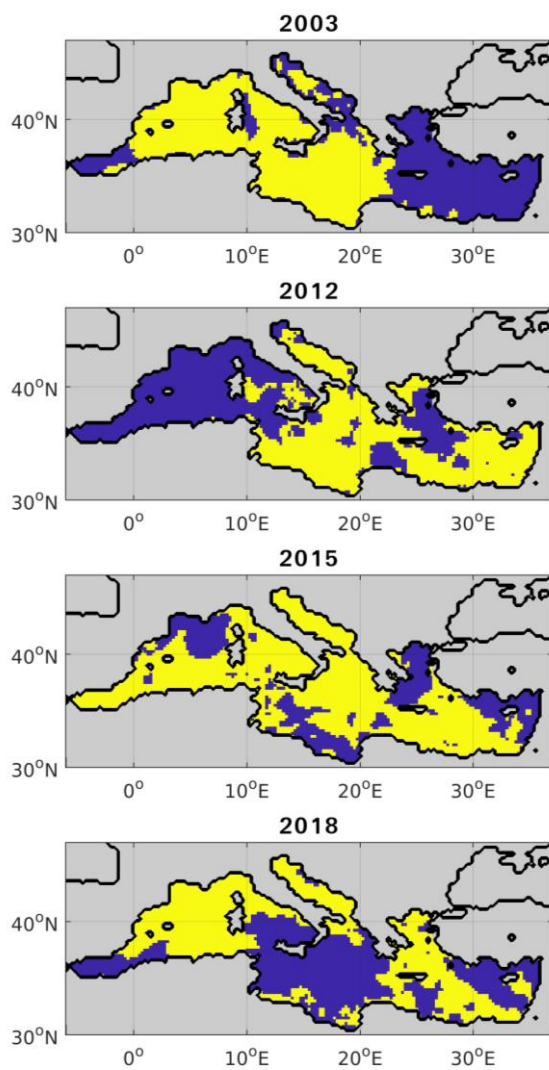
965 Figure B1: Spatial extent of EMSs concentrating more than 50% of the Mediterranean Sea grid points: 2003, 2012, 2015 and 2018 (from top to bottom, respectively). Yellow stands for areas experiencing EMS conditions and blue for non-EMS conditions.
