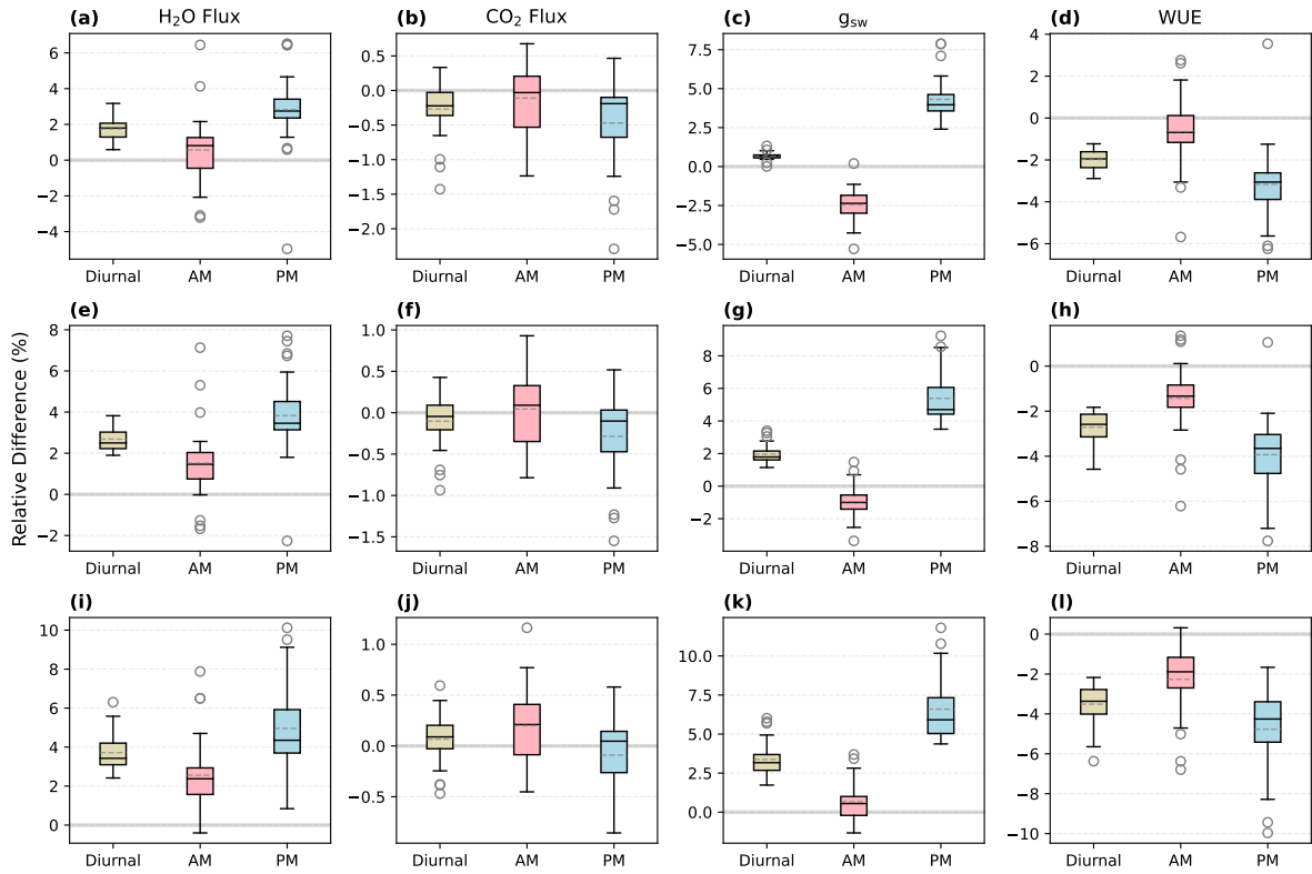
Figure S3: Relative differences (NSS - SS; RD) in the predicted daytime-mean fluxes of the NSS and SS simulations for August 2017, for results when \tau_{op}/\tau_{cl} < 1 . The solid line in each box indicates the median, and the dashed line represents the mean. The results for the transpiration rate (H 2 O flux), net productivity (CO 2 flux), canopy-averaged stomatal conductance to water ( g_{sw} ), and water-use efficiency (WUE) are shown in the respective columns from left to right. (a-d) \tau_{op} = 750 s, \tau_{cl} = 900 s, (e-h) \tau_{op} = 600 s, \tau_{cl} = 900 s, (i-l) \tau_{op} = 450 s, \tau_{cl} = 900 s. Diurnal: 5:00-19:00, AM: 5:00-12:00, PM: 12:00-19:00.
