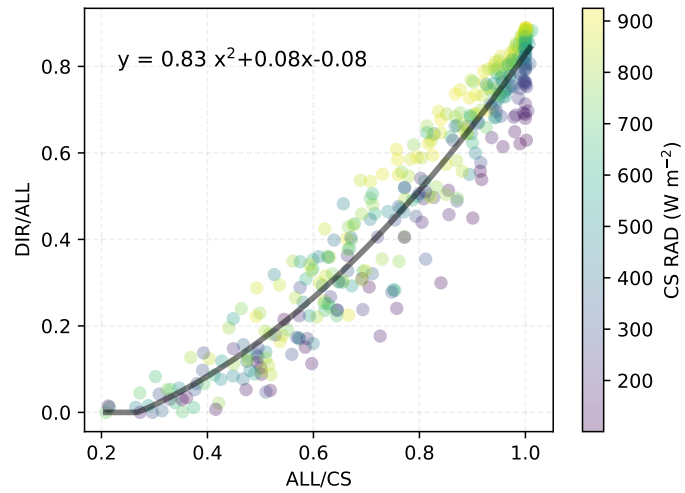
Figure S2: The empirical relationship between the direct radiation (DIR) fraction and the ratio between the total downward solar radiation (ALL) and the clear sky radiation (CS) in August 2017, filtered by 100 \text{W m}^{-2} CS radiation. Radiations are from the ERA5-Land hourly dataset.
