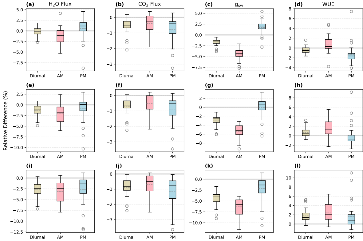
Figure S4: Relative differences (NSS - SS; RD) in the predicted daytime-mean fluxes of the NSS and SS simulations for August 2017, for results when \tau_{op}/\tau_{cl} > 1 . The solid line in each box indicates the median, and the dashed line represents the mean. The results for the transpiration rate (H 2 O flux), net productivity (CO 2 flux), canopy-averaged stomatal conductance to water ( g_{sw} ), and water-use efficiency (WUE) are shown in the respective columns from left to right. (a-d) \tau_{op} = 900 s, \tau_{cl} = 750 s, (e-h) \tau_{op} = 900 s, \tau_{cl} = 600 s, (i-l) \tau_{op} = 900 s, \tau_{cl} = 450 s. Diurnal: 5:00-19:00, AM: 5:00-12:00, PM: 12:00-19:00.
