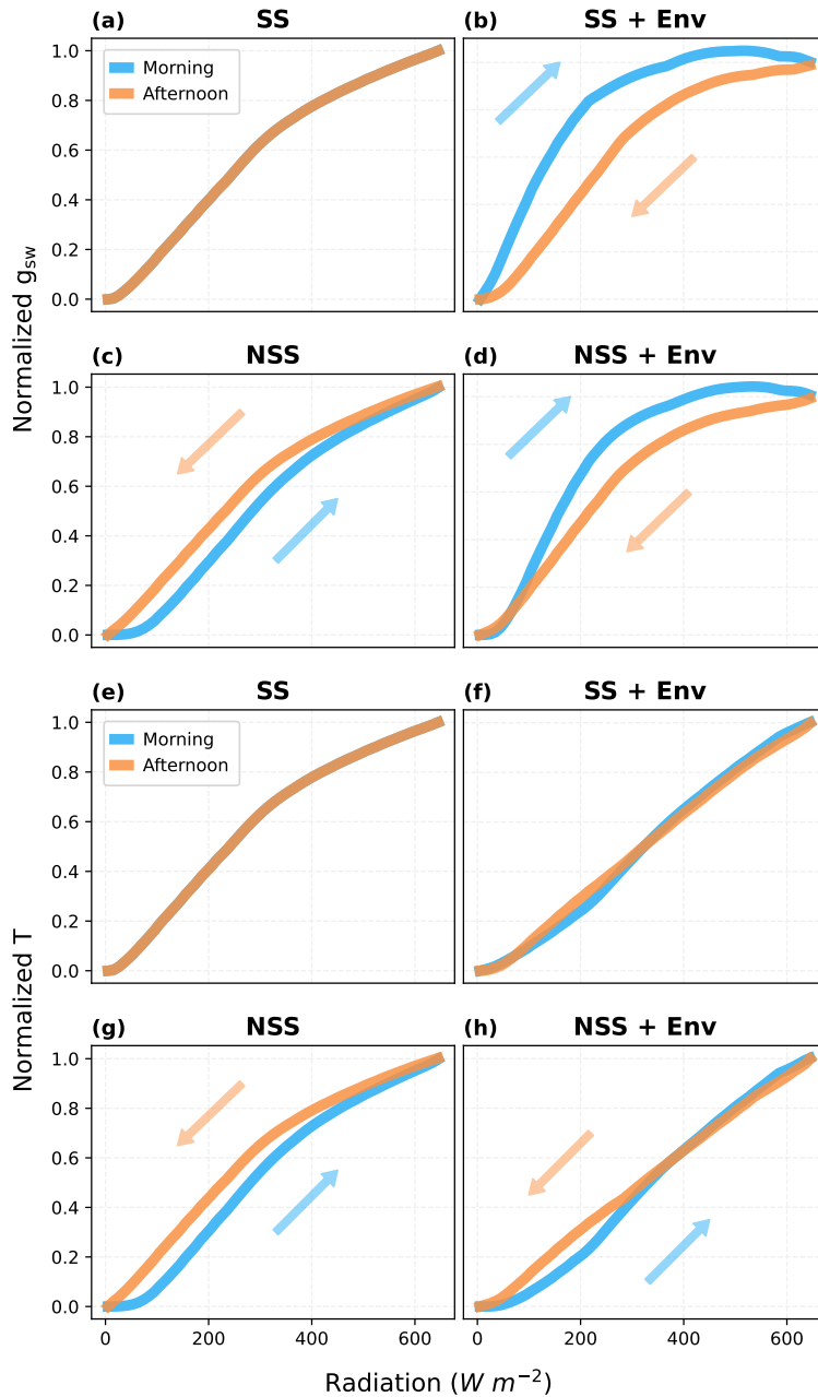
Figure S7: Hysteresis of the canopy-mean stomatal conductance ( g_{sw} ) and canopy transpiration rate ( T ) in response to radiation during an ideal clear-sky day, when \tau_{op} = 900 s, \tau_{cl} = 300 s. (a, e) SS model, (b, f) SS model with coupled diurnal variations of environmental conditions (Env, e.g. air temperature, VPD), (c, g) NSS model, (d, h) NSS model with Env. (a-d) normalized g_{sw} responses, (e-h) normalized T responses. In simulations without Env variations, except for the radiation, all the other environmental drivers were kept at the daytime means. g_{sw} and T is normalized with the values at noon (12:00). Arrows indicate the increasing and decreasing parts of the diurnal courses.
