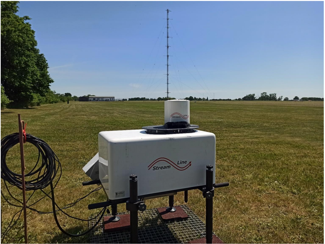
165 Figure 1: DL 2 with the 99 m tall lattice tower in the background, where a sonic anemometer is mounted at a height of 90 m above ground, on-site during the FESST@MOL 2020 campaign in Falkenberg (Tauche), Germany.
