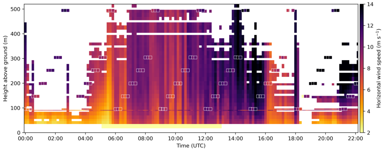
370 Figure 7: Overview of the different ten minutes mean horizontal wind speed measurement methods we used as an example for 06 July 2020. The background data are the results of the VAD 1 measurements, the white boxes show the results of the VT DL step/stare mode at the six different heights. The line at the height of 90 m above ground shows the sonic anemometer data.
