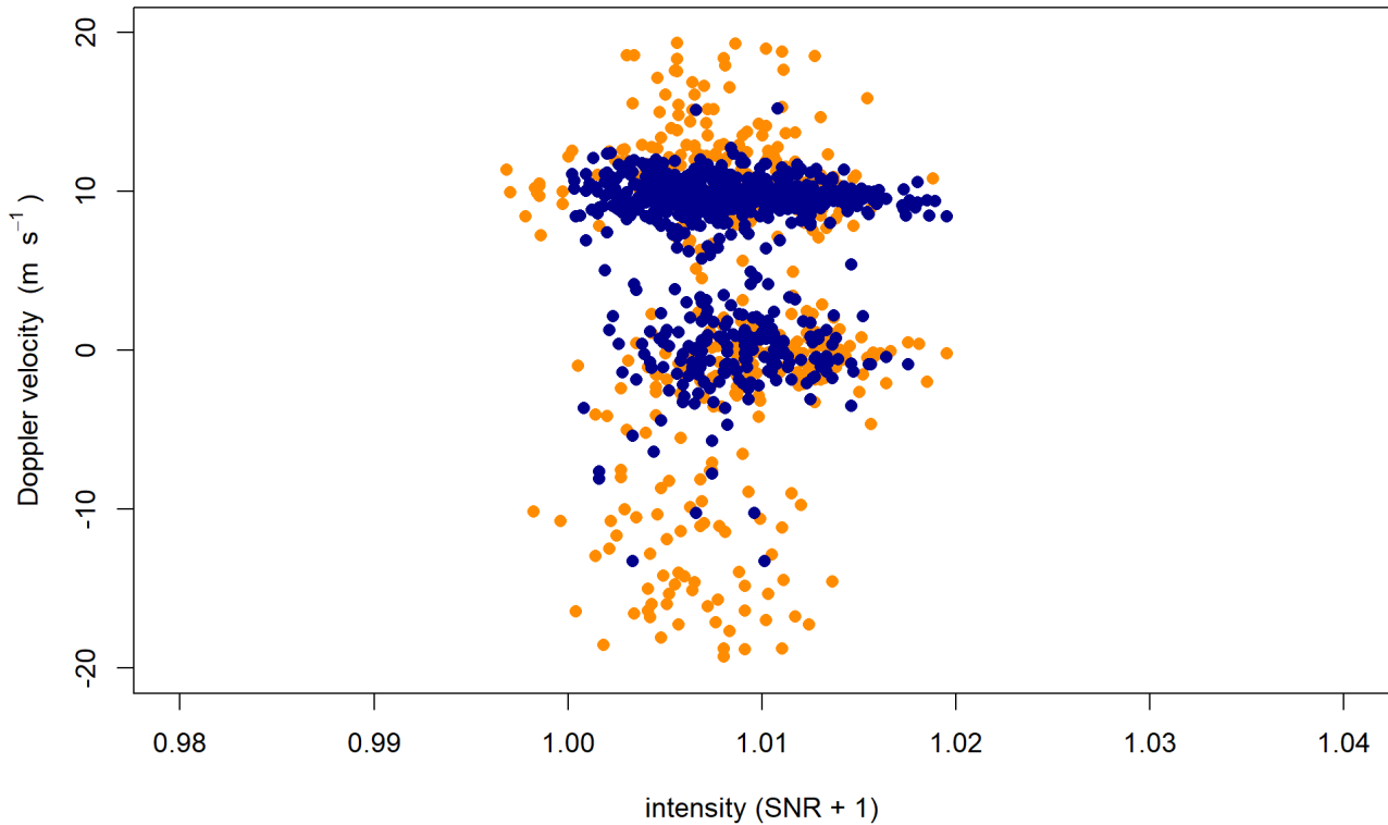
300 Figure 4: Example plot to show the problem of noise around zero, the figure shows the unfiltered data (orange) and the data after applying the SNR + 1 and MAD filters (blue) for DL 2 for the period of 10:30 – 11.00 p.m. on 06 July 2020 for a single range gate at a height of 1220 m above ground.
