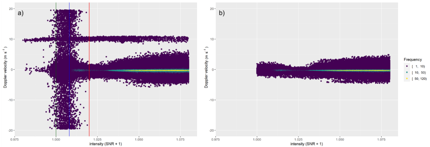
510 Figure 10: Comparison between unfiltered (a) and filtered (b) data of VS DL on 06 July 2020 at the heights of 60 m – 500 m above ground. The colored lines in a) mark the different SNR + 1 thresholds of 1.000 (dark green), 1.008 (blue), and 1.020 (red).
