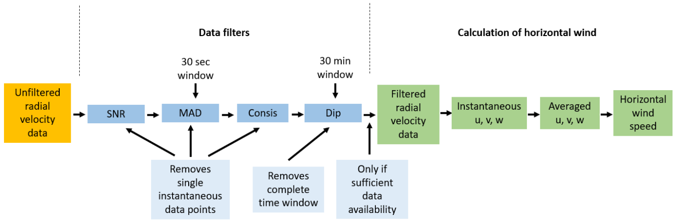
315 Figure 5: Sequence of the different data filters and processing steps used on the radial velocity data of the different DL instruments. The blue boxes represent the different filtering steps. Green are the steps that happen after applying the filters. The light blue box represents the minimum of values inside a 30 sec period and the minimum number of 30 sec periods required before averaging.
