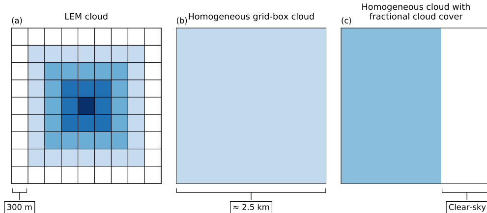
Figure 3. Illustration of the method to derive homogeneous NWP clouds from LEM clouds. The plot shows a layer of grid boxes. (a) Clouds in the LEM simulation. (b) Homogeneous grid-box cloud at a resolution of 2.5 km. (c) Homogeneous cloud with fractional cloud cover at a resolution of 2.5 km.
