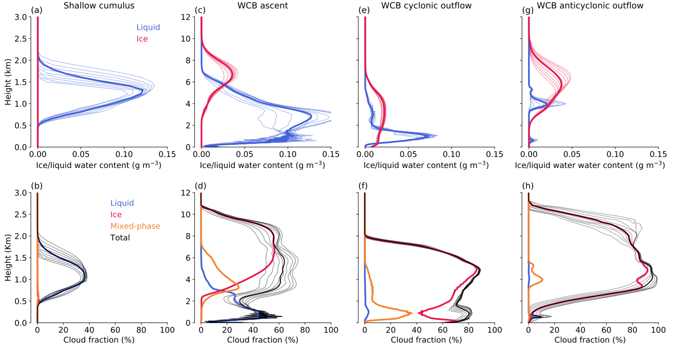
Figure 2. Profiles of domain-averaged cloud hydrometeor contents and total cloud fraction, decomposed into the contributions from liquid, ice, and mixed-phase clouds for all four LEM domains. Thin lines show profiles for nine snapshots between domain local hours 12:30 to 16:30. The thick lines show time-averaged profiles. The threshold used to determine cloudy boxes for both ice and liquid water contents is 10^{-8} kg kg -1 (Costa-Surós et al., 2020). Note the different y-axes for panels (a) and (b).
