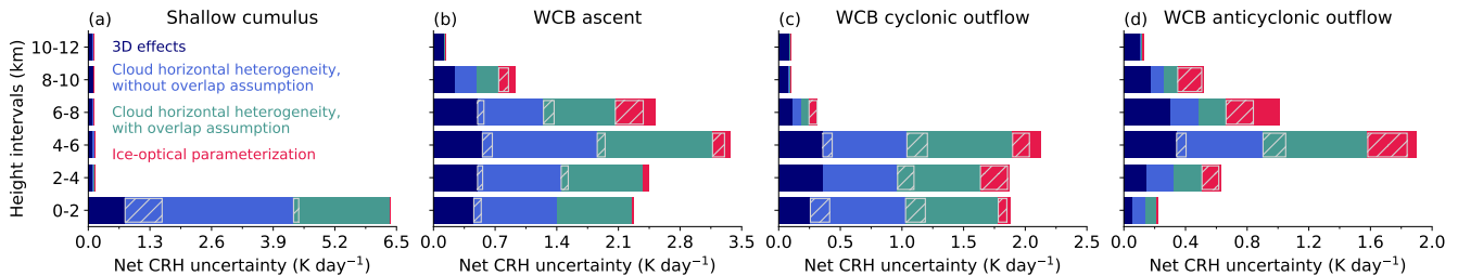
Figure 11. Same as Fig.10 but for local uncertainties of net CRH. For comparison, the mean net CRH uncertainties from Fig.10 are superimposed as gray hatched bars. The mean uncertainties smaller than 0.05 K day -1 are not shown as they would not be visible in the plot. Note the different x-axes in the panels.
