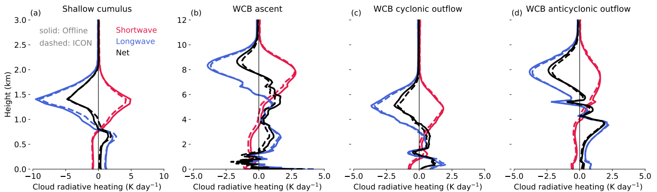
Figure 4. Domain and time averages of shortwave, longwave, and net CRH. Profiles are shown for the (a) shallow cumulus, (b) WCB ascent, (c) WCB cyclonic outflow, and (d) WCB anticyclonic outflow regions. The ICON CRH is shown in dashed lines, and the CRH derived from the offline reference 1D radiative transfer calculation is shown in solid lines. Note the different x- and y-axes between panels (a) and (b-d).
