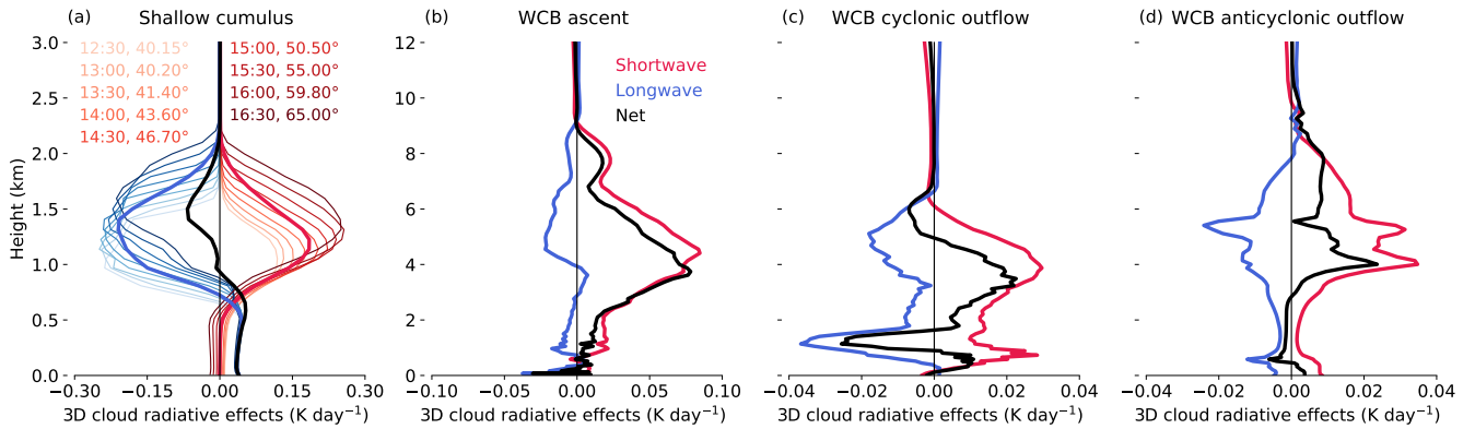
Figure 6. Average profiles of shortwave, longwave, and net 3D cloud radiative effects for the four cyclone regions. 3D cloud radiative effects are calculated as the difference in domain mean CRH between 3D (MYSTIC) and 1D (MYSTIC-ICA) radiative transfer calculations. The thin lines in panel (a) show the 3D radiative effects for nine snapshots between domain local hours 10 12:30 to 14 16:30, with the legend indicating the time and domain mean solar zenith angles for all snapshots. Note the different x-axes in panels.
