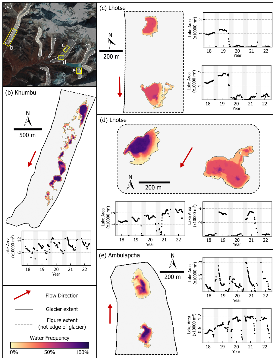
Figure 4. Water frequency maps and time series of select individual lakes or groups of lakes. Locations of each (b-e) are indicated in the top-left overview map. Lake maps are colored by water frequency (darker colors indicating more frequent water). The time series show the total area in individual Planet images. Grey shaded areas indicate monsoon season (15 June-30 September). Year tick-marks indicate the start of each year. Red arrows indicate the glacier flow direction.
