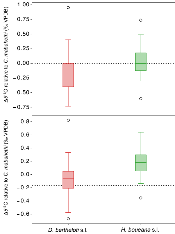
Figure 5. Box plots for the \delta^{18}\text{O} and \delta^{13}\text{C} deviations of D. bertheloti s.l. and H. boueana s.l. with reference to C. mabathethi in samples from MIS 3 of KL11.
