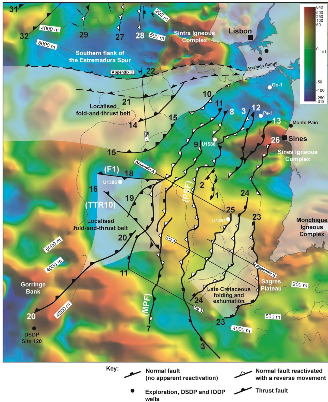
Figure 6: Structural map of SW Iberia superimposed on Differential Reduction to The Pole (DRTP) data. The map, when combined with the interpreted seismic data, highlights the presence of localised, early-stage fold-and-thrust belts between the Sintra and Sines magmatic complexes, and west of this latter. Structures mapped constitute long fault zones that are hard linked at depth to constitute >200 km long features. Note that the white triangles indicate normal faults reactivated with a reverse movement, contrasting with the common black triangles, or ‘teeth’, of thrust faults. DRTP data provided by Getech UK.
