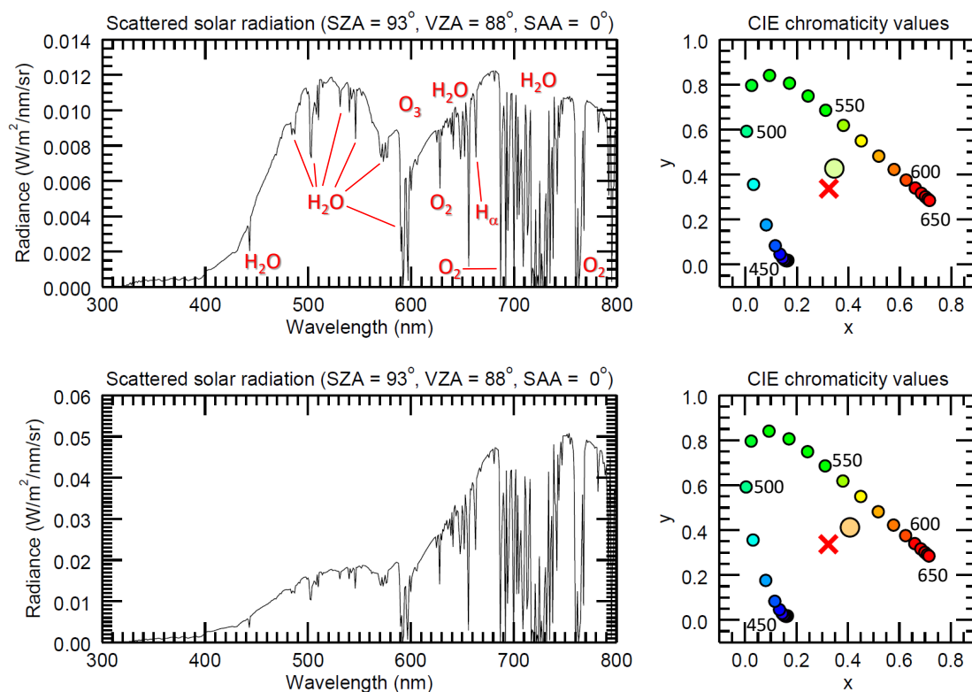
Figure 2. Spectra (left panels; note different ordinate ranges) and CIE chromaticity diagrams (right panels) for the following viewing geometry: \text{SZA} = 93^\circ , \text{VZA} = 88^\circ , \text{SAA} = 0^\circ . The simulations shown in the top row are based on the following assumptions: \text{AOD} = 0.3 , t_{med} = 650 \text{ nm} , S = 1.1 , \text{TOC} = 400 \text{ DU} . For the bottom row, the \text{AOD} has been set to zero and the other parameters remain the same. The “x” in the right column panels corresponds to the chromaticity values of the unattenuated solar spectrum. The arc of colour circles corresponds to pure spectral colours at different wavelengths (values given in nm with 10 nm steps) and the single coloured circle shows the chromaticity values of the spectrum on the left.
