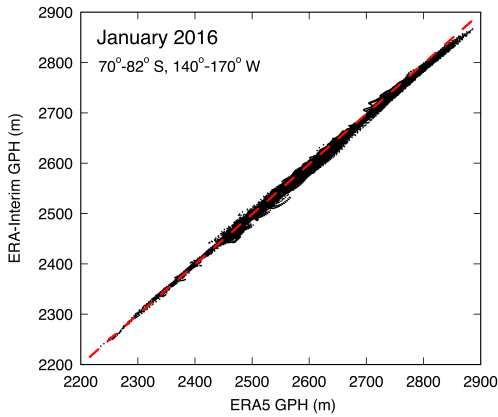
225 Figure 3: Geopotential heights at 700 hPa for ERA-Interim versus ERA5 reanalyses for an area over the eastern Ross Sea and Ross Ice Shelf. The dashed red line is the one-to-one correspondence.
