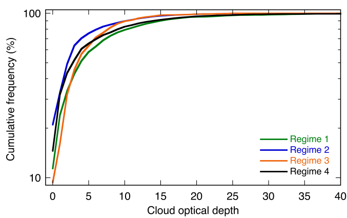
Figure 9: Cumulative frequency distributions of conservative-scattering cloud optical depth under overcast skies, for each of the four meteorological regimes.
