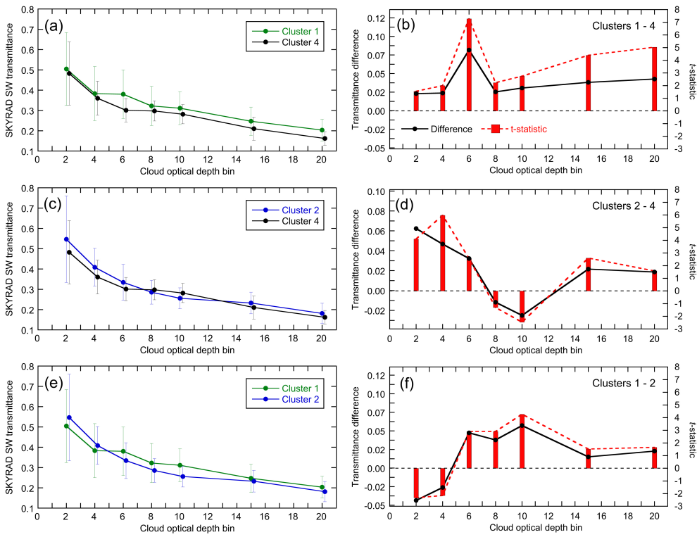
420 Figure 10: SKYRAD measured shortwave atmospheric transmittance as a function of conservative-scattering cloud optical depth bin, comparing meteorological regimes 1, 2 and 4. Each pair of panels shows the individual mean transmittances for the optical depth bins (left), then the transmittance difference between the two compared regimes (in legend) along with the statistic from Student's t -test (right). Error bars are plus/minus one standard deviation. Cloud optical depths are of width 2 for the first five bins, then 5 for the largest bins, and are identified on these plots by their upper bound. For the range of sample sizes considered here, a t -statistic \geq 2.0 indicates statistical significance.
