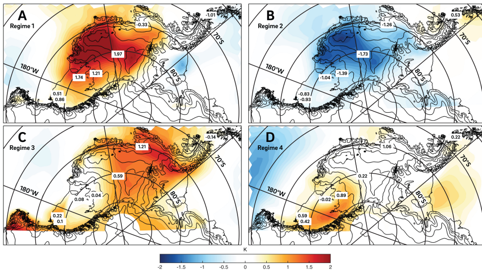
175 Figure 2: Anomalies of ERA-Interim-based 2 m near-surface air temperature (color bar) for each of the four meteorological regimes identified by the k -means clustering technique for the summer months (DJF). Numbers overlaid on these maps are observed 2 m air temperature anomalies computed from six University of Wisconsin automatic weather stations (Lazzara et al. 2012). Solid lines depict topography in steps of 500 m.
