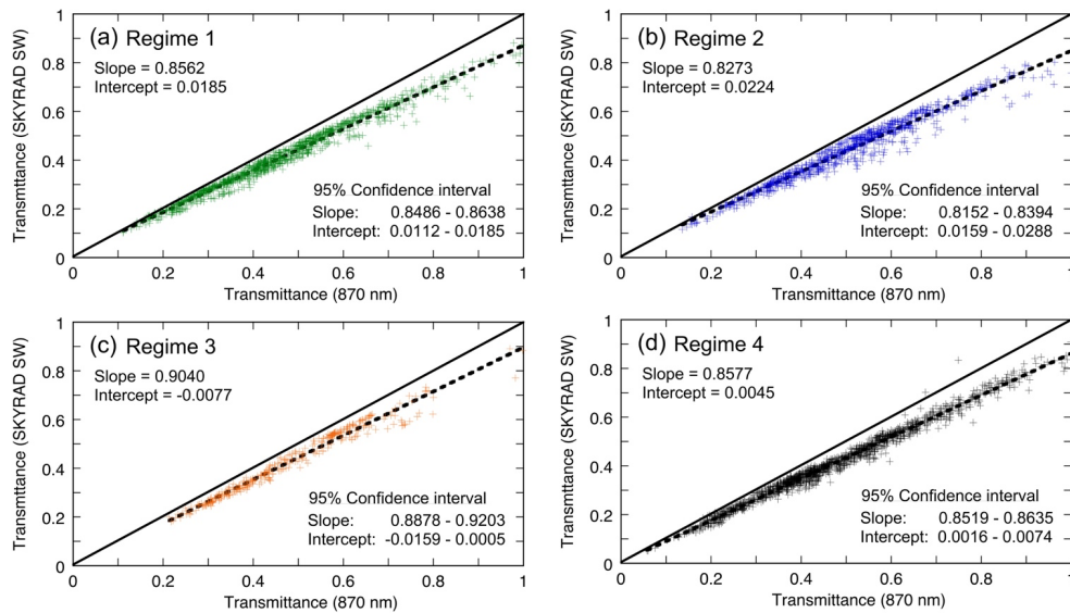
335 Figure 7: Broadband shortwave transmittance as measured by the SKYRAD as a function of narrow-band transmittance at 870 nm as measured by the MFRSR under all overcast skies throughout the austral summer 2015-16, for each of the four meteorological regimes. The solid line depicts one-to-one correspondence. The dotted line depicts a linear regression, with the slope and intercept and the 95% confidence intervals on the slope and intercept given in each panel.
