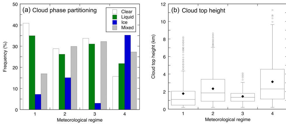
240 Figure 4: MODIS retrievals of cloud properties throughout the austral summer 2015-16 in a 1° x 1° latitude x longitude grid cell over McMurdo Station, and sorted by the four meteorological regimes from the k-means clustering analysis: (a) cloud thermodynamic phase; (b) cloud top height. In the second panel the box encloses the middle 50% of the distribution (lower quartile to upper quartile), the median is depicted by the dividing line, and the diamond depicts the mean value. The lines extending above and below each box depict nearly the entire distribution. Individual points above these lines represent individual outliers whose values are greater than the upper quartile value plus 1.5 times the interquartile distance. 245
