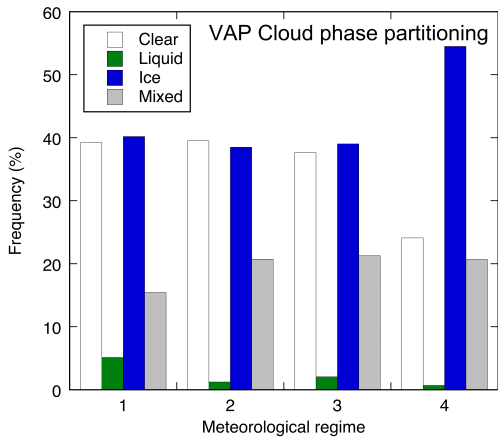
265 Figure 5. As in Figure 4a but for the ARM THERMOCLDPHASE High Spectral Resolution Lidar phase retrievals for the highest detected cloud layer above the AWARE site on Ross Island.
