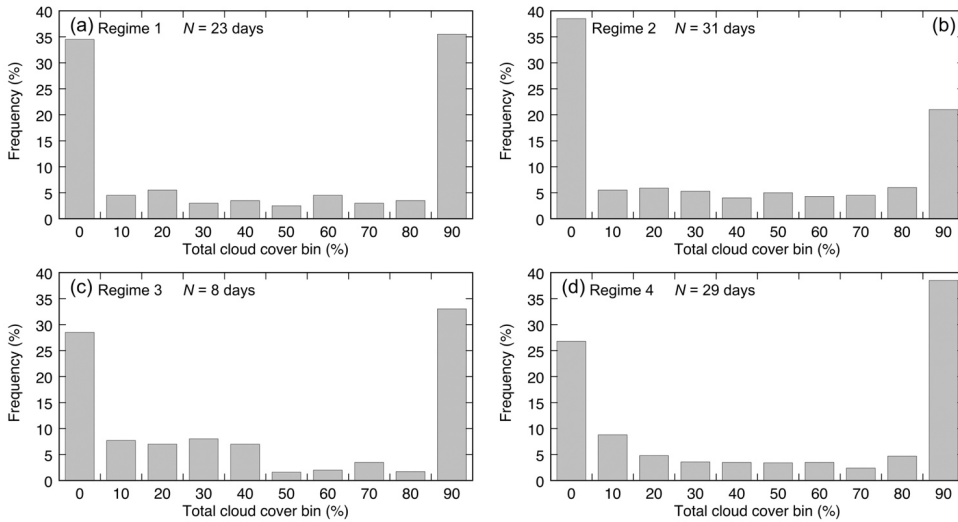
295 Figure 6: Histograms of total cloud cover measured by the TSI on Ross Island throughout the austral summer 2015-16, for each of the four meteorological regimes. The bins are identified by their lower bound, with the exception of the clear sky bin, which depicts coverage in the range 0-5%. The number of days each regime occurred is given on each panel.
