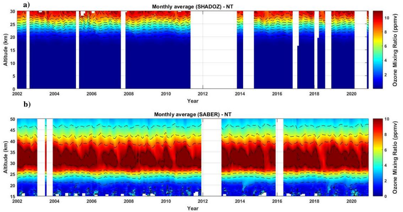
760 Figure 2: Time-height cross-section of monthly averages of ozone mixing ratio (in ppmv) over Natal (a) from radiosonde, and 765 (b) from SABER instrument, respectively in the 0-30 km and 15-50 km altitude ranges, from January 2002 to December 2020.
