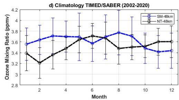
Figure 7: Monthly climatological OMR values (in ppmv) for SM (in blue) and NT (in black) from SABER records from 2002 to 2020 at 4 selected heights: 24 km, b) 32 km, c) 40 km and d) 48 km. The vertical bars represent \pm 1\sigma (standard-deviation).
