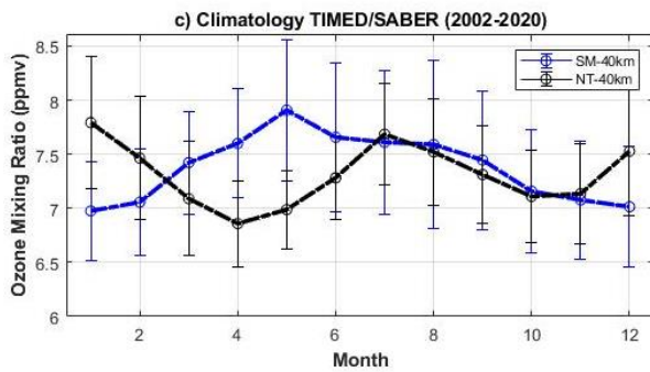
Figure 7: Monthly climatological OMR values (in ppmv) for SM (in blue) and NT (in black) from SABER records from 2002 to 2020 at 4 selected heights: 24 km, b) 32 km, c) 40 km and d) 48 km. The vertical bars represent \pm 1\sigma (standard-deviation).
