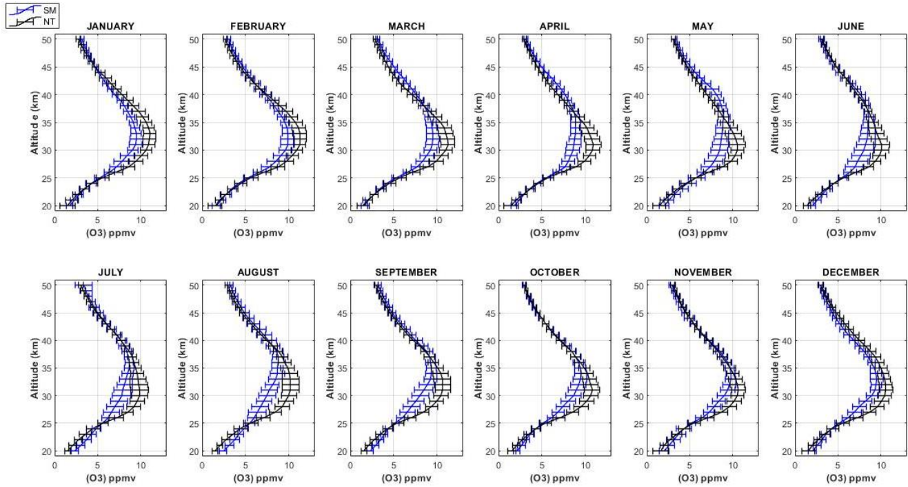
825 Figure 5: Comparison of monthly climatological OMR profiles between Santa Maria (blue) and Natal (black) using SABER data, during 2002 – 2020, between 20 and 50 km of altitude. The horizontal bars represent \pm 1\sigma (standard-deviation). The monthly climatological OMR vertical profiles are given in ppmv.
