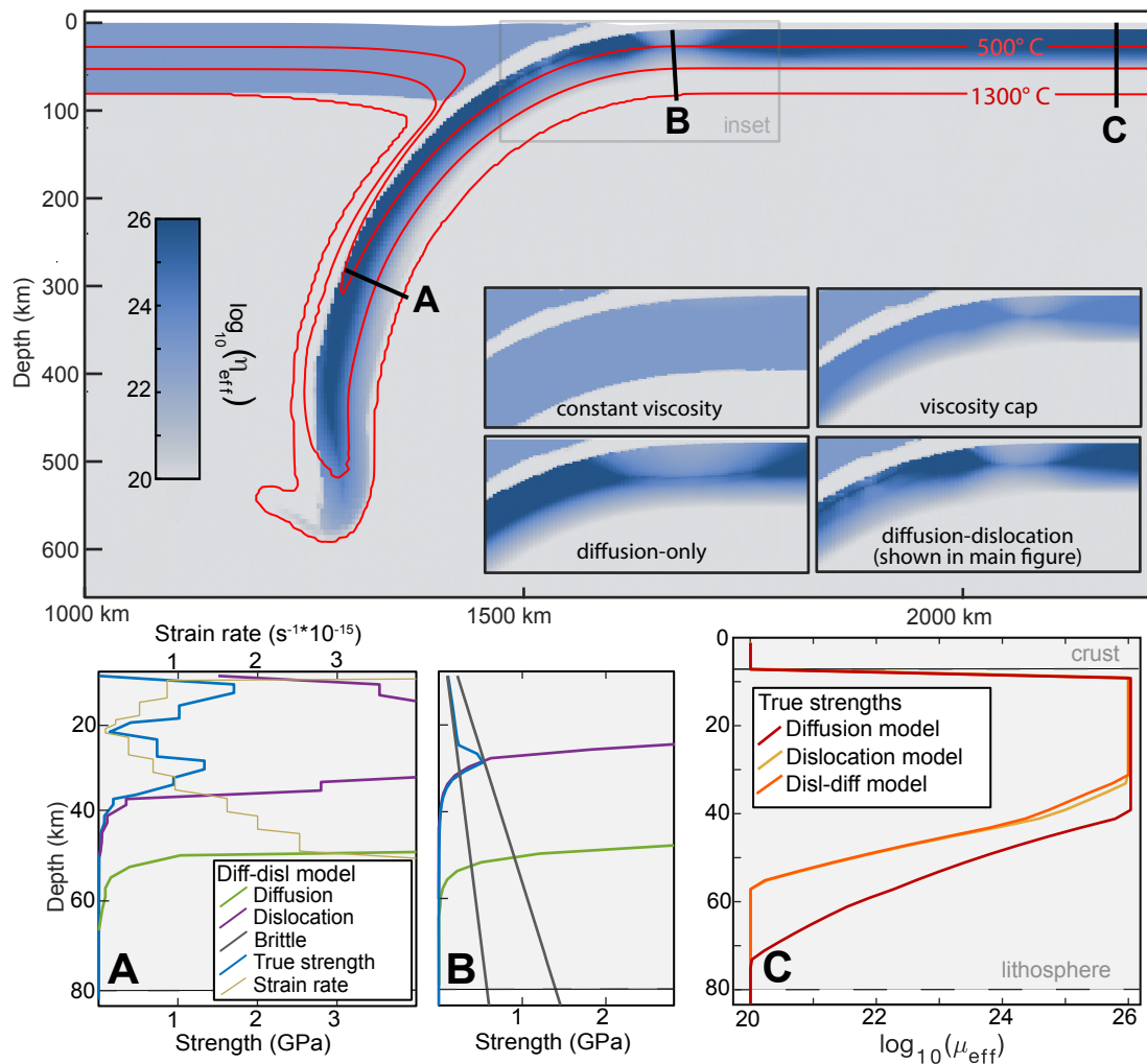
Figure 5. An image of the viscosity structure of a slab following dislocation and diffusion creep laws after 10 million years. Plots along profiles A and B show the strength of the slab (blue), compared to the strengths predicted by dislocation creep (purple), diffusion creep (green), and brittle failure (gray) with \phi = 20^\circ and \phi = 10^\circ under local strain rates and pressures. Profile A shows strength at middle depths of the upper mantle, where the upper half of the slab hits the viscosity cap and no brittle deformation is active. The thin yellow line shows strain rate (top axis), which reaches a minimum approximately 20 km into the slab. Plot B shows strength at the surface near the trench where the slab bends and undergoes brittle deformation. Plots in C show viscosity vs depth in the diffusion, dislocation, and diffusion-dislocation slabs. These plots represent un-subducted lithosphere with strain rates too low for plastic deformation. The location of these profiles is indicated on the model image. The insets show the viscosity structures of slabs where they bend at the trench. Each snapshot is taken from a similar point in the subduction process, with the slab tip approximately 100 km from the bottom boundary. All models have some plastic failure in this region, but the degree to which plastic failure lowers bending resistance is much higher in the creep-governed models than in the constant-viscosity model.
