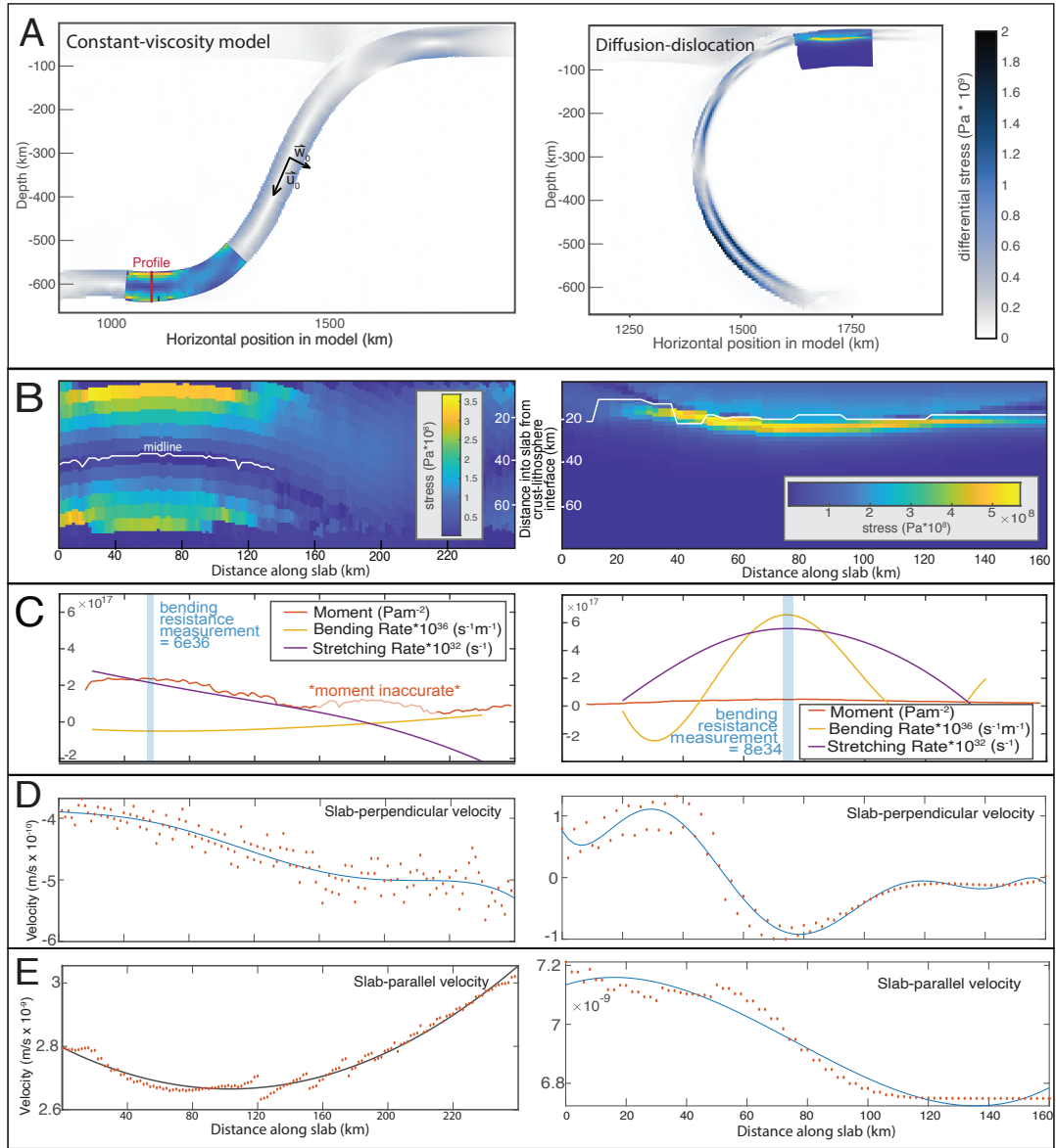
Figure A2. Panel A shows images of the constant 10^{23} Pas reference slab (left) and the diffusion-dislocation slab with a viscosity cap of 10^{26} Pas (right). Plots are colored by differential stress. Highlighted sections show where curvature, bending rate, etc. are calculated. These sections are colored according to the scheme in Panel B. For the reference slab, we highlight the calculation at the bottom of the model where the slab unbends, and for the diffusion-dislocation slab, we highlight the calculation at the trench, but calculations at both locations were performed for all models. B shows the analyzed sections of each slab, colored by slab-parallel stress, \sigma_{ss} , which is used in the calculation of bending moment. The approximate stress minimum at the center of the plate is traced by a white line. C shows bending rate, stretching rate, and moment, scaled by orders of magnitude to be visible on the same axes. The vertical blue lines indicate the profiles from which bending resistance was calculated, where bending rate is maximized. D and E Show slab perpendicular velocity and slab-parallel velocity, respectively, sampled from the model in red points, and the curves used to fit those points in blue.
