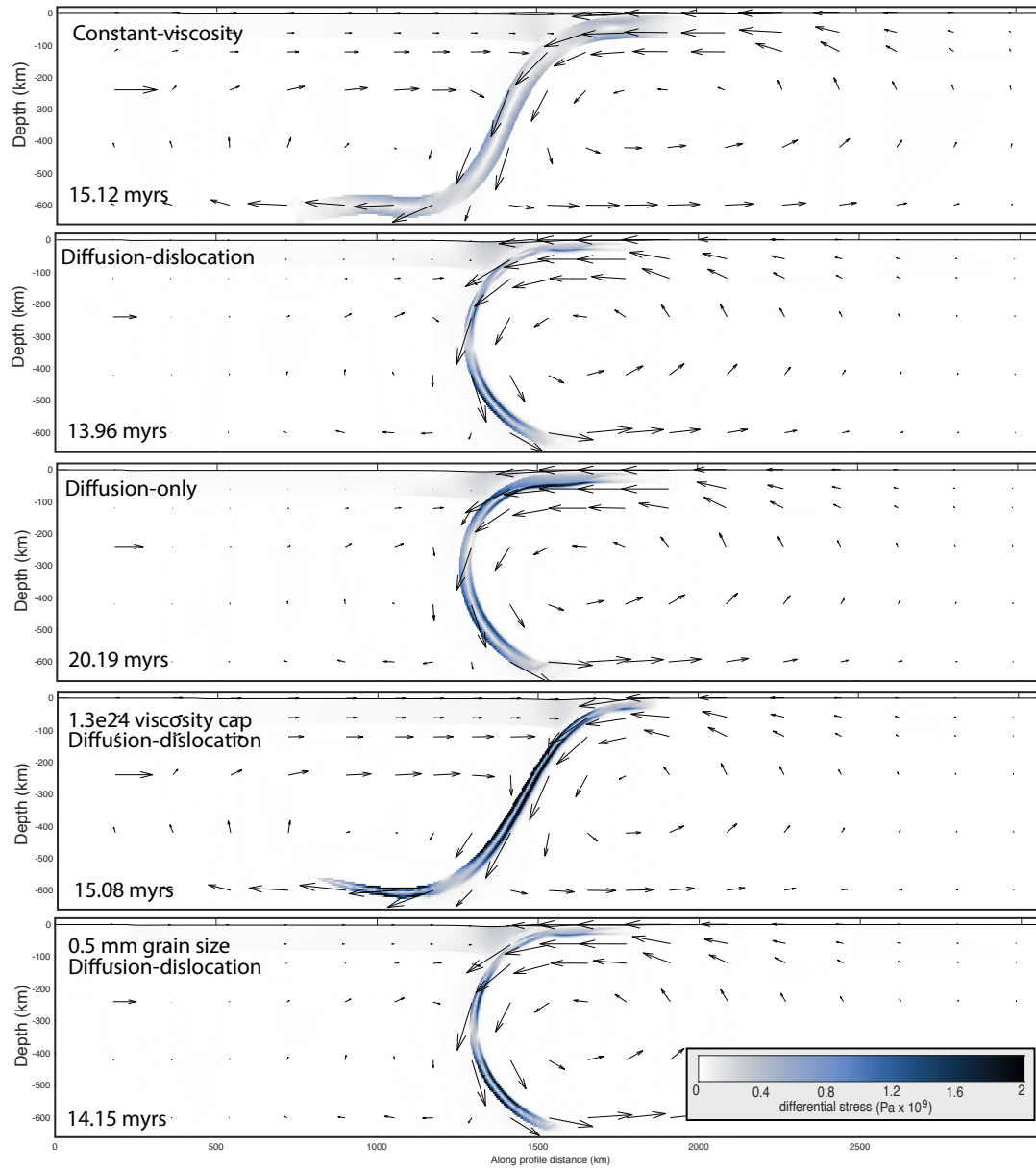
Figure A1. Images of the models for which we calculated bending resistance, colored by differential stress. Times on the lower left corner of each plot indicate at what elapsed time the measurements were taken.
