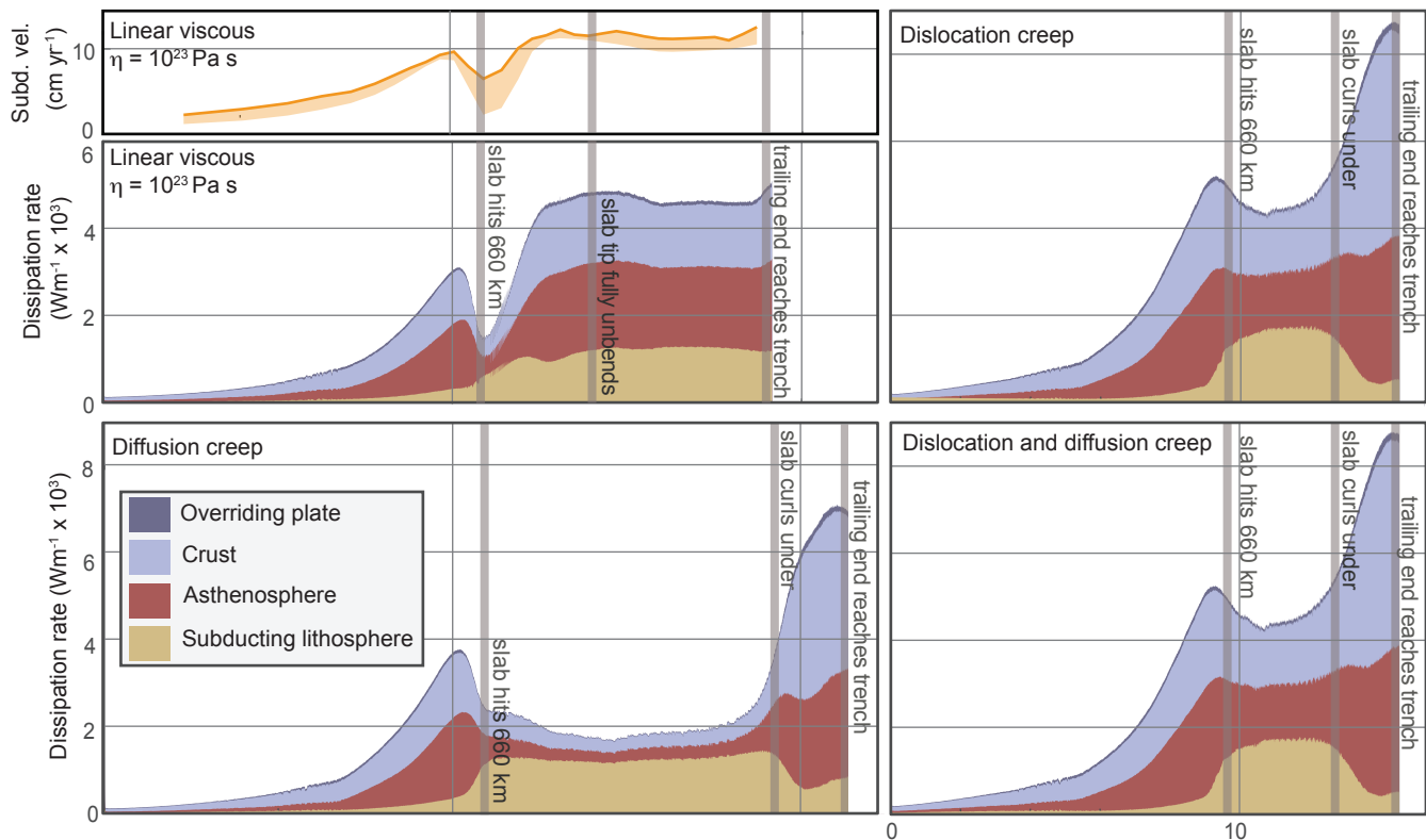
Figure 6. Dissipation of energy over time in each model. Each curve is broken down into dissipation in the crust, mantle lithosphere, asthenosphere, and the overriding plate. The plot on the upper left shows subduction velocity for the reference model to illustrate the correlation with the total rate of energy dissipation shown in the plot below. Vertical grey bars mark notable points in the evolution of each experiment.
