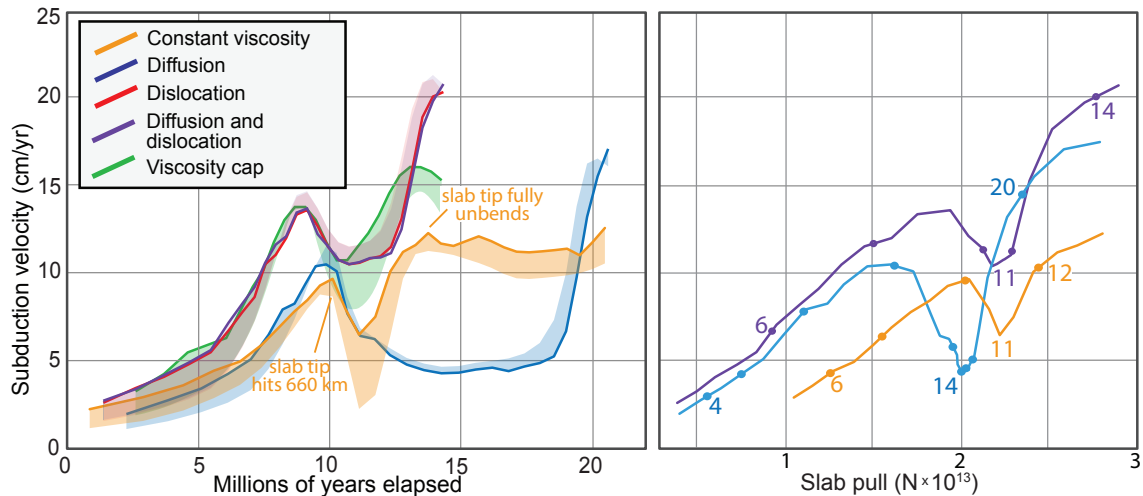
Figure 4. The plot on the left shows subduction velocity over time for the constant-viscosity reference slab and four creep-governed slabs. The bold curves show the rate at which material is consumed at the trench and the opposite edge of the shaded region around each curve shows the rate of motion of the slab with respect to the model boundaries. The thickness of the shaded region therefore represents the velocity of the trench. During periods where the shaded region lies below the bold line, the model undergoes slab rollback. Where the shaded region lies above the line, there is trench advance. The plot on the right shows how subduction velocity varies with slab pull in the constant-viscosity, diffusion, and diffusion-dislocation models. The lines follow the progression of each model through time with points at 2 million year intervals. Data are only plotted until the slab begins to lie flat on the bottom of the model. Beyond this point, slab pull is no longer proportional to the density anomaly of the subducted slab, and the calculation of slab pull is less straightforward.
