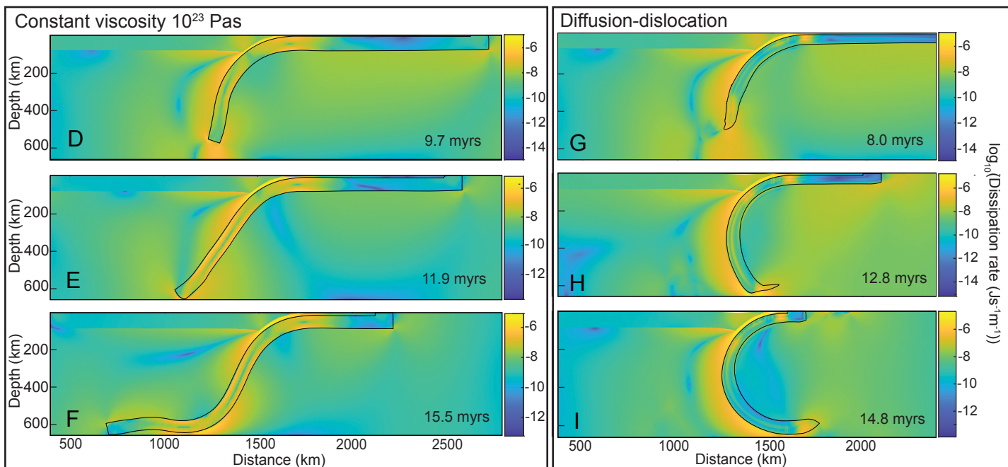
Figure 7. Dissipation rate in the crust (A), sub-lithospheric mantle (B), and slab mantle lithosphere (C) plotted against subduction velocity. The lines trace out the progression of each model over time, with selected points in time indicated in millions of years. Panels D-F show the distribution of energy dissipation in the reference model at 3 key snapshots. Panels G-I show distribution of energy dissipation for similar stages in the parallel diffusion-dislocation model. Plots are colored according to \log_{10} of dissipation rate in \text{J s}^{-1} \text{m}^{-1} . In each panel, the portion of the slab that exceeds the viscosity of the asthenosphere is outlined in black.
