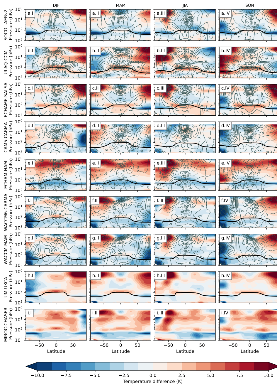
Figure A3. The difference of the time-slice simulations, averaged over 20 years for each season for temperature and zonal winds. Anomalies are calculated with respect to 1999-2004 ERA-I data, which was regridded to the respective model grid. Temperature is shown in color, while winds are in gray contours. Solid lines indicate stronger than observed westerly zonal winds, while dashed lines are weaker than observed. The numbers along with the contours are the anomalies in \text{ms}^{-1} . Each column represents one season, while each row represents one model. The simulated tropopause is shown as a black line, also averaged over each season respectively.
