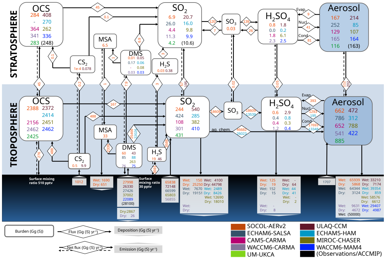
Figure 1. The atmospheric sulfur cycle with burdens (in Gg(S)) and fluxes ( \text{Gg(S)yr}^{-1} ) for S-gases and sulfate aerosols (displayed in analogy to Feinberg et al. (2019) and Sheng et al. (2015)). The term "Aerosol" refers only to sulfate aerosol. The figure includes all burdens as provided by the models involved. For CAM5-CARMA, WACCM6-CARMA, WACCM6-MAM, and UM-UKCA, stratospheric burdens are calculated from monthly mean volume or mass mixing ratios, integrated from the model tropopause upward because these burden values were not provided. Burdens and fluxes are averaged over the entire period. We use SAGE-3 \lambda for aerosol and MIPAS for SO 2 , DMS emission from Lana et al. (2011), which are all observation-derived. Additionally, we show the aerosol wet depositions from a multi-model mean from the Atmospheric Chemistry and Climate Model Intercomparison Project (ACCMIP) (Lamarque et al., 2013), as previously used in Feinberg et al. (2019). These observation-derived data and the ACCMIP value are in parentheses. Most fluxes are given as one-way fluxes, while cross-tropopause transport, as well as OCS and H 2 S emissions are provided as net fluxes. Fluxes are only available for one or two models at a time (SOCOL-AERv2 and ULAQ-CCM or SOCOL-AERv2 and ECHAM5-HAM). Emissions of OCS and H 2 S were prescribed as mixing ratios in the surface layer, in some models. In that case, emission and deposition net fluxes for both species are derived by balancing the sum of the other fluxes of all species.
