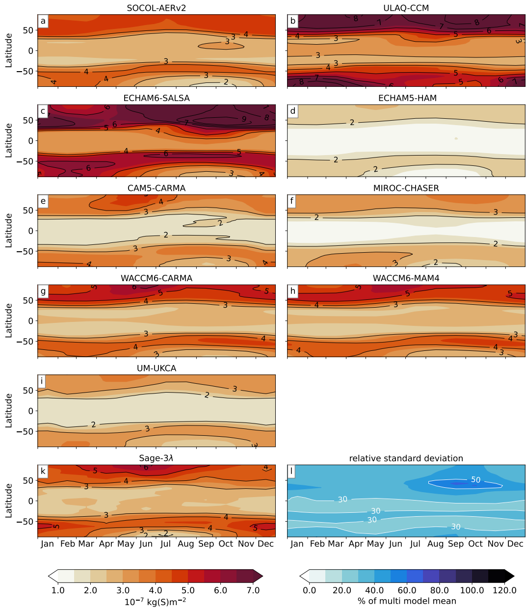
Figure 5. The stratospheric aerosol column in \text{kg m}^{-2}\text{m}^{-2} , averaged for each month over the 20 years of simulation, 10 years for ULAQ-CCM, and six years for SAGE-3λ. (a-i) Each represent one model for all latitudes over time. (k) is the SAGE-3λ dataset. (l) shows the RSD of all models (not including SAGE-3λ). All data were gridded to a 5^\circ \times 5^\circ grid to calculate the RSD.
