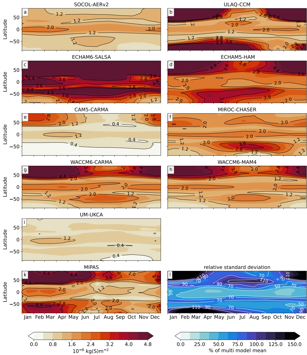
Figure 8. The stratospheric SO 2 burden in \text{kg m}^{-2} \text{kg(S)m}^{-2} for all models in (a-i), MIPAS in (k), and the multi-model RSD in (l). See also Fig. 5.
