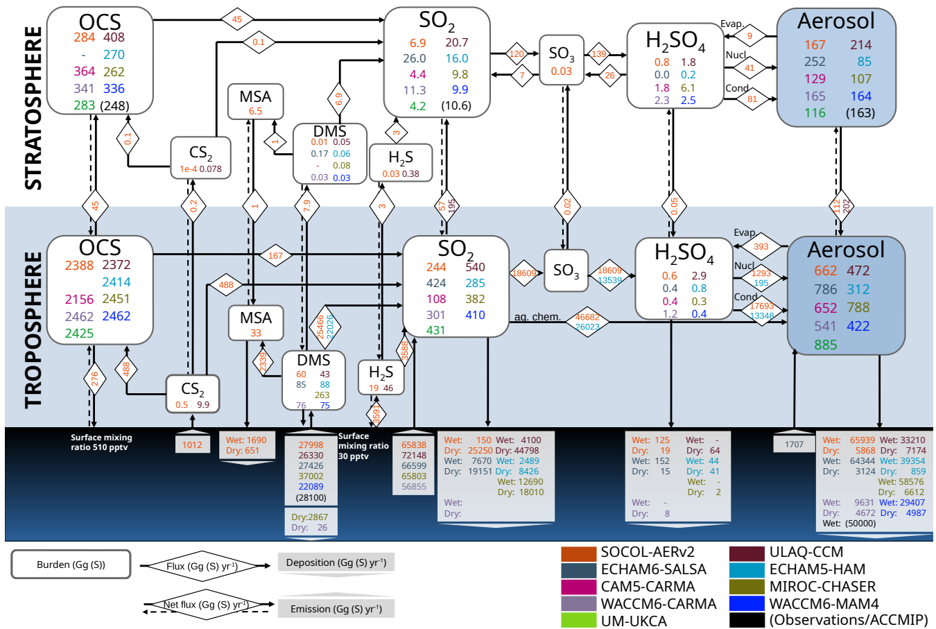
Figure 1. The atmospheric sulfur cycle with burdens (in \text{Gg}(\text{S})\text{Gg}(\text{S}) ) and fluxes ( \text{Gg}(\text{S})\text{Gg}(\text{S})\text{yr}^{-1} \text{yr}^{-1} ) for S-gases and sulfate aerosols (displayed in analogy to Feinberg et al. (2019) and Sheng et al. (2015)). Note that the The term "Aerosol" refers only to sulfate aerosol. The figure includes all burdens as provided by the models involved. For CAM5-CARMA, WACCM6-CARMA, WACCM6-MAM, and UM-UKCA, stratospheric burdens are calculated from monthly mean volume or mass mixing ratios, integrated from the model tropopause upward because these burden values were not provided. Burdens and fluxes are averaged over the entire period. Observation-derived data, and a multi-model mean from ACCMIP are in brackets. We use SAGE-3 \lambda for aerosol and MIPAS for SO 2 , DMS emission from Lana et al. (2011), and which are all observation-derived. Additionally, we show the aerosol wet depositions from a multi-model mean from the Atmospheric Chemistry and Climate Model Intercomparison Project (ACCMIPmodels) (Lamarque et al., 2013), as previously used in Feinberg et al. (2019). These observation-derived data and the ACCMIP value are in parentheses. Most fluxes are given as one-way fluxes, while cross-tropopause transport, as well as OCS and H 2 S emissions are provided as net fluxes. Note that fluxes Fluxes are only available for one or two models at a time (SOCOL-AERv2 and ULAQ-CCM or SOCOL-AERv2 and ECHAM5-HAM). Emissions of OCS and H 2 S were prescribed as mixing ratios in the surface layer, in some models. In that case, emission and deposition net fluxes for both species are derived by balancing the sum of the other fluxes of all species.
