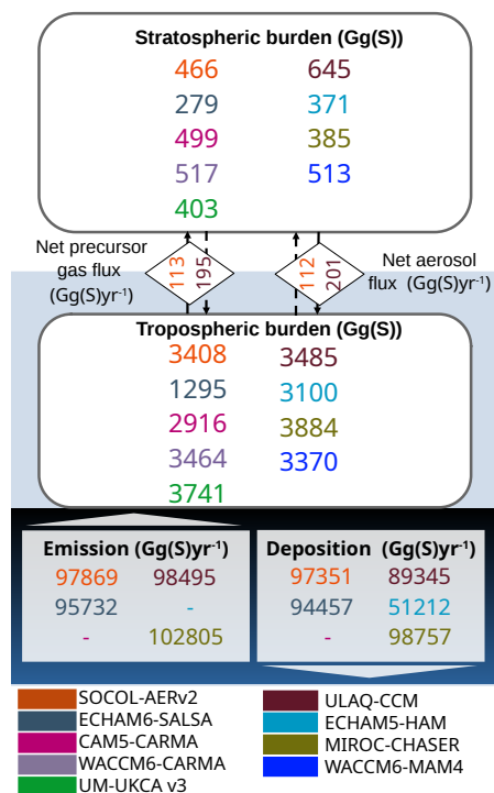
Figure 2. The total sulfur balance for each model. All sulfur species are summed up for each model and depicted here in Gg(S). Cross tropopause fluxes (in Gg(S)yr -1 ) are net fluxes of aerosol precursor gases (net upward) plus the net aerosol flux (net downward), which were only provided by SOCOL-AERv2 and ULAQ-CCM. Note that the burden for ECHAM6-SALSA is lower, as the model does not include OCS. Therefore this model is excluded from the calculation of the model spread for the total sulfur burden.
