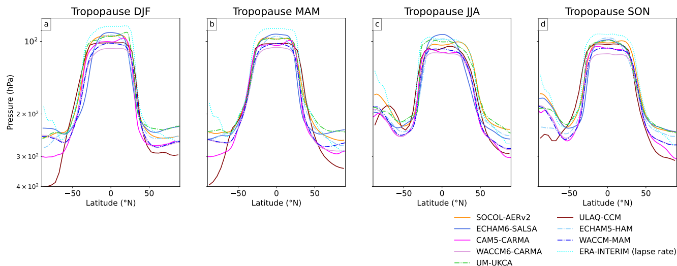
Figure A5. The tropopauses of each model as well as the ERA-INTERIM-ERA-I derived tropopause which was used to calculate stratospheric burdens for SAGE-3λ.
