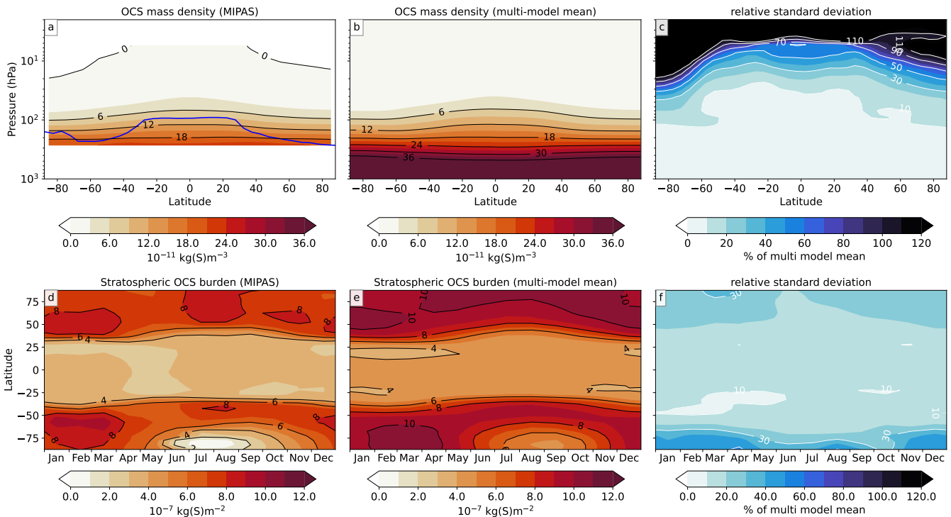
Figure 6. The OCS mass density in \text{kg(S)}\text{m}^{-3} is shown in the top row (a-c) as a multi-model mean of all models which include. The bottom row depicts the zonally averaged stratospheric OCS burden in \text{kg(S)}\text{m}^{-2} (d-f). Panels (a) and (d) show the MIPAS dataset, (b) and (e) are the multi-model means and (c) and (f) is the RSD. All model data were interpolated onto the same grid and vertical coordinates. The RSD is shown in (b). Panel (e) depicts the multi-model mean of the stratospheric OCS burden in \text{kg(S)}\text{m}^{-2} . The RSD for the stratospheric burden is shown in panel (d). The data were calculated from volume mixing ratios of OCS, using the ideal gas law and provided temperature and pressure fields. ECHAM6-SALSA does not track OCS and is therefore not included here.
