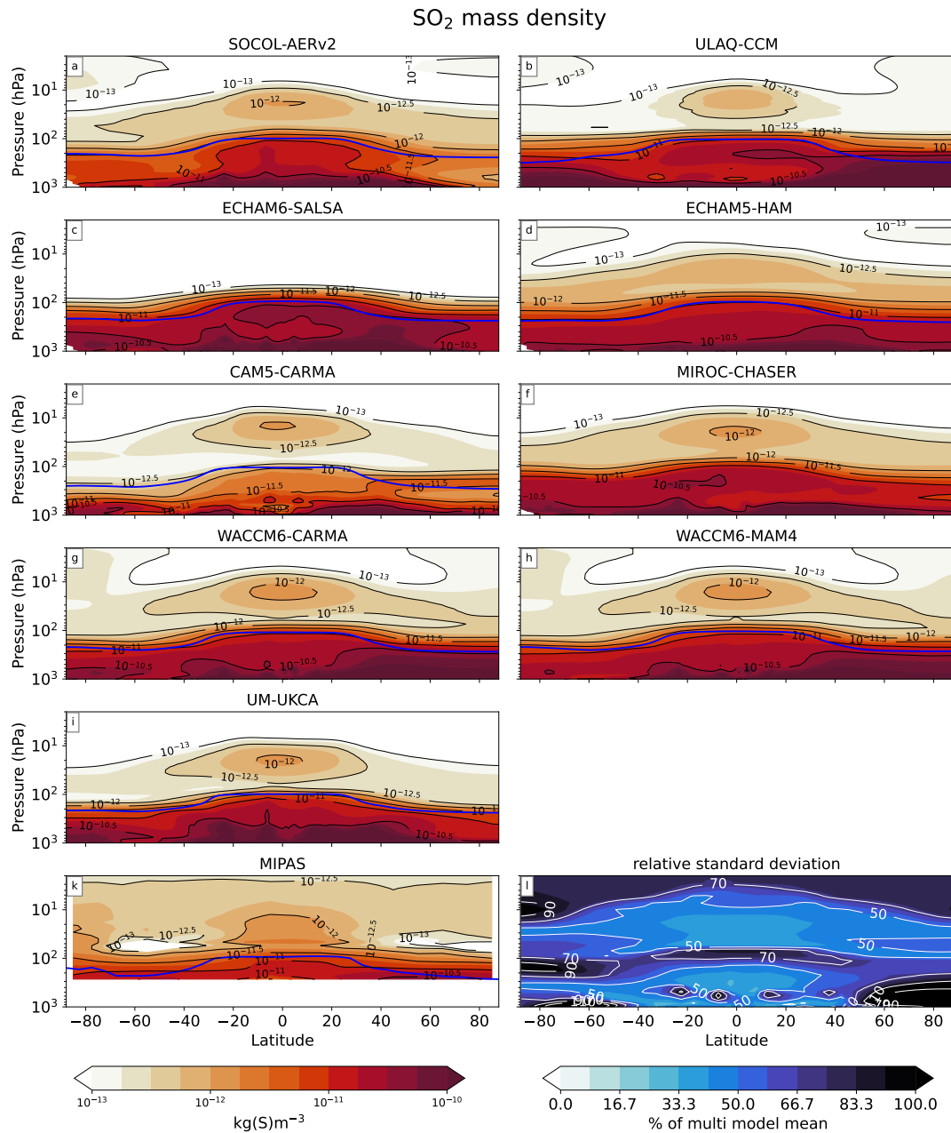
Figure 7. The stratospheric SO 2 burden in \text{kg m}^{-3} on a logarithmic color scale. The models are depicted in (a-i), while the MIPAS-derived dataset is shown in (k). The RSD in (l) is obtained from the multi-model ensemble. The tropopause is shown as a blue line and was averaged over the simulated time period and all longitudes. The mass density was obtained from volume mixing ratios, using the model temperature and pressure applied to the ideal gas law.
