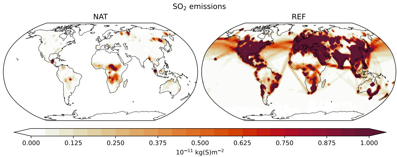
Figure A1. The SO 2 emissions from the MACC-CITY inventory for the NAT experiments without anthropogenic emissions on the left, and the REF experiment with anthropogenic emissions on the right. Continuously outgassing volcanic emissions are included in both simulations.
