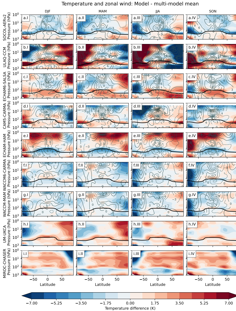
Figure A3. Depicted is the difference of the time-slice simulations, averaged over 20 years for each season for temperature and zonal winds. All data were gridded to a 5^\circ \times 5^\circ \times 5^\circ grid and to 39 pressure levels. Anomalies are calculated with respect to the multimodel mean. Temperature is shown in color, while winds are in gray contours. Solid lines indicate stronger than observed westerly zonal winds, while dashed lines are weaker than observed. The numbers along with the contours are the anomalies in \text{m s}^{-1} . Each column represents one season, while each row represents one model. The simulated tropopause is shown as a black line, also averaged over each season respectively.
