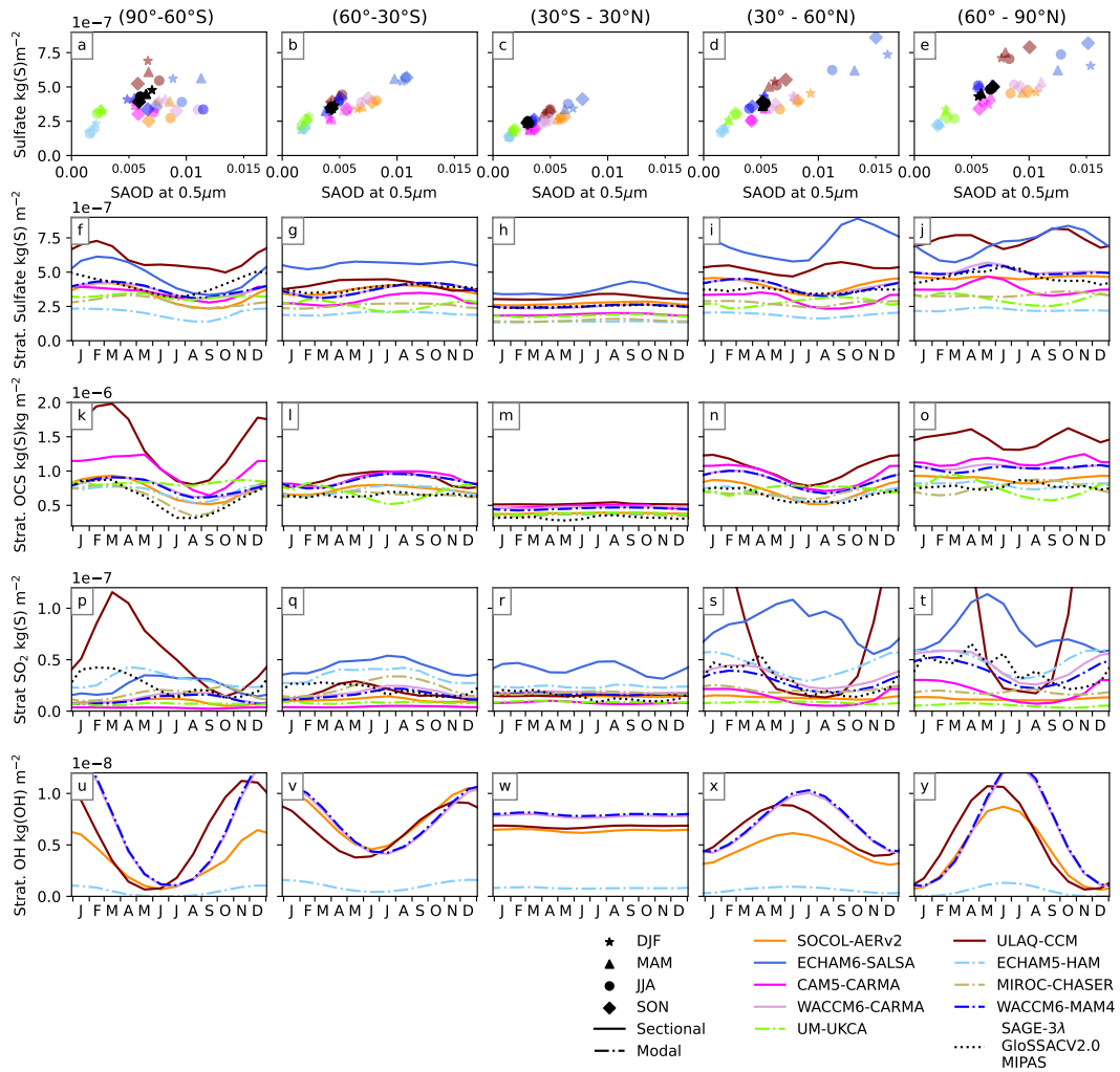
Figure 3. The seasonal cycle of the three most abundant atmospheric sulfur species (sulfate aerosol, \text{SO}_2 , and OCS), as well as OH ( OH was only reported by five models ). All data were zonally averaged over the latitude band given in each column title. Additionally, (a-e) represent the relationship between the SAOD at 0.5\mu\text{m} and the sulfate burden for five latitude bins. Each season is depicted by a character: A star for winter, a triangle for spring, a circle for summer, and a diamond for autumn. (f-j) depict the seasonal cycle of the stratospheric aerosol burden for each of these latitude bins. In (k-o), we see the stratospheric OCS burden, while (p-t) show the stratospheric \text{SO}_2 burden and (u-y) the stratospheric OH burden respectively. Each burden is given in \text{kg(S)}\text{m}^{-2} except for OH, which is given as \text{kg(OH)}\text{m}^{-2} . All data have been averaged over the 20 simulated years for each month. Not shown in the figure are the maximum values of the stratospheric \text{SO}_2 burden in ULAQ-CCM and the stratospheric OH burden in both WACCM6 models. ULAQ-CCM \text{SO}_2 burdens in the northern mid-latitudes peak in January at 1.9 \times 10^{-7} \text{ kg(S)}\text{m}^{-2} or 5.5 \times 10^{-7} \text{ kg(S)}\text{m}^{-2} in the northern polar region. Maximum OH burdens in WACCM6-CARMA and WACCM6-MAM4 in both the NH (July) and SH (December) amount to 1.3 \times 10^{-8} \text{ kg(OH)}\text{m}^{-2} .
