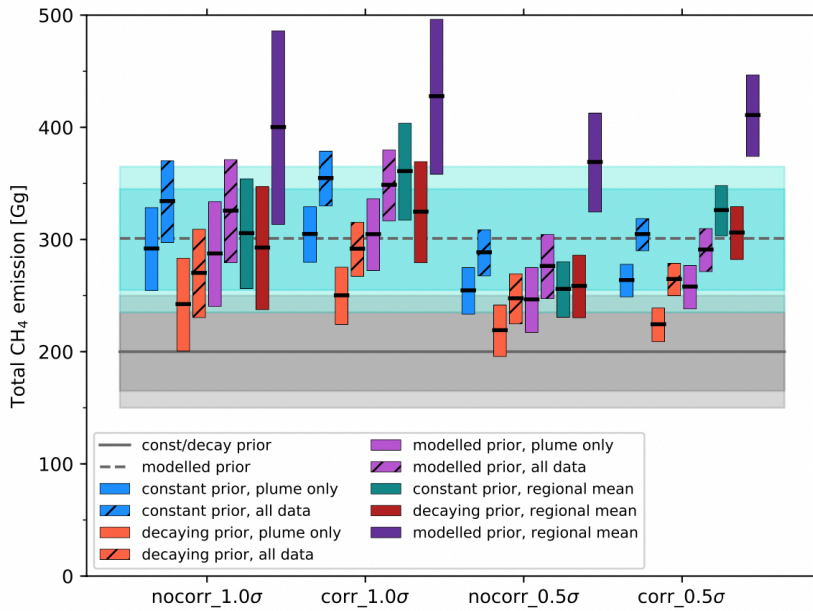
950 Figure 7: Total (two-day) posterior CH 4 emissions (Gg) from the Nord Stream leaks during 26 th – 27 th September 955 based on multiple different IASI-based inverse modelling calculations. Boxes represent the 1σ uncertainty on each inversion, with each thick horizontal black line representing the mean. Blue boxes represent inversions with the constant prior where the model is optimised against individual IASI retrievals, whilst orange boxes are the same but for the decaying prior and pink are for the modelled prior. Teal boxes represent inversions with the constant prior where the model is optimised against the mean XCH 4 in the plume region, whereas red boxes are the same but for the decaying prior and purple for the modelled prior. Hatched boxes show inversions in which all IASI data is included, and unhatched boxes show inversions in which retrievals only within the plume region are included. ‘Corr’ and ‘nocorr’ refers to inversions with and without prior temporal correlations included, whilst 1σ and 0.5σ refer to inversions with 100% and 50% prior uncertainty. The grey solid line shows the prior emission total for the constant and decaying priors , with 50% and 100% 3-hour prior uncertainty shaded in dark and light grey, respectively. The grey dashed line shows the modelled prior emission, with 50% and 100% 3-hour prior uncertainty shaded in dark and light turquoise, respectively.
