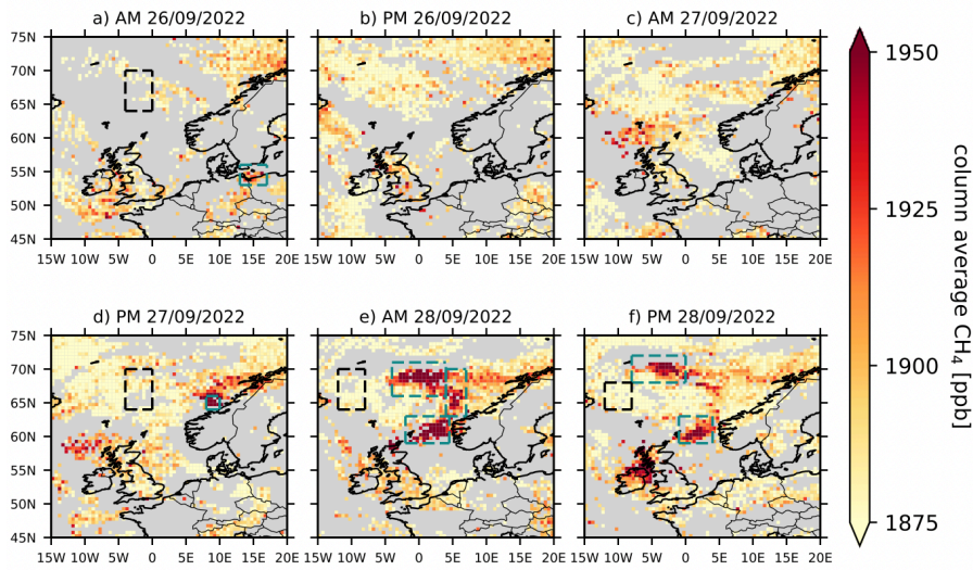
900 Figure 2: IASI column average CH 4 (ppb) for 26th - 28th September 2022. Retrievals are averaged onto 0.25° × 0.25° grid boxes, weighted inversely to their uncertainties for the morning and evening overpasses of each day. Black dashed boxes show 'background' regions used in the integrated mass enhancement (IME) method, whilst turquoise dashed boxes show 'enhancement' regions. Grey regions are obscured by cloud.
