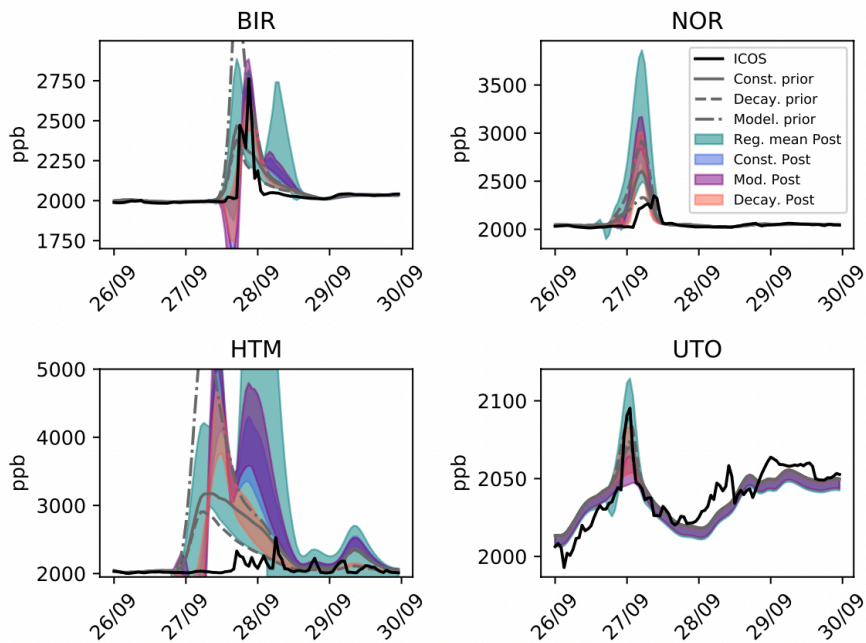
905 Figure 3: Observed (black line) and simulated (grey lines/coloured shading) CH 4 mixing ratios (ppb) at Integrated Carbon Observation System (ICOS) sites during 26 th – 29 th September 2022. Observations and model output are both 910 averaged into hourly means. ICOS sites are at Birkenes, Norway (BIR), Norunda, Sweden (NOR), Hyltemossa, Sweden (HTM) and Utö, Finland (UTO). See main text and Figure 1 for further details. Grey lines show TOMCAT- simulated CH 4 using the three prior emission estimates, and shaded regions show the simulated min/max range for the inversions with constant prior (blue), decaying prior (red) and modelled prior (purple) optimised against individual retrievals, and for inversions optimised against the regional mean (teal). Inlet heights are the highest available at each site: 75m at BIR; 100m at NOR; 150m at HTM and 57m at UTO. Note the different y-axis ranges in each panel.
