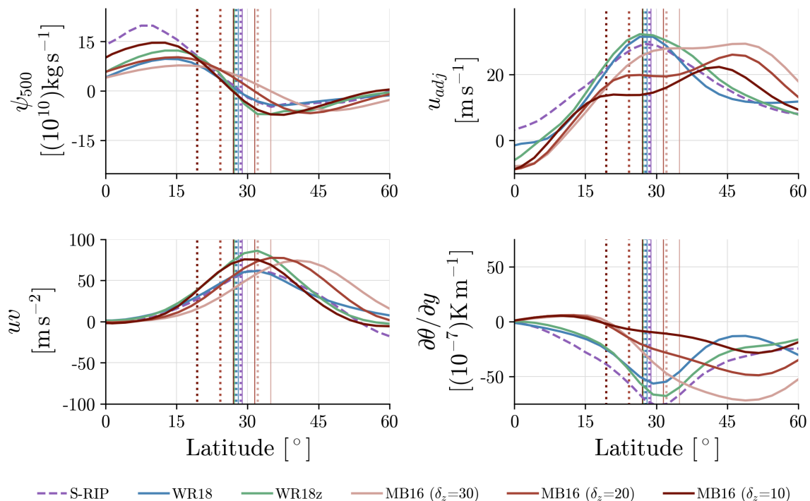
Figure 5. NH DJF meridional streamfunction at 500 hPa (top left), adjusted wind (top right), vertically averaged eddy momentum flux between 200-400 hPa (bottom left), and vertically averaged meridional temperature gradient between 100-400 hPa (bottom right) for S-RIP, WR18, WR18z, MB16 (default, \delta_z = 10 ), MB16 ( \delta_z = 20 ), and MB16 ( \delta_z = 30 ). The dotted and solid thin vertical lines show the climatological \phi_{STJ} and climatological \phi_{HC} , respectively, for each corresponding simulation.
