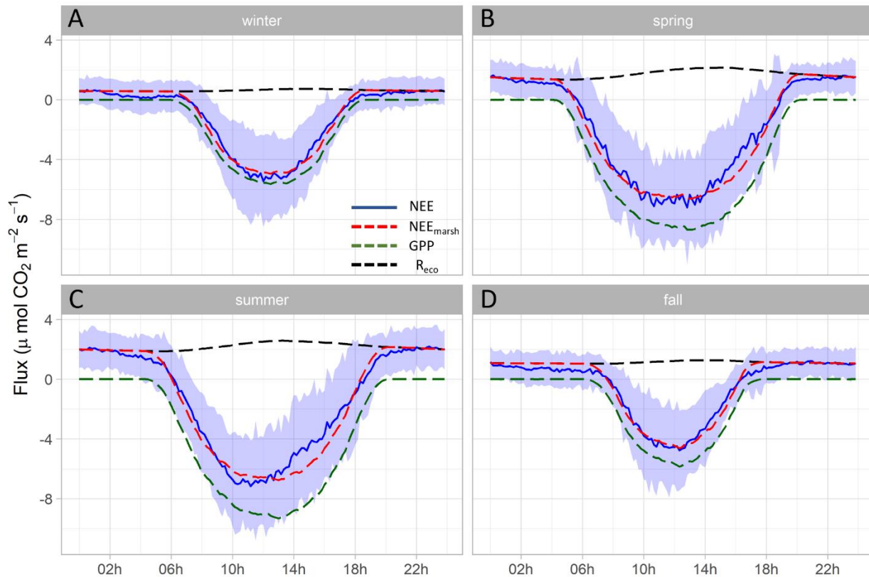
415 Figure 5: Hourly plots of the measured NEE, estimated NEE_{\text{marsh}} , estimated GPP and estimated R_{\text{eco}} diurnal variations obtained every 10 minutes in winter (A), spring (B), summer (C) and fall (D) over the year 2020. NEE averages are represented by blue solid lines whereas standard deviations are represented by blue areas; the NEE_{\text{marsh}} , GPP and R_{\text{eco}} averages are represented by red, green and black dotted lines, respectively. The NEE fluxes were partitioned into GPP and R_{\text{eco}} according to Kowalski et al. (2003) using monthly coefficients (see the M&M section). Night-time periods correspond to GPP = 0 \mu\text{mol m}^{-2} \text{s}^{-1} and NEE_{\text{marsh}} = R_{\text{eco}} . All values are in \mu\text{mol CO}_2 \text{m}^{-2} \text{s}^{-1} . 420
