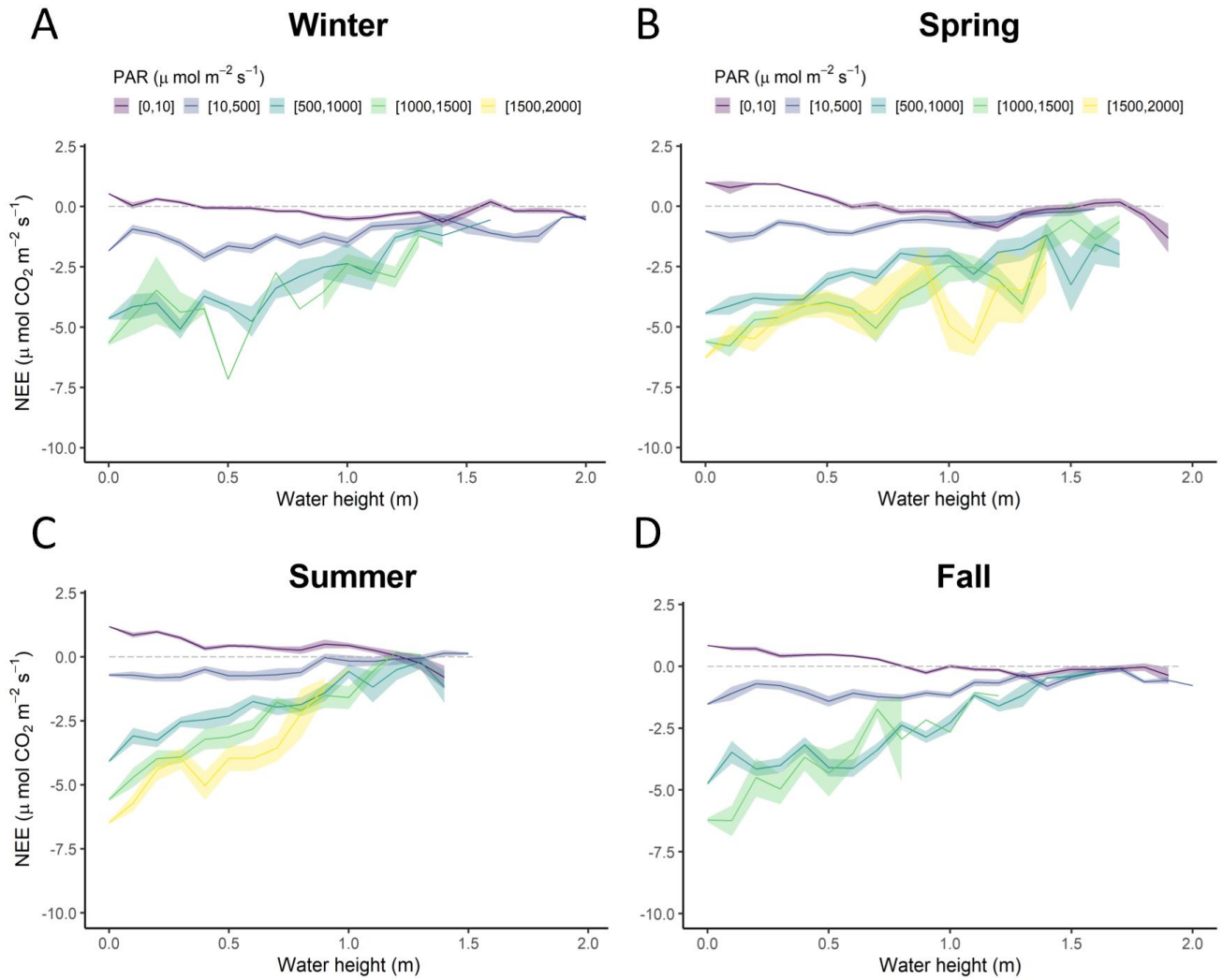
Figure 8: Diurnal variations of NEE ( \mu\text{mol CO}_2 \text{ m}^{-2} \text{ s}^{-1} ) obtained every 10 minutes according to water height (Hw, m) within five PAR groups (see captions in Fig. 6) in winter (A), spring (B), summer (C) and fall (D). NEE values were averaged every 0.1 m. The coloured areas represent the standard error of the mean.
