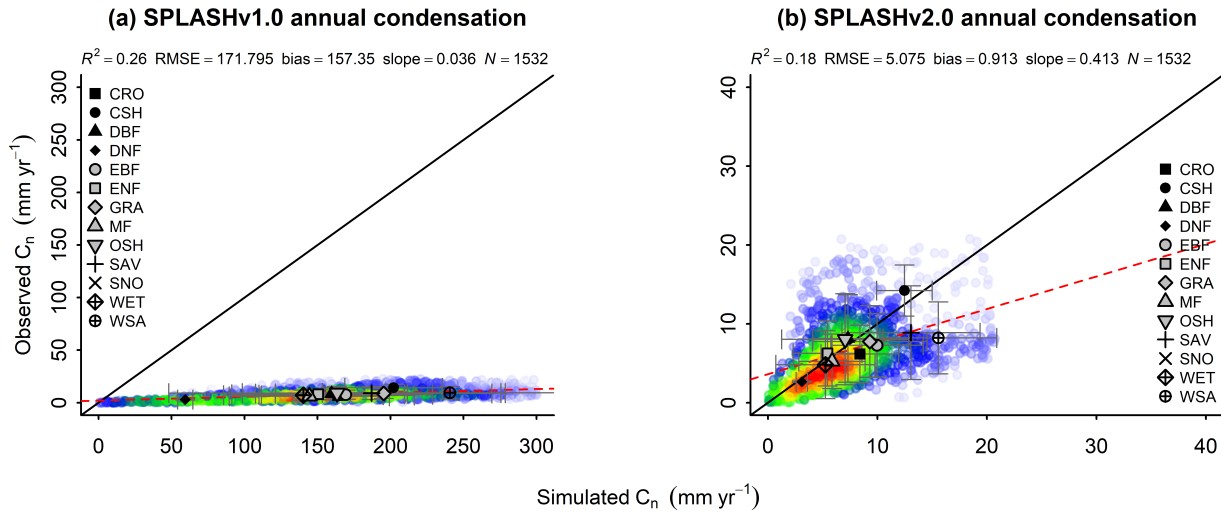
Figure 28. Correlation of observed and simulated values of C_n with data from all the sites pooled. The color scale shows point density; red indicates higher density. (a) simulations with SPLASH v1.0. (b) simulations with SPLASH v2.0.
