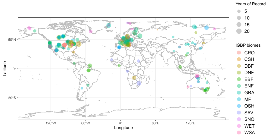
Figure 8. FLUXNET stations used for the I_{LW} parameter calibration.
