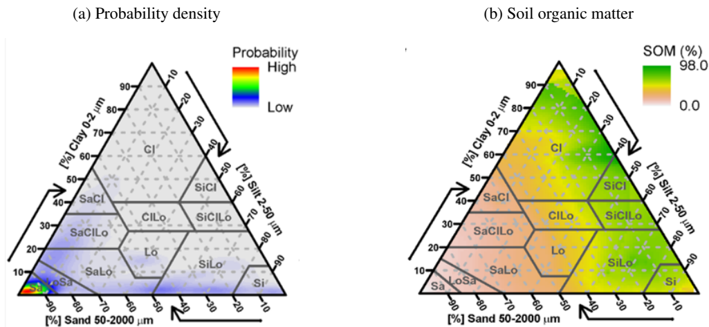
Figure 14. K_{sat} and \theta_{sat} measurements used to calibrate the pedotransfer functions. (a) Probability density of the samples according to their textural classes. (b) Average soil organic matter content of the samples per textural class.
