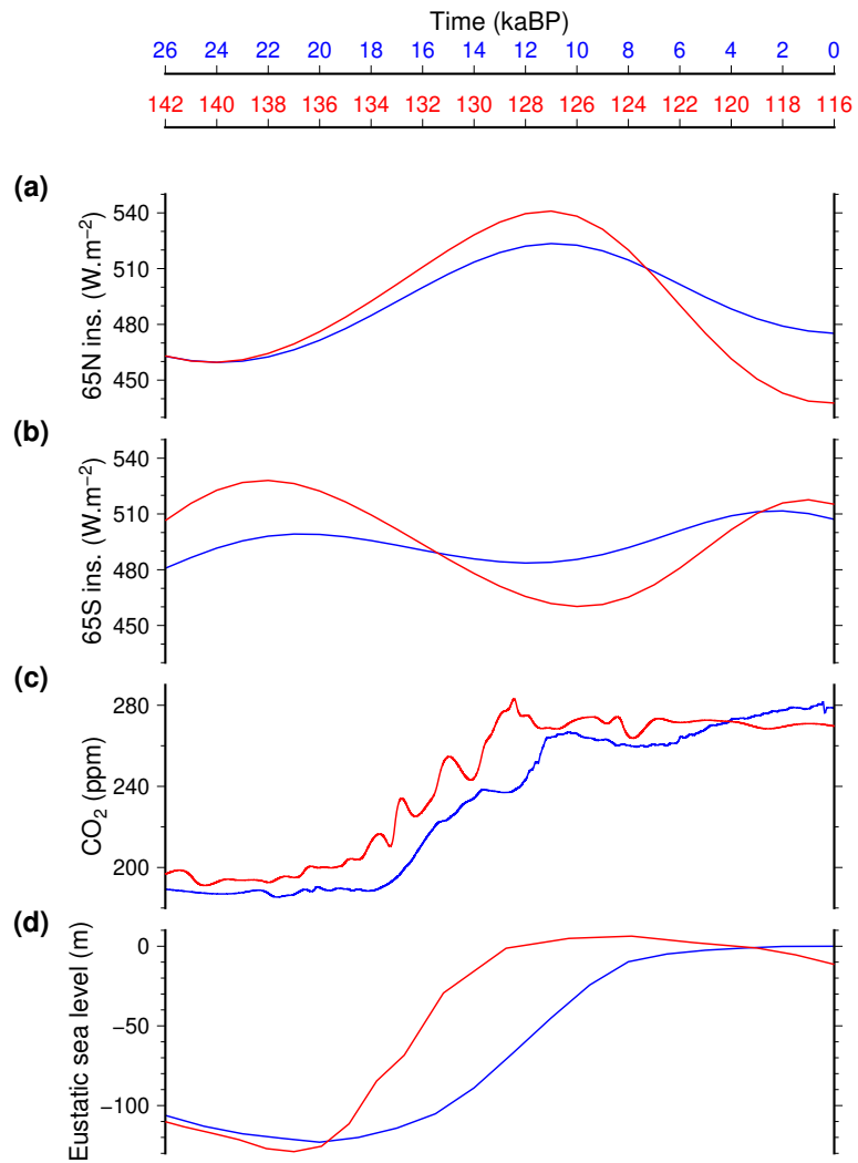
Figure 1. Temporal evolution of the major forcings over TII (red) and TI (blue). (a): June mean insolation at 65°N and (b): december mean insolation at 65°S (Berger, 1978). (c): carbon dioxide mixing ratio (Lüthi et al., 2008). (d): eustatic sea level (Waelbroeck et al., 2002).
