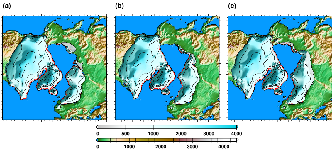
Figure 12. Initial ice sheet topographies for the the sensitivity experiments. (a): Reference ice sheet. (b): Slightly reduced North American ice sheet (-8 % in ice volume) and larger Eurasian ice sheet (+36 %). (c): Slightly reduced North American ice sheet (-6 %) and much larger Eurasian ice sheet (+71 %).
