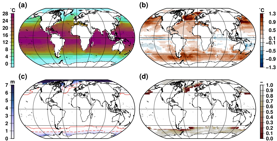
Figure 3. Sea surface temperature and sea ice thickness for glacial initial conditions. (a): climatological annual mean sea surface temperature computed at 26 kaBP . (b): 142 kaBP temperature difference with respect to 26 kaBP . (c): climatological annual mean sea ice thickness at 26 kaBP . The continuous red line stands for the maximal sea ice extent at 26 kaBP and the dashed line stands for a mean annual thickness of 0.5 cm at 26 kaBP . (d): 142 kaBP thickness ratio relative to 26 kaBP .
