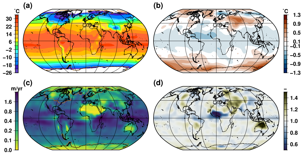
Figure 2. Temperature and precipitation for glacial initial conditions. (a): climatological annual mean near surface air temperature computed at 26 kaBP . (b): 142 kaBP temperature difference with respect to 26 kaBP . (c): climatological annual mean precipitation at 26 kaBP . (d): 142 kaBP precipitation ratio relative to 26 kaBP . The orange line is the extent of the ice sheets.
