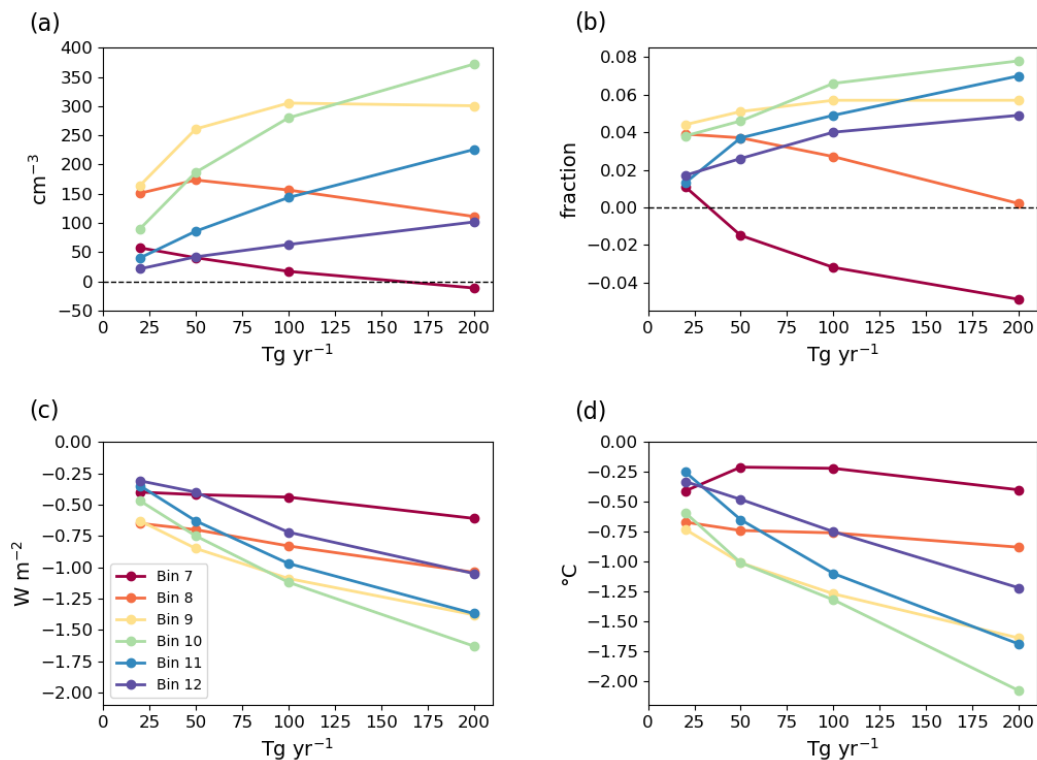
Figure 32: 10-year mean changes with respect to a non-perturbed control as a function of sea-salt injection rate in UKESM1 simulations using different sea-salt emission size bins: (a) cloud-top CDNC averaged over the four injection regions (cm -3 ), (b) cloud fraction averaged over the four injection regions, (c) global-mean ToA net radiation (W m -2 ), (d) global-mean near-surface air temperature (°C). The sizes of bins 7-12 are given in Table 1.
