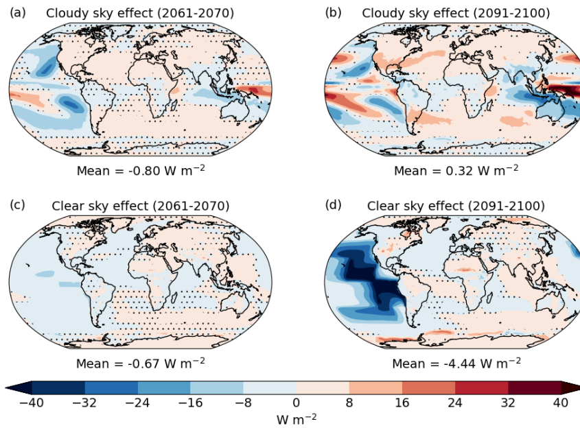
1045 Figure 65: The decades of maximum contribution from the cloudy- and clear-sky effects of MCB in terms of ToA net SW (G6MCB minus ssp245; \text{W m}^{-2} ): 2061-2070 is the decade of maximum cloudy-sky effect (panels (a) and (c): left column) and 2091-2100 the maximum for the clear-sky effect (panels (b) and (d): right column). Stippled areas show where the differences are not significant at the 5% level in a two-tailed t -test.
