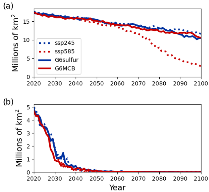
120 Figure 154: Arctic sea-ice area ( 10^6 \text{ km}^2 ) for (a) March, showing the maximum sea-ice extent, and for (b) September, showing the minimum extent.
