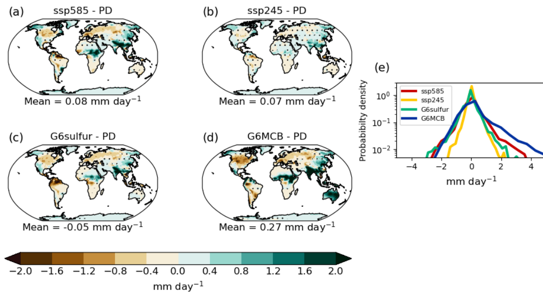
Figure 110: Same as Fig. 98 but for JJA land precipitation rate (mm day -1 ).
