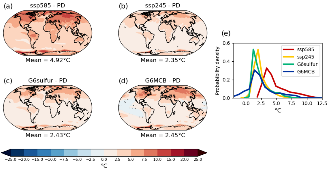
1070 Figure 98: Change in JJA near-surface air temperature (°C) for 2081-2100 compared with PD in (a) ssp585, (b) ssp245, (c) G6sulfur and (d) G6MCB. Stippled areas show where the differences are not significant at the 5% level in a two-tailed t -test. (e) Probability density function of the changes.
