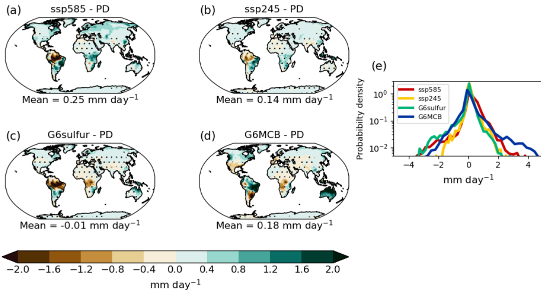
Figure 121: Same as Fig. 110 but for DJF.
