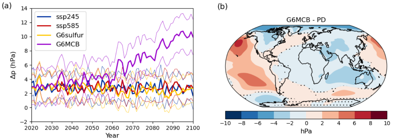
125 Figure 165: a) The SOI (hPa) derived as the simple difference in pressure between Tahiti and Darwin as a function of time for the simulations described in the text. The thick lines represent the ensemble mean and the thin lines the mean \pm two standard deviations. b) The spatial distribution of the change in the pressure pattern (hPa) determined for 2081-2100 for G6MCB compared with present day (PD).
