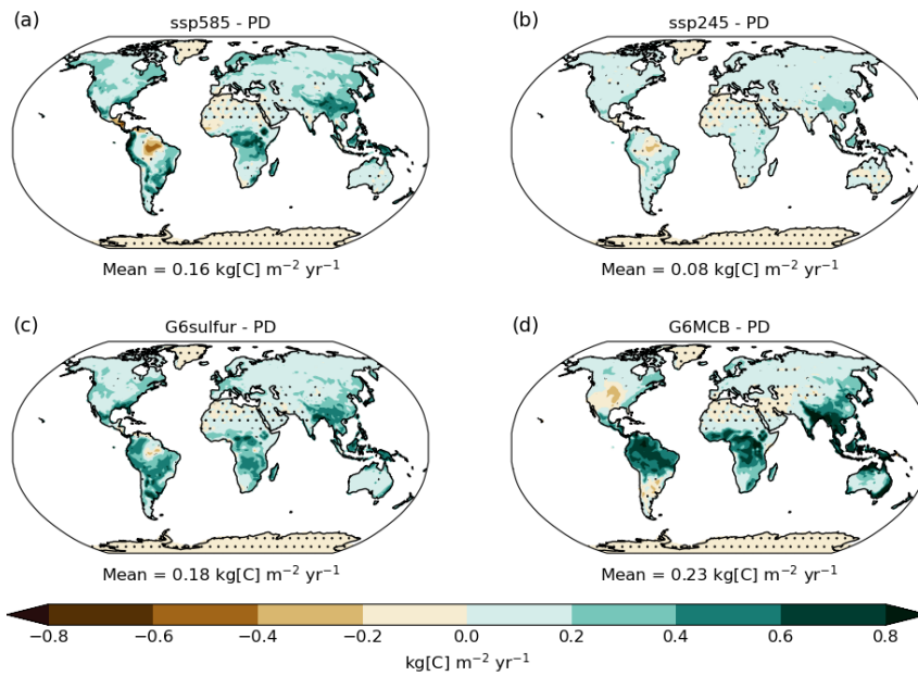
Figure 13.2: Change in annual-mean NPP (kg of carbon m -2 yr -1 ) for 2081-2100 compared with PD in (a) ssp585, (b) ssp245, (c) G6sulfur and (d) G6MCB. Stippled areas show where the differences are not significant at the 5% level in a two-tailed t -test.
