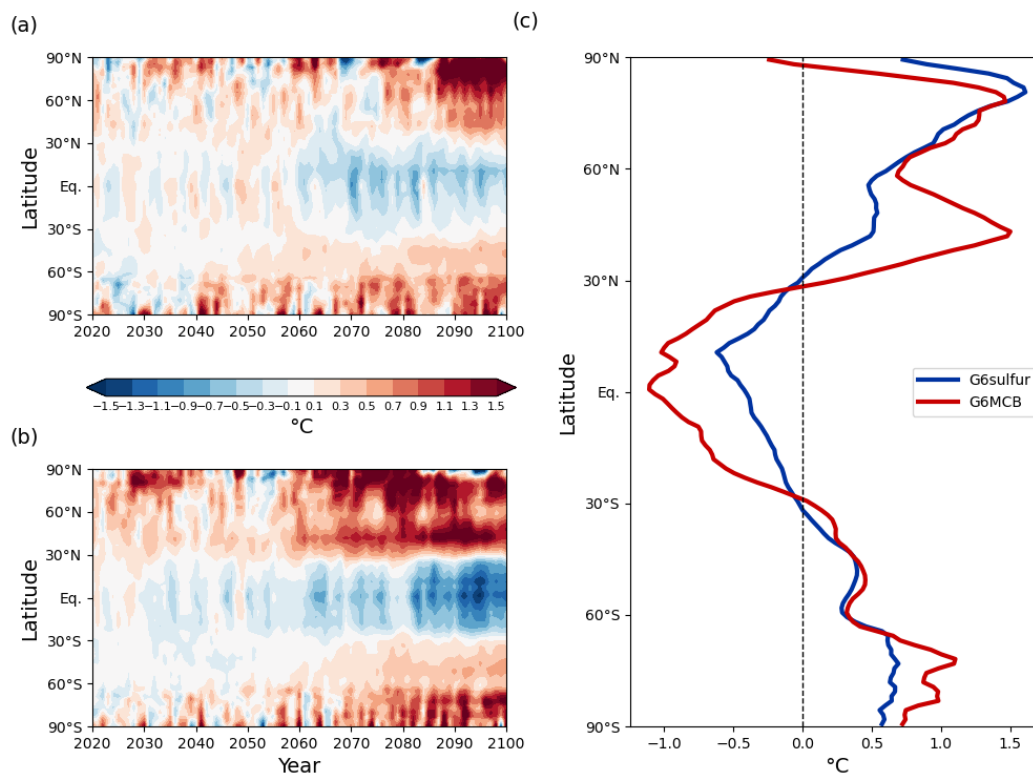
Figure 87: (a) Time-latitude evolution of the difference in near-surface air temperature ( ^{\circ}\text{C} ) between G6sulfur and ssp245. (b) The same as (a) but for the difference between G6MCB and ssp245. (c) Zonal means of the temperature differences for 2081-2100.
