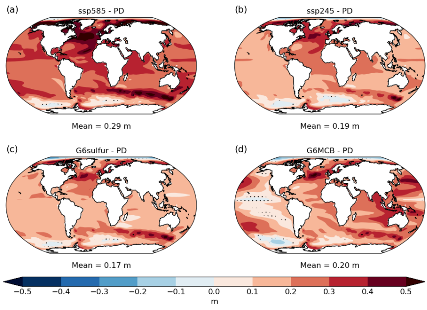
Figure 143: Change in sea-level for 2081-2100 compared with PD in (a) ssp585, (b) ssp245, (c) G6sulfur and (d) G6MCB. Stippled areas show where the differences are not significant at the 5% level in a two-tailed t -test.
