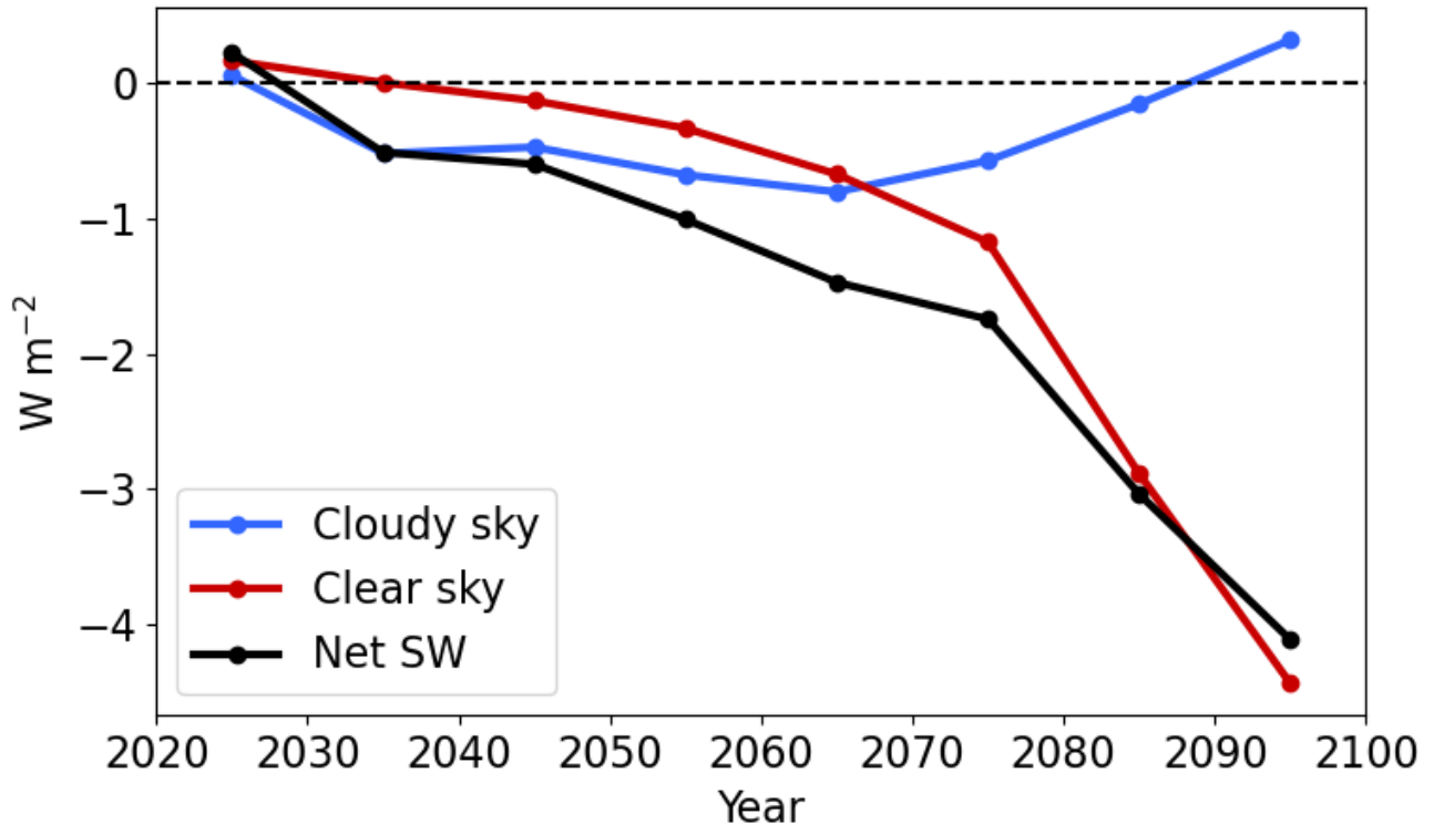
1040 Figure 54: Ensemble-mean estimates of the cloudy-sky, and clear-sky, and net solar contributions to the difference in decadal-mean ToA net downwards SW radiation between G6MCB and ssp245 (W m -2 ).
