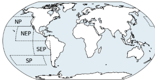
Figure 12: The regions used for sea-salt injection in G6MCB; only ocean points within each region were used.
