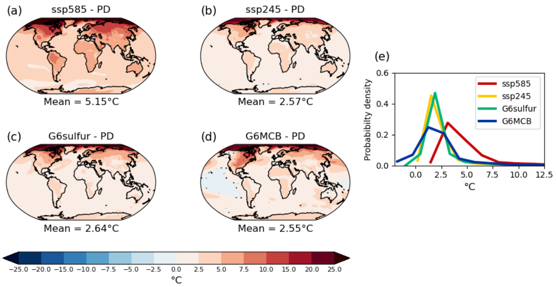
Figure 109: Same as Fig. 98 but for DJF.
