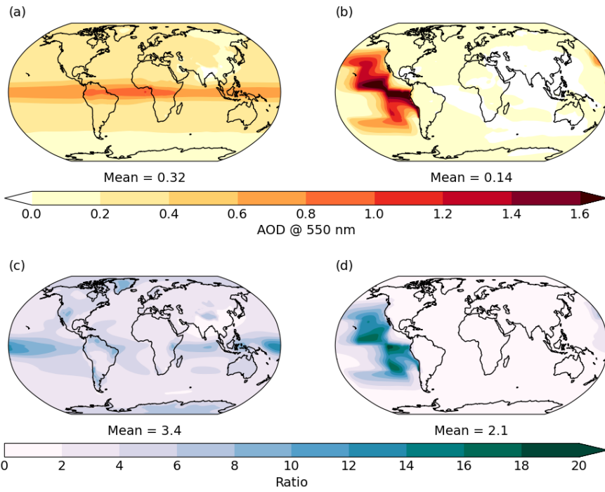
1055 | Figure 76: (a) The difference in AOD at 550 nm for 2081-2100 in G6sulfur compared with present-day. (b) Same as (a) but for G6MCB. (c) The ratio of AOD between G6sulfur (2081-2100) and PD. (d) Same as (c) but for G6MCB.
