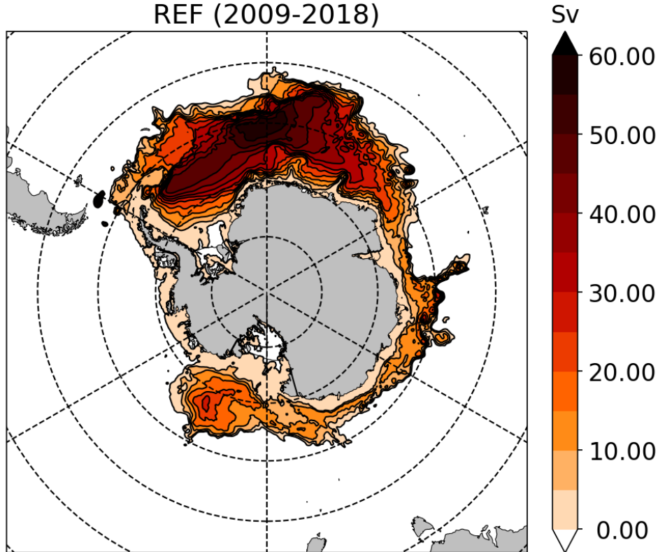
Figure 2. Climatological (2009-2018) barotropic stream function ( \Psi ) in REF (contours every 10 Sv). Areas beyond the polar gyres are in white. The zonal and meridional barotropic transports (Sv) between two locations are given by U = -\Delta_y \Psi and V = \Delta_x \Psi , i.e. by the signed differences in \Psi between these two points.
