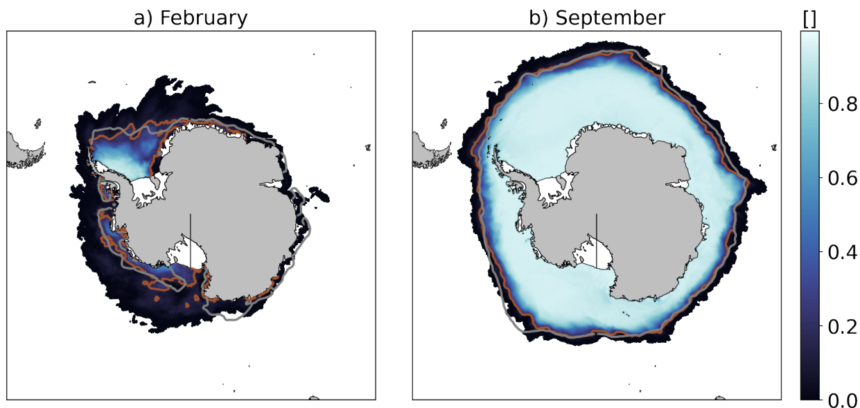
Figure 3. Climatological (2009-2018) sea ice concentration in REF in (a) February and (b) September. The grey lines indicate the sea ice extent in the satellite product of Meier et al. (2021), and the brown line shows the equivalent in our REF simulation.
