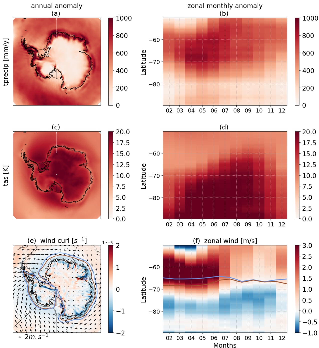
Figure 1. Maps of annual mean anomalies (left) and monthly-mean zonal-mean anomalies (right) for total precipitation (a,b), total precipitation and (c,d) near surface air temperature (e, d) near surface wind curl and wind anomalies (arrows) (f) near surface zonal wind . In (e,) and (f) The black, the blue line is the position of the zero zonal wind in the JRA reanalysis, and the green-brown line is the equivalent in for the perturbed forcing wind .
