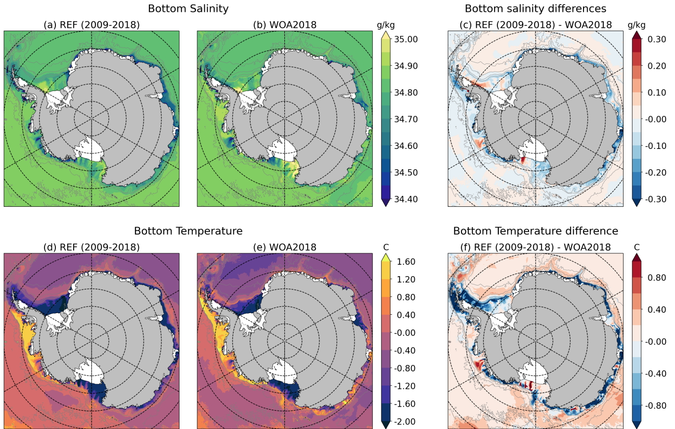
Figure 4. Upper panels: climatological bottom practical salinity in (a) REF and (b) WOA2018 (Locarnini et al., 2019; Zweng et al., 2019) and (c) the difference REF-WOA2018. Lower panels: climatological conservative temperature in (d) REF (e) WOA2018 and (f) the difference.
