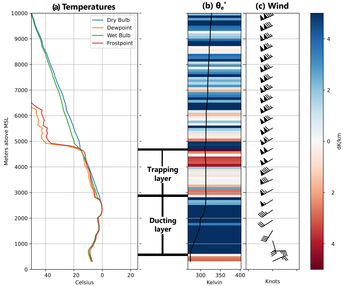
Figure 10. Upper air sounding data from Buffalo, NY, valid for 1200 UTC 25 Feb 2022. (a) Dry bulb temperature (blue), dew point (orange), wet bulb temperature (green), and frost point (red) profiles (all in °C). (b) Equivalent saturation potential temperature ( \theta_e^* ) profile (black line, K) overlaid on the vertical gradient in \theta_e^* ( K\ km^{-1} ). Positive values (blue) of the vertical gradient in \theta_e^* indicate absolute stability, while negative values (red) indicate conditional or absolute instability. (c) Horizontal wind profile (barbs, kts; colored according to wind speed). Annotation indicates the vertical extents of a ducting layer and a trapping layer according to the gravity wave duct criteria described by Lindzen and Tung (1976) and Koch and O’Handley (1997).
