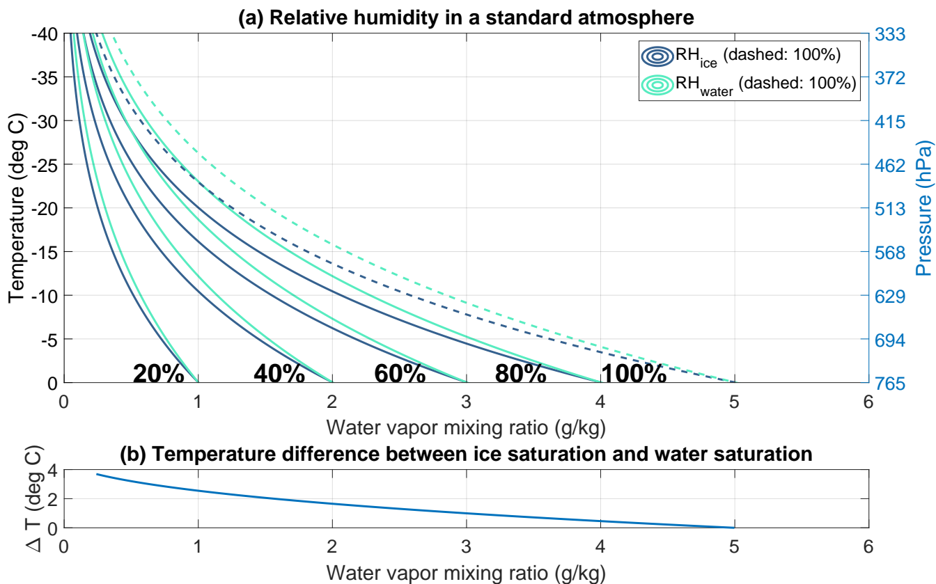
Figure 1. (a) Contours of relative humidity with respect to ice ( RH_{ice} ) and with respect to liquid water ( RH_{water} ) as a function of temperature and water vapor mixing ratio, assuming a standard atmosphere temperature-pressure relationship (corresponding pressure values on right axis). RH values are contoured at 20% intervals, with the 100% contour dashed. (b) The temperature difference between the 100% RH_{ice} and 100% RH_{water} contours for each water vapor mixing ratio.
