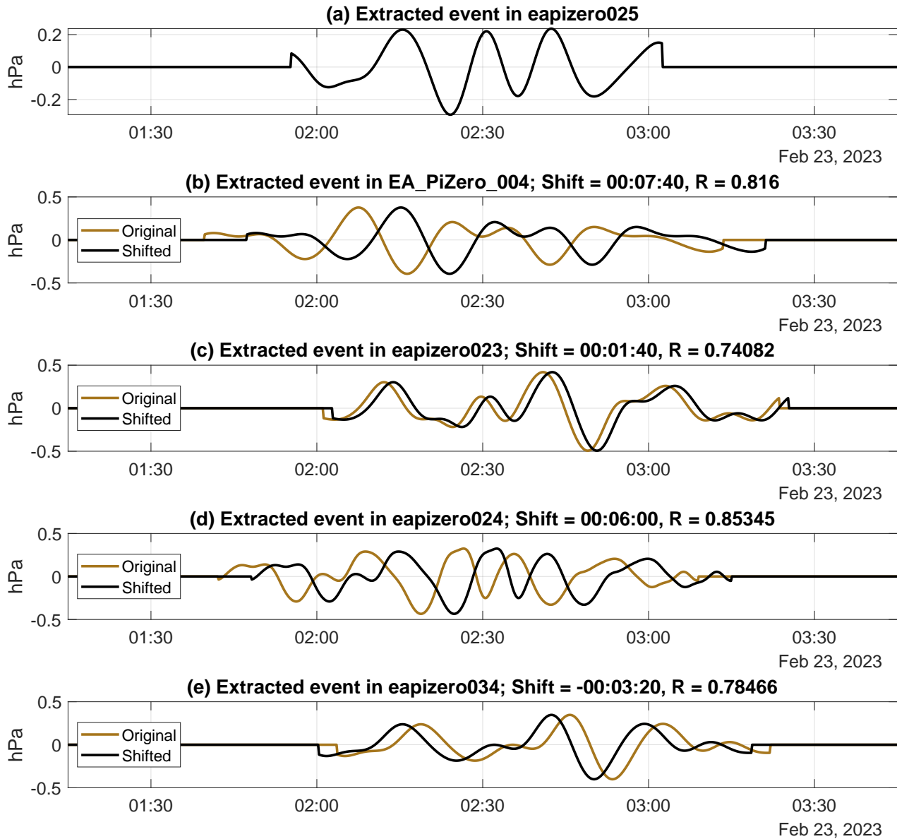
Figure 7. Extracted waveforms corresponding to the gravity wave train on 23 Feb, 2023 for sensors 25 (a), 04 (b), 23 (c), 24 (d), and 34 (e). In (b), (c), (d), and (e), brown lines show the extracted wave event with no time shift, and black lines show the extracted wave event shifted in time according to the peak cross-correlation with the extracted wave event time series for the event in sensor 25 (time shift and correlation coefficients are shown in subplot titles). All times are UTC.
