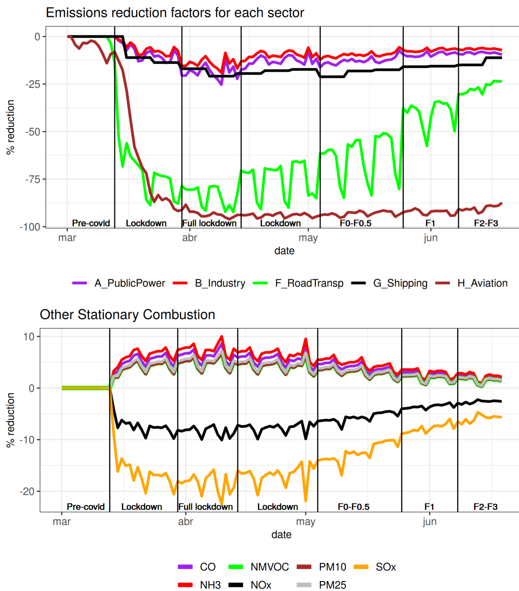
Figure 3. Emissions reduction percentage (%) for each sector. Note that the other stationary combustion sector has a different reduction level for each pollutant. The periods analysed here are written at the bottom of the figure.
