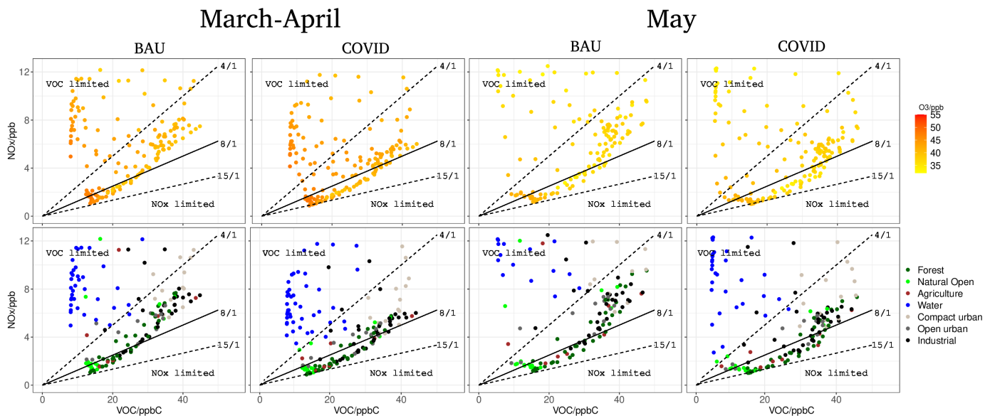
Figure 6. Same as Figure 4 during the evening (19-21 UTC).
