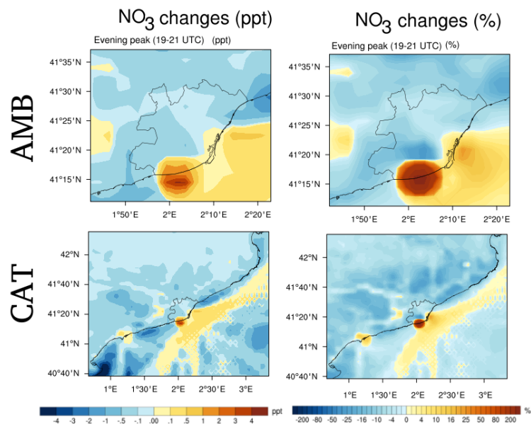
Figure 8. Evening-averaged surface NO 3 changes over the Metropolitan Area of Barcelona (AMB) and the Catalonia region ( CAT ) during 30 March to 12 April (only weekdays) and 18 to 30 May (only weekdays), with absolute values (ppt) and relative changes (%) shown. Relative changes (%) were calculated as ((\text{COVID-BAU})/\text{BAU}) \times 100 .
