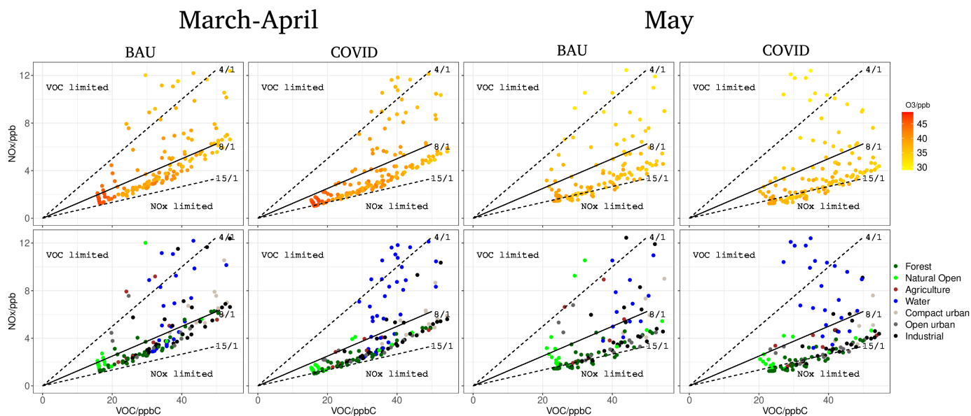
Figure 4. Change in Modelled O_3 concentrations (top panels) for 30 March to 12 April (only weekdays) and 18 to 30 May (only weekdays) for both simulations, BAU (left panels) and COVID (right panels), over the AMB area during the morning (6-8 UTC). Each dot of the top row corresponds to the O_3 concentration difference (ppb) of one grid cell of the AMB at the surface level. The dots in the lower row represent the land use for each model grid cell.
