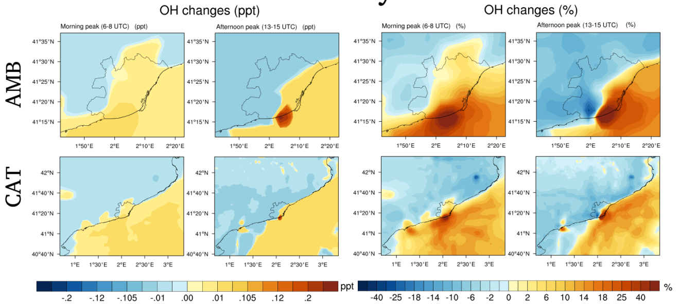
Figure 7. Morning and afternoon averaged surface OH changes over the Metropolitan Area of Barcelona (AMB) and the Catalonia region ( CAT ) during 30 March to 12 April (only weekdays) and 18 to 30 May (only weekdays), with absolute values (ppt) and relative changes (%) shown. Relative changes (%) were calculated as ((\text{COVID-BAU})/\text{BAU}) \times 100 .
