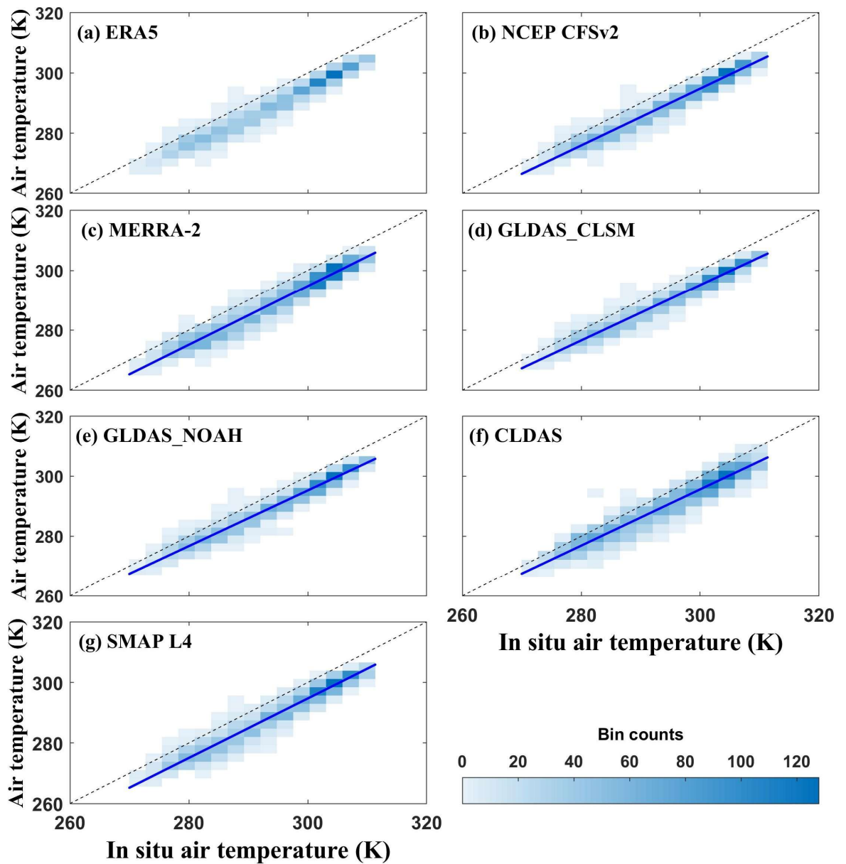
510 Fig. 9 Scatterplots of model- and observation-based air temperature averaged over all stations, from 1 April 2015 to 31 March 2020. ERA5, MERRA-2, NCEP CFSv2, GLDAS_CLSM, GLDAS_NOAH, CLDAS and CMA products provide the air temperature datasets at the 2-m screen level. SMAP L4 product provides the air temperature at center height of the lowest atmospheric model layer. Darker regions show a higher density of data point and the blue line in each subplot represents the fitted trend for the data points.
