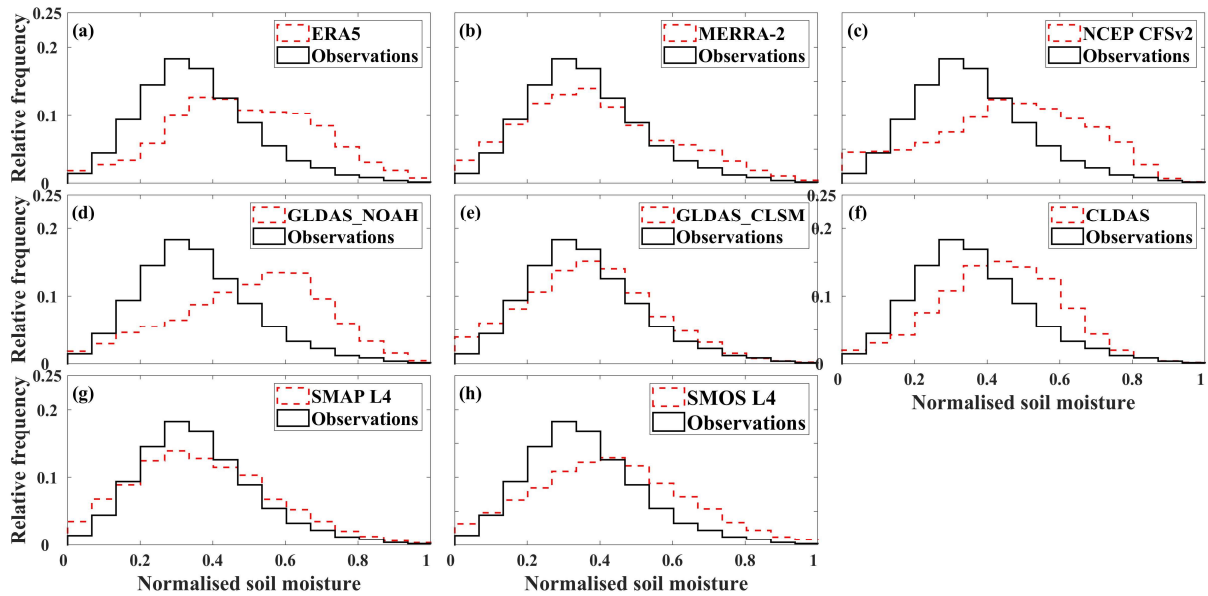
475 Fig. 6 Histograms of the relative frequency (vertical axis) of the various normalized RZSM datasets and in situ observations.
