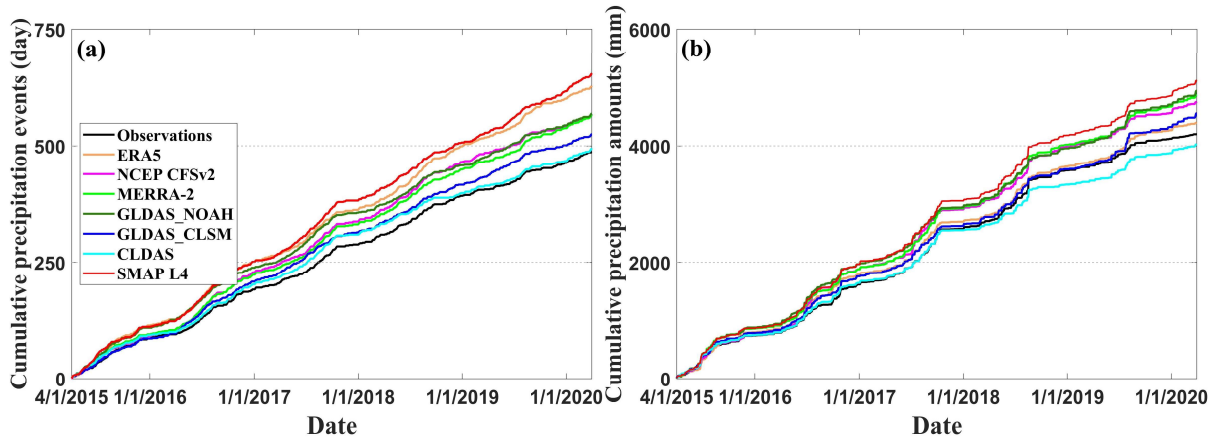
495 Fig. 7 Comparison of cumulative precipitation events and cumulative precipitation amounts between model-derived precipitation and in situ precipitation observations averaged over all in situ stations from 1 April 2015 to 31 March 2020.
