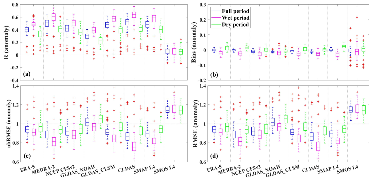
435 Fig. 4 Single-station RZSM anomalies comparison between model-derived RZSM and in situ soil moisture observations for different periods, including the Full period (from 1 April 2015 to 31 March 2020), Wet period (from June to September) and Dry period (from October to May). Each outlier “+” represents an in situ station. The five horizontal lines of the box plot represent the minimum, 25 th percentile, 50 th percentile, 75 th percentile and maximum from bottom to top, respectively.
