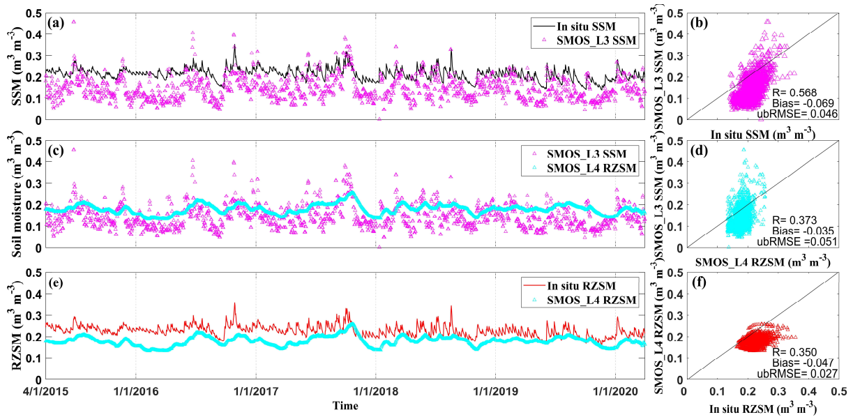
Fig. 12 Comparison of time series (left panel) and scatterplots (right panel) of SMOS L3 SSM vs. in situ SSM (Fig. 12a and b), SMOS L3 SSM vs. SMOS L4 RZSM (Fig. 12c and d) and SMOS L4 RZSM vs. in situ RZSM (Fig. 12e and f).
