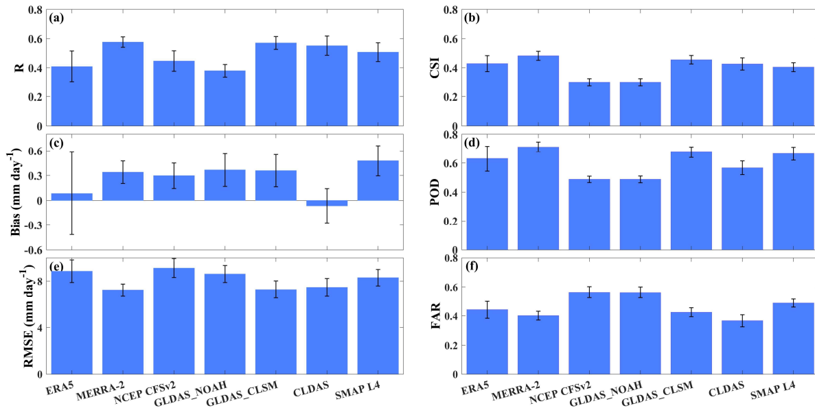
500 Fig. 8 Summary of error metrics of gridded precipitation data against in situ precipitation observations (left panel), right panel shows the detection ability of gridded precipitation to reproduce the observed precipitation. The blue histogram represents the median and black error bar represents the standard deviation.
