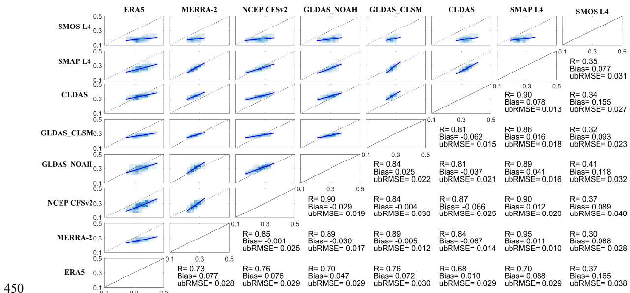
Figure 5 Comparison of different RZSM products (volumetric water content, \text{m}^3 \text{ m}^{-3} ) with each other. The scatterplots and their corresponding statistics are located on opposite sides of each other, that is, the scatterplot of the data pair SMOS L4-ERA5 is in the top left-hand corner, while the respective statistical values are found in the bottom right-hand corner. Darker regions show a higher density of data point and the blue line in each subplot represents the fitted trend for the data points.
