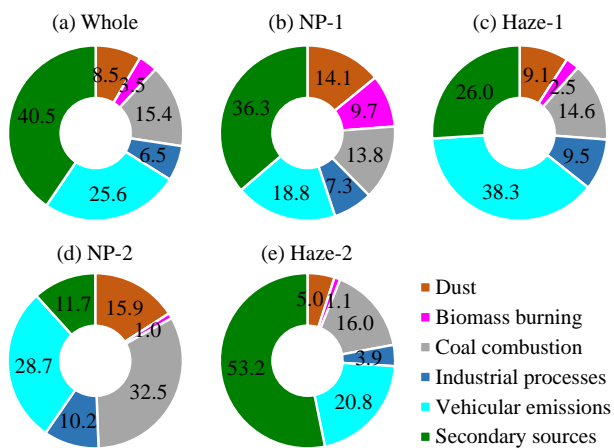
Figure 8: Composition of PM 2.5 sources in different periods (%).
