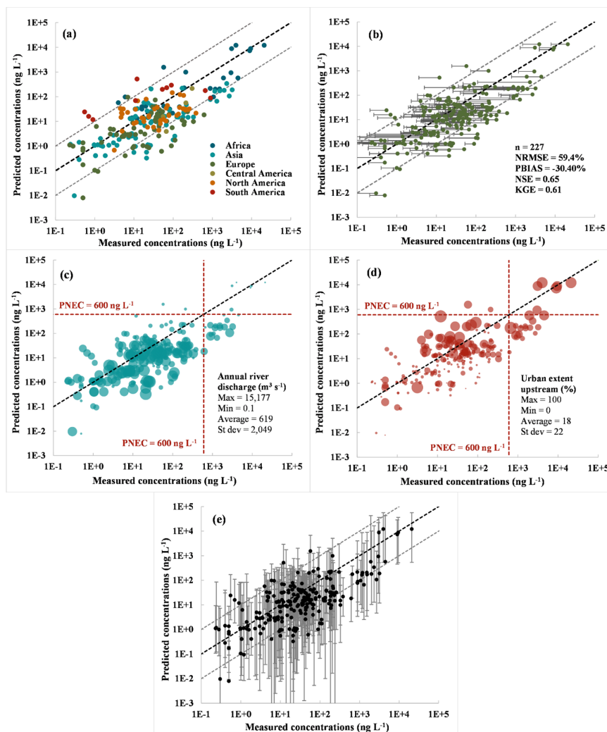
Figure 5. Evaluation of the SMX concentrations estimated using HydroFATE for baseline Scenario 1 (average-flow conditions; see Table 1 for scenario settings) individual points represent comparisons between Measured (MEC) and Predicted (PEC) Environmental Concentrations in the same river reach. The black dashed line represents the 1:1 line and the gray dashed lines represent the error line corresponding to one order of magnitude. Panel (a) shows a general scatter plot between MECs and PECs and indicates their spatial distribution (with different point colors representing the geographic regions). Panel (b) shows uncertainties of MECs regarding river discharge where the ends of the error bars represent a modified MEC assuming the original was measured during low-flow conditions; n is the number of records; NRMSE is the normalized root mean square error; PBIAS is the percent bias; NSE is the Nash-Sutcliffe efficiency; and KGE is the Kling-Gupta efficiency. Panel (c) indicates the annual river discharge at the river reach of the MEC in different bubble sizes; and panel (d) indicates the urban extent upstream of the river reach of the MEC in different bubble sizes; the red dashed lines represent the threshold for the PNEC. Panel (e) shows uncertainties of PECs where the error bars represent the range of resulting PECs using the parameter and configuration settings of Scenarios 3 and 4. Error bars that extend below 0.001 \text{ ng L}^{-1} may include predicted zero concentrations.
