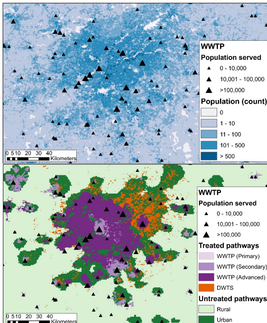
210 Figure 2. Example of the location of WWTPs and the population distribution (top panel) and the modeled contaminant pathway 215 allocation (bottom panel) for the Atlanta metropolitan area in the United States. The areas shaded in purple (bottom panel) show the estimated service areas associated with individual WWTPs (black triangles). The populations residing in these areas are connected to the river network as point sources based on the discharge locations of their respective WWTPs. The populations residing in the orange areas (bottom panel) are identified as being associated with decentralized wastewater systems and are connected to the river network as diffuse but treated sources within the catchment of each river reach. The populations residing in the areas represented by shades of green (bottom panel) are associated with untreated wastewater contributions and are connected to the river network as diffuse sources within the catchment of each river reach.
