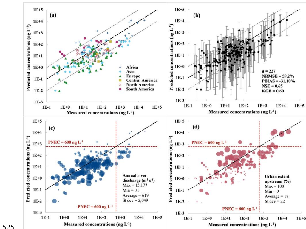
525 Figure 5. Evaluation of the SMX concentrations estimated using HydroFATE for baseline Scenario 1 (average-flow conditions; see Table 1 for scenario settings). Individual points represent comparisons between Measured (MEC) and Predicted (PEC) Environmental Concentrations in the same river reach. The black dashed line represents the 1:1 line and the gray dashed lines represent the error line corresponding to one order of magnitude. Panel (a) shows a general scatter plot between MECs and PECs and indicates their spatial distribution (with different symbols and colors representing the geographic regions). Panel (b) shows uncertainties of PECs where the error bars represent the range of resulting PECs using the parameter and configuration settings of Scenarios 3 and 4; n is the number of records; NRMSE is the normalized root mean square error; PBIAS is the percent bias; NSE is the Nash-Sutcliffe efficiency; and KGE is the Kling-Gupta efficiency. Panel (c) indicates the annual river discharge at the river reach of the MEC in different bubble sizes; and panel (d) indicates the urban extent upstream of the river reach of the MEC in different bubble sizes; the red dashed lines represent the threshold for the PNEC. Error bars that extend below 0.001 ng L -1 may include predicted zero concentrations.
