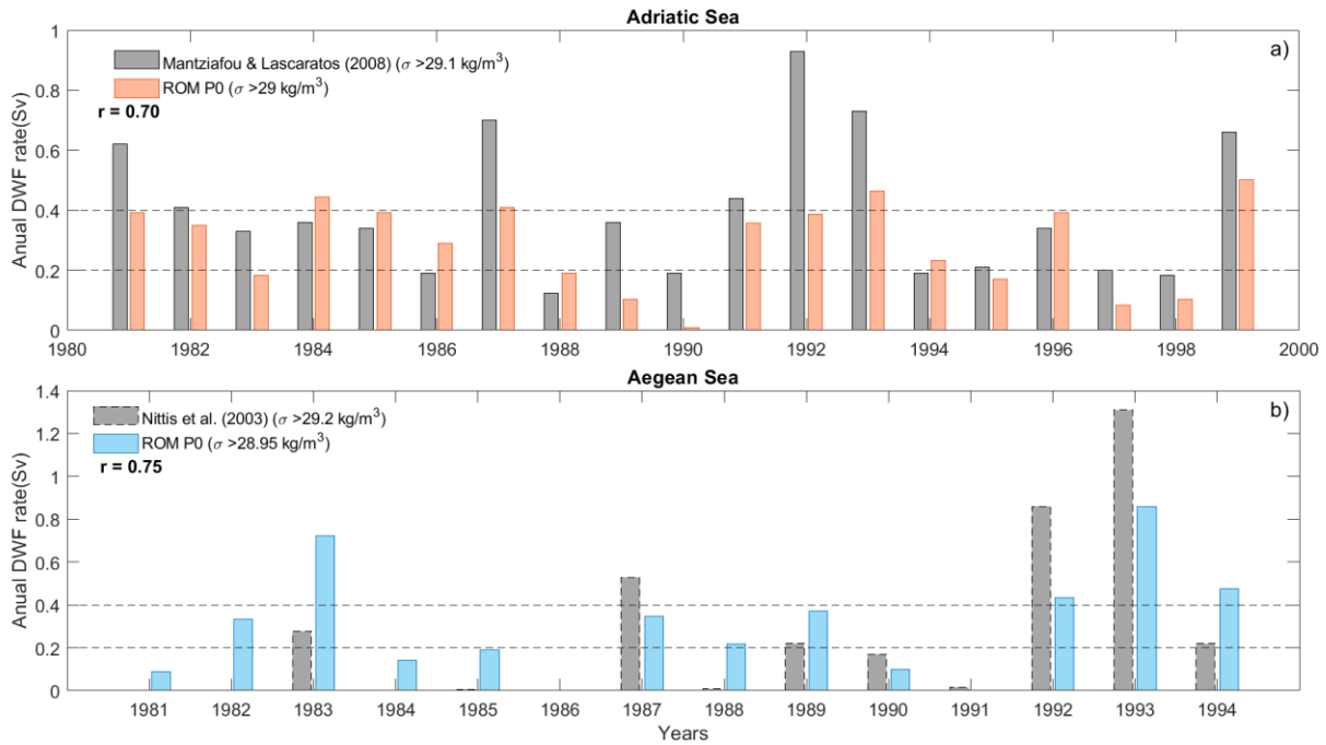
480 Figure 2. Annual formation rate (Sv) of deep water in the (a) Adriatic Sea and (b) Aegean Sea. Note different ranges in vertical and horizontal axes.
