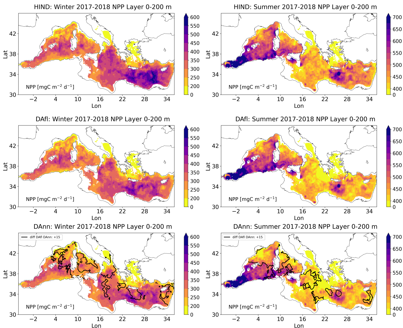
Figure 11. Maps of winter (FMA) and summer (JJA) net primary production [NPP, mgC m -2 d -1 ] in the three simulations: HIND (first row); DAfl (second row). DAnn (third row). Seasonal averages were calculated for the period 2017-2018. The black contour lines in the third row encompass areas where the NPP difference between DAnn and DAfl exceeds 15 mgC m -2 d -1
