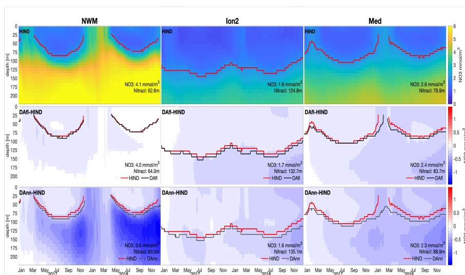
Figure 7. Hovmöller diagram of nitrate of HIND simulation (first row) and differences between assimilation runs and HIND (second and third rows) for 2 sub-basins (nwm and ion2) and the Mediterranean Sea (med). Evolution of the depth of nitracline (the depth at which nitrate concentration is 2 \text{ mmol m}^{-3} ) for the three runs: red (HIND) and black (DAfl and DAnn) lines. The averages of 0-200m concentration and of nitracline for the simulated period are reported.
