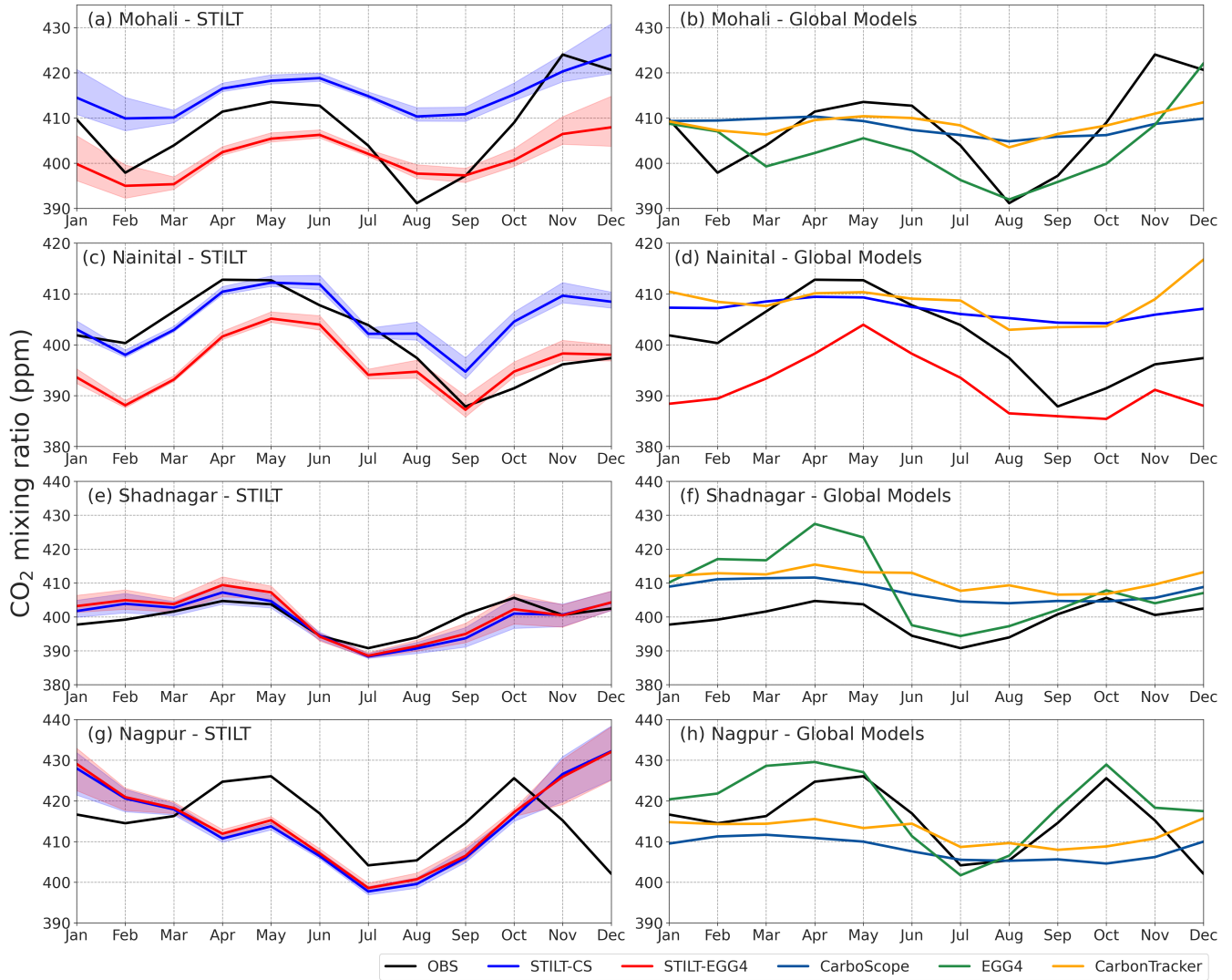
Figure 3. CO 2 seasonal cycle for different stations. Monthly mean values of CO 2 observations in comparison with STILT simulations (left panel) and global models (right panel) are given. Blue (STILT-CS) and red (STILT-EGG4) curves represent the ensemble average of the STILT simulations using different anthropogenic fluxes. Shaded regions represent the range of the model simulations.
