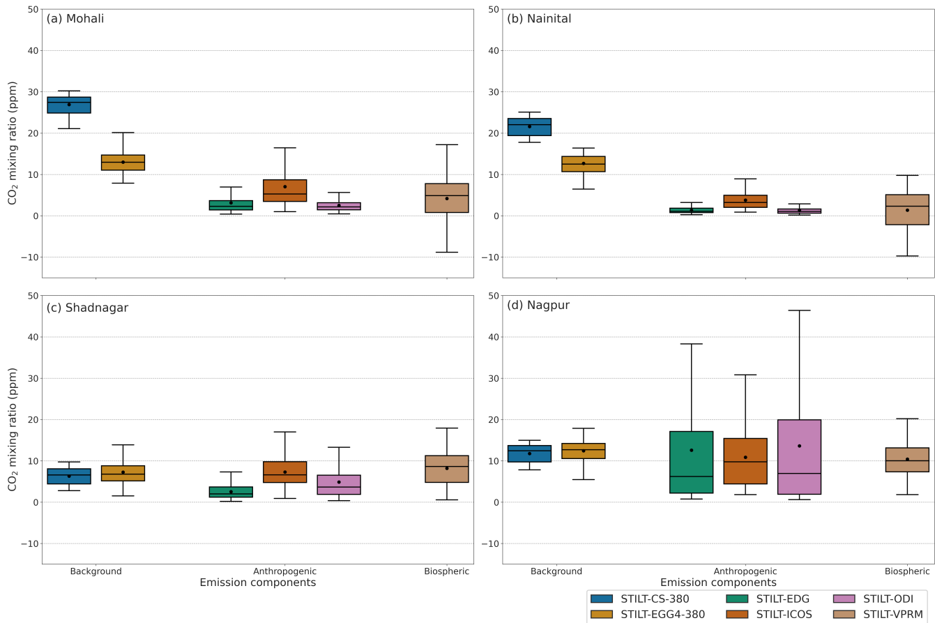
Figure 5. Variability in STILT CO 2 emission components at different stations. For better comparison with other emission components, 380 ppm is reduced from background components. The panels represent the variability in (a) Mohali daytime (11:00-16:00 local time) simulations, (b) Nainital, (c) Shadnagar and (d) Nagpur simulations.
