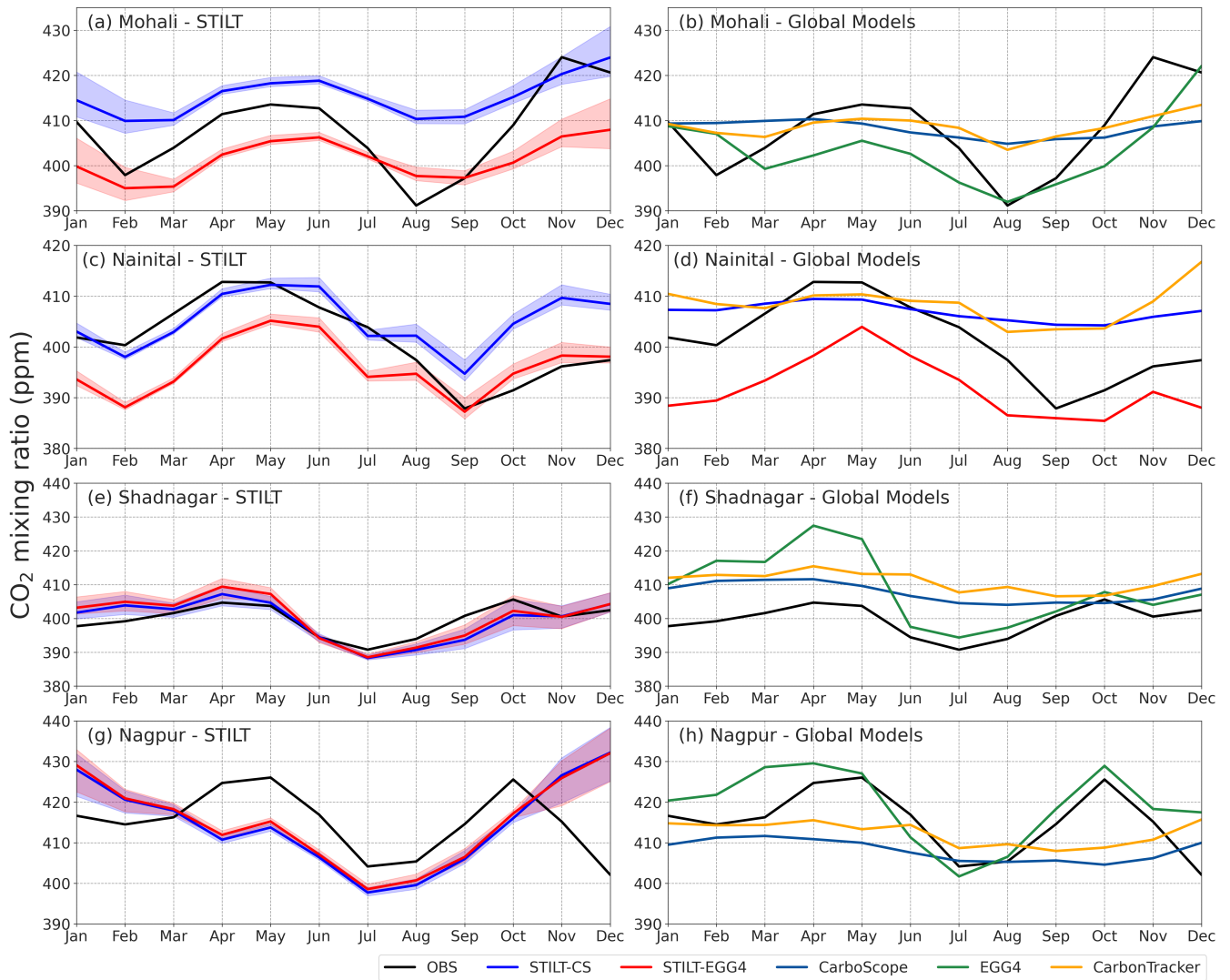
Figure 3. CO 2 time-series seasonal cycle for different stations. Monthly mean values of weekly-CO 2 observations in comparison with STILT simulations (14:00 local time left panel) at NTL with and global models (right panel) STILT simulations are given. Blue (STILT-CS) and red (STILT-EGG4) curves represent the ensemble average of the STILT simulations using different anthropogenic fluxes. Shaded regions represent the range of the model simulations. (b) Global reanalysis products:
