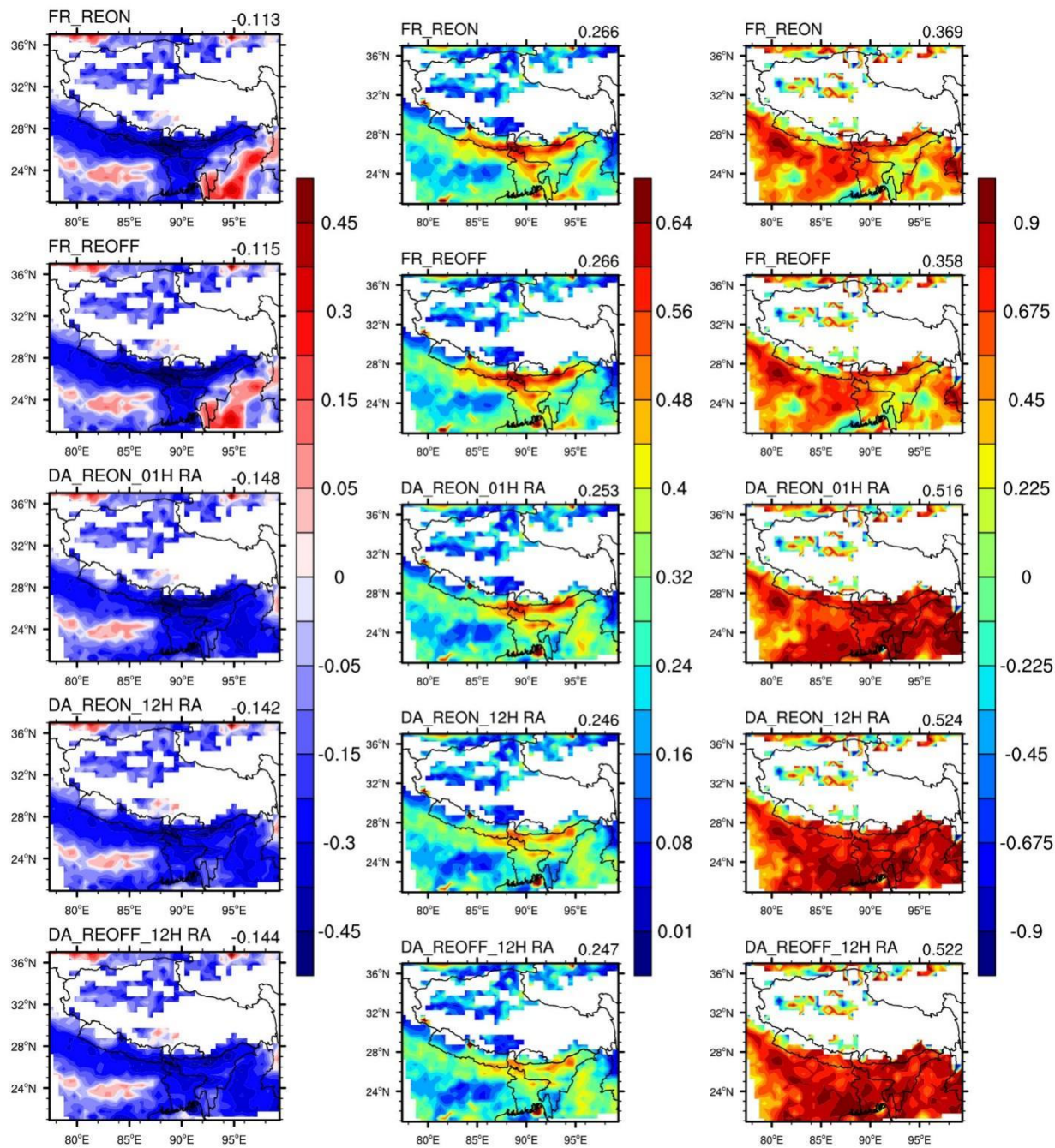
830 Figure 4: Spatial distributions of the BIASES (the left column), RMSEs (the center column), CORRs (the right column) between the simulated or analysis field and MODIS AOTs at 550 nm during 10-24 March 2018 for the FR_REON, FR_REOFF, DA_REON_01H, DA_REON_12H, DA_REOFF_12H experiments.
